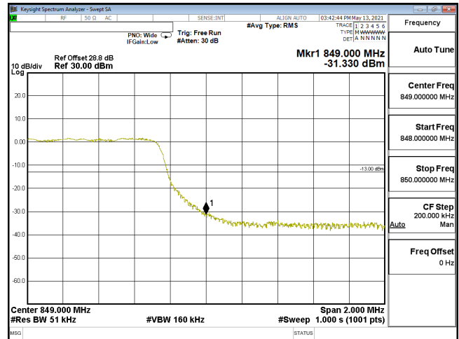
EDGE-ENDC_30A_n5-256QAM_5M_CH169300_846.5(25,0)_SCS15KHz
