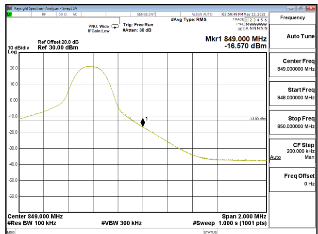
EDGE-ENDC_30A_n5-QPSK_10M_CH168800_844(1,51)_SCS15KHz
