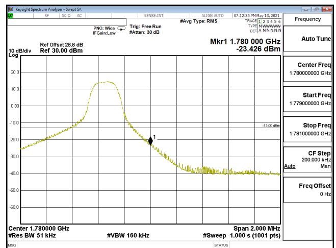
EDGE-ENDC 12A_n66-256QAM 5M_CH355500_1777.5(1,24)_SCS15KHz
