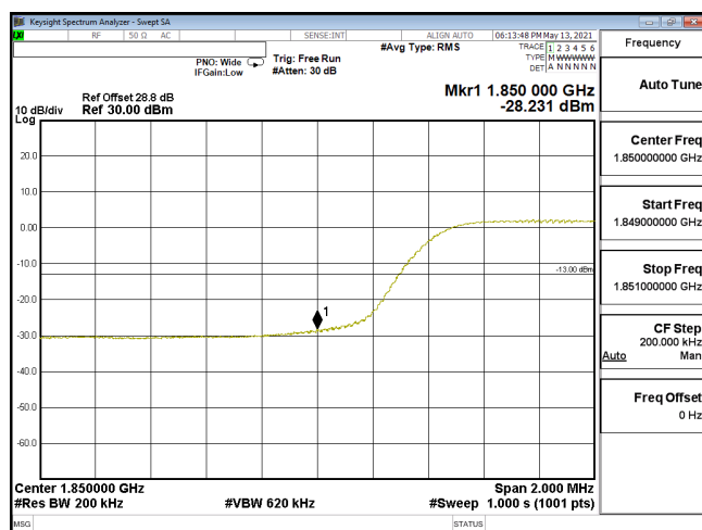
EDGE-ENDC_5A_n2-16QAM_20M_CH372000_1860(100,0)_SCS15KHz
