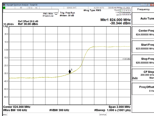
EDGE-ENDC_30A_n5-QPSK_10M_CH165800_829(50,0)_SCS15KHz
