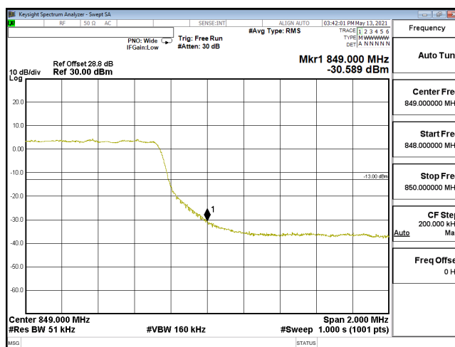
EDGE-ENDC_30A_n5-16QAM_5M_CH169300_846.5(25,0)_SCS15KHz
