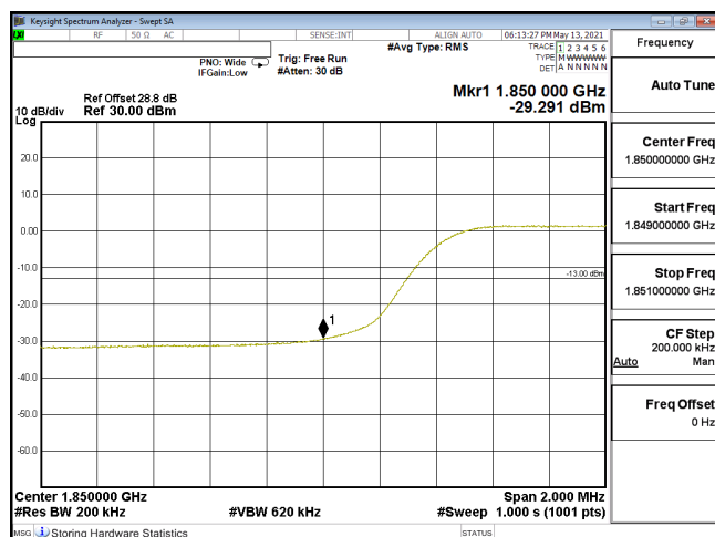
EDGE-ENDC_5A_n2-64QAM_20M_CH372000_1860(100,0)_SCS15KHz
