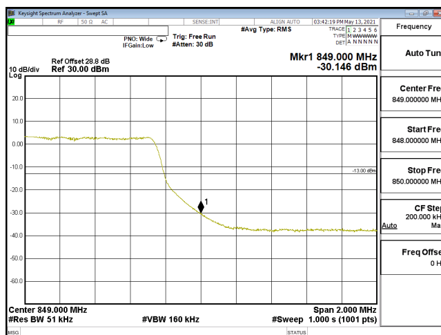
EDGE-ENDC_30A_n5-64QAM_5M_CH169300_846.5(25,0)_SCS15KHz
