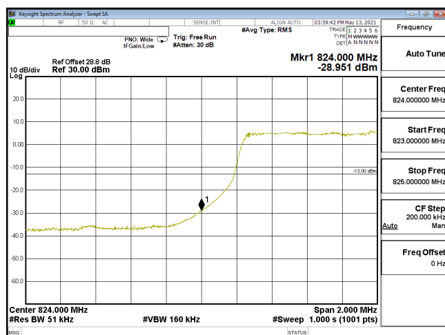
EDGE-ENDC_30A_n5-QPSK_5M_CH165300_826.5(25,0)_SCS15KHz
