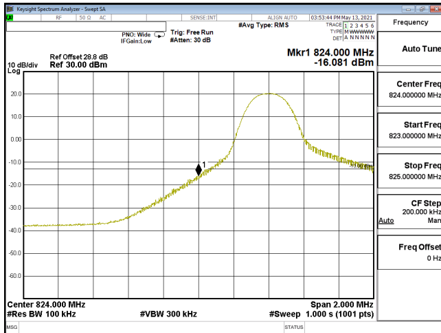
EDGE-ENDC_30A_n5-16QAM_10M_CH165800_829(1,0)_SCS15KHz
