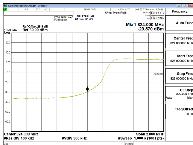
EDGE-ENDC_30A_n5-16QAM_10M_CH165800_829(50,0)_SCS15KHz
