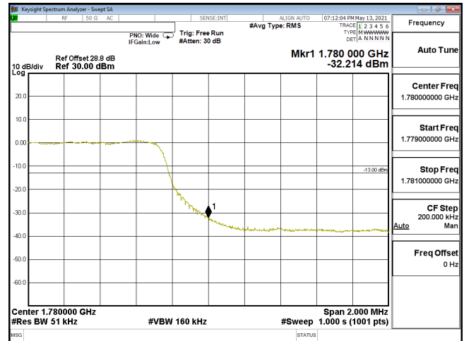
EDGE-ENDC_12A_n66-256QAM_5M_CH355500_1777.5(25,0)_SCS15KHz
