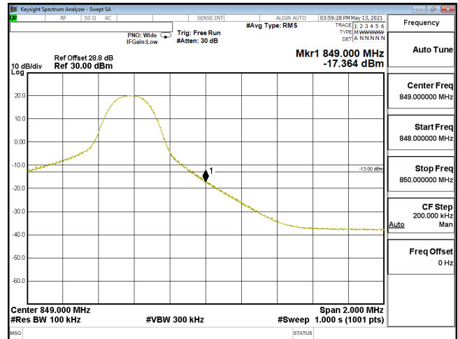
EDGE-ENDC_30A_n5-16QAM_10M_CH168800_844(1,51)_SCS15KHz
