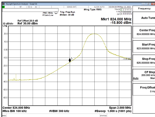
EDGE-ENDC_30A_n5-64QAM_10M_CH165800_829(1,0)_SCS15KHz
