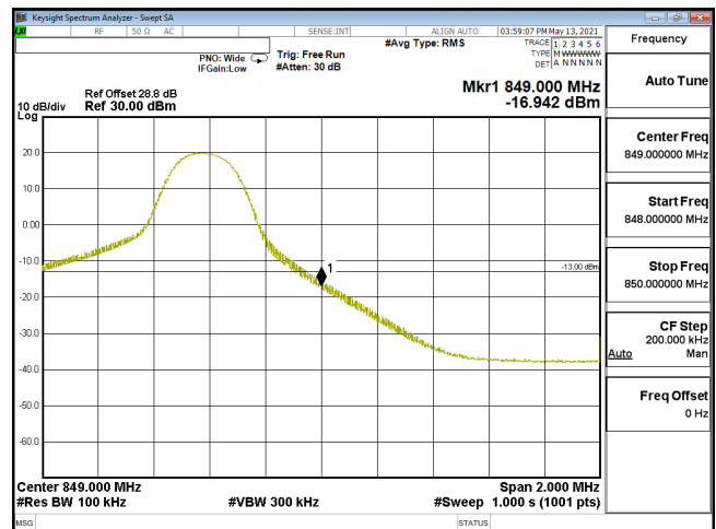
EDGE-ENDC_30A_n5-64QAM_10M_CH168800_844(1,51)_SCS15KHz
