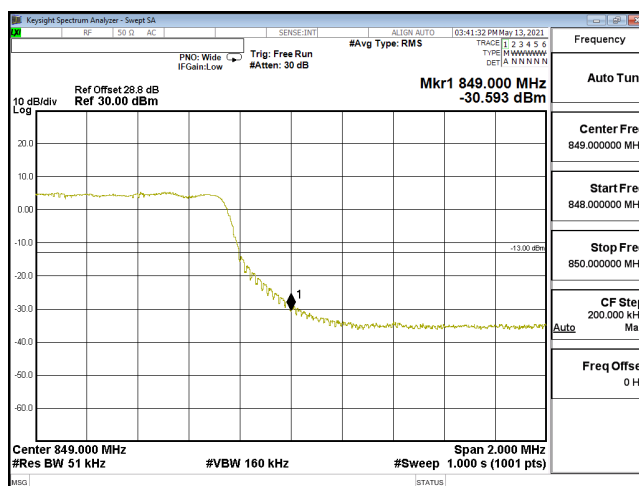
EDGE-ENDC_30A_n5-QPSK_5M_CH169300_846.5(25,0)_SCS15KHz
