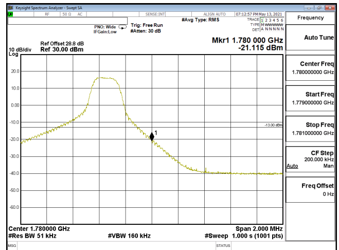
EDGE-ENDC_12A_n66-64QAM_5M_CH355500_1777.5(1,24)_SCS15KHz
