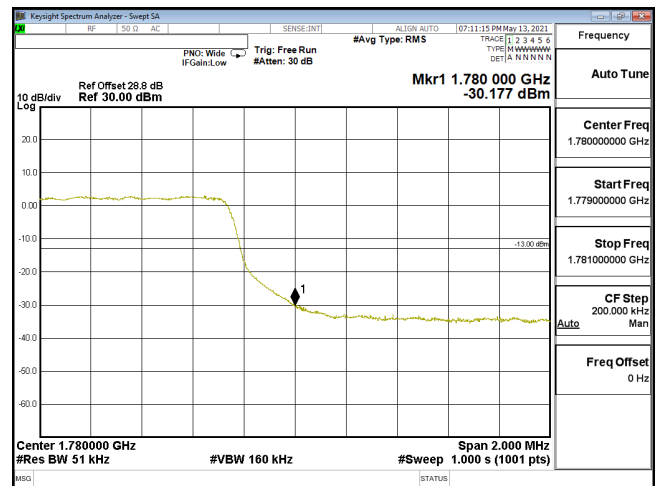
EDGE-ENDC_12A_n66-16QAM_5M_CH355500_1777.5(25,0)_SCS15KHz
