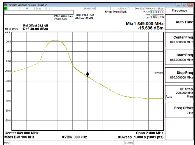
EDGE-ENDC_30A_n5-PI2-BPSK_10M_CH168800_844(1,51)_SCS15KHz
