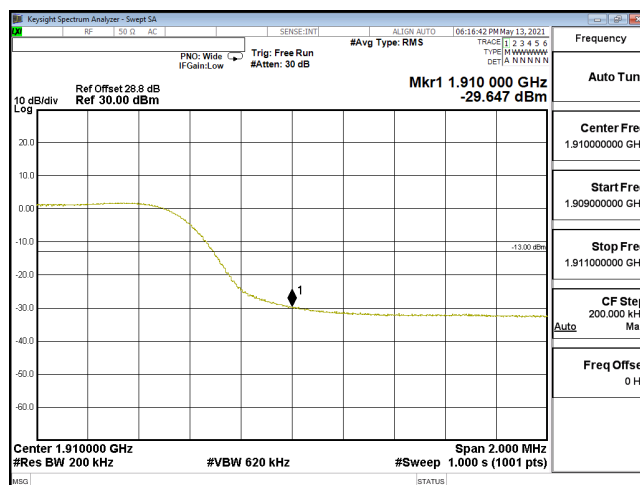
EDGE-ENDC_5A_n2-64QAM_20M_CH380000_1900(100,6)_SCS15KHz
