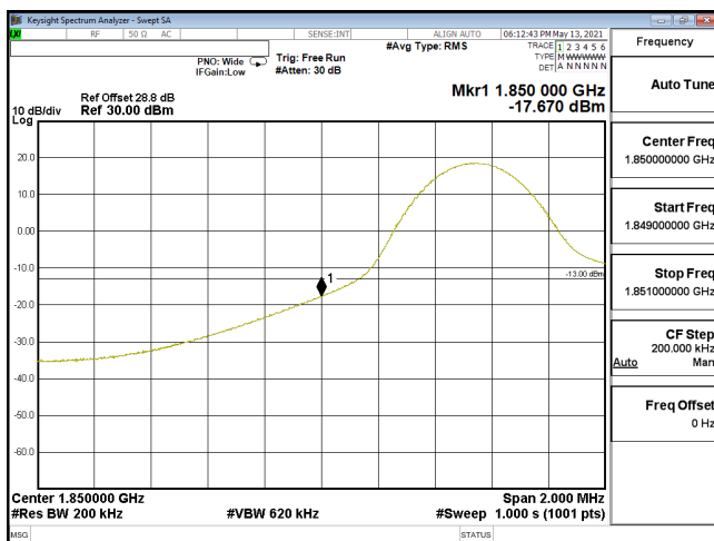
EDGE-ENDC_5A_n2-256QAM_20M_CH372000_1860(1,0)_SCS15KHz
