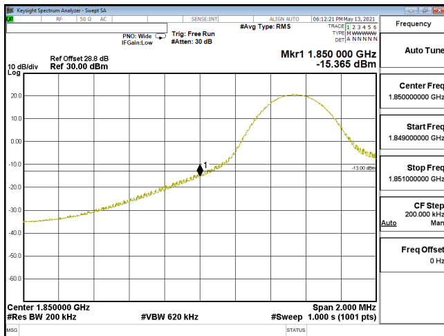
EDGE-ENDC_5A_n2-64QAM_20M_CH372000_1860(1,0)_SCS15KHz
