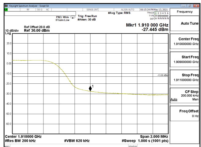
EDGE-ENDC_5A_n2-PI2-BPSK_20M_CH380000_1900(100,6)_SCS15KHz
