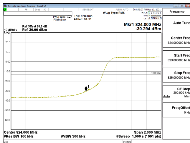
EDGE-ENDC_30A_n5-PI2-BPSK_10M_CH165800_829(50,0)_SCS15KHz
