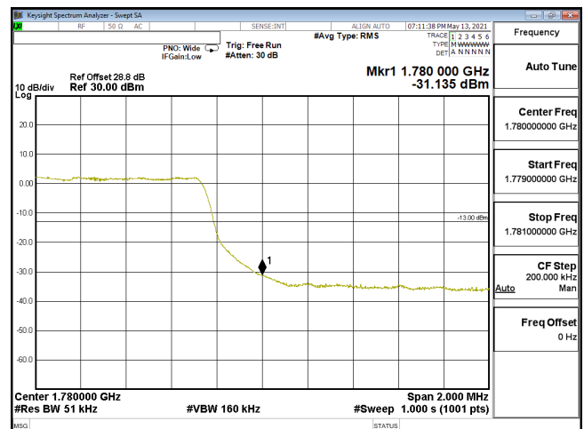
EDGE-ENDC_12A_n66-64QAM_5M_CH355500_1777.5(25,0)_SCS15KHz
