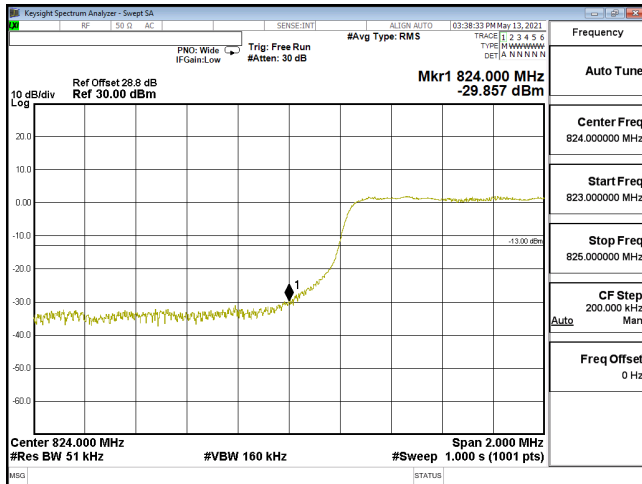
EDGE-ENDC_30A_n5-256QAM_5M_CH165300_826.5(25,0)_SCS15KHz
