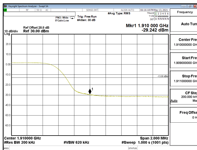
EDGE-ENDC_5A_n2-16QAM_20M_CH380000_1900(100,6)_SCS15KHz
