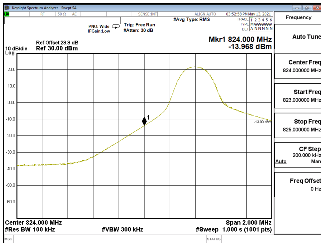
EDGE-ENDC_30A_n5-PI2-BPSK_10M_CH165800_829(1,0)_SCS15KHz
