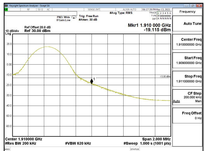
EDGE-ENDC_5A_n2-256QAM_20M_CH380000_1900(1,105)_SCS15KHz
