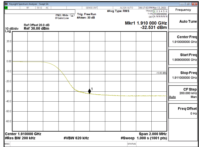
EDGE-ENDC_5A_n2-256QAM_20M_CH380000_1900(100,6)_SCS15KHz
