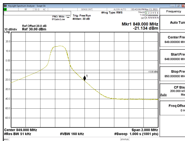
EDGE-ENDC 30A n5-256QAM 5M CH169300 846.5(1,24) SCS15KHz
