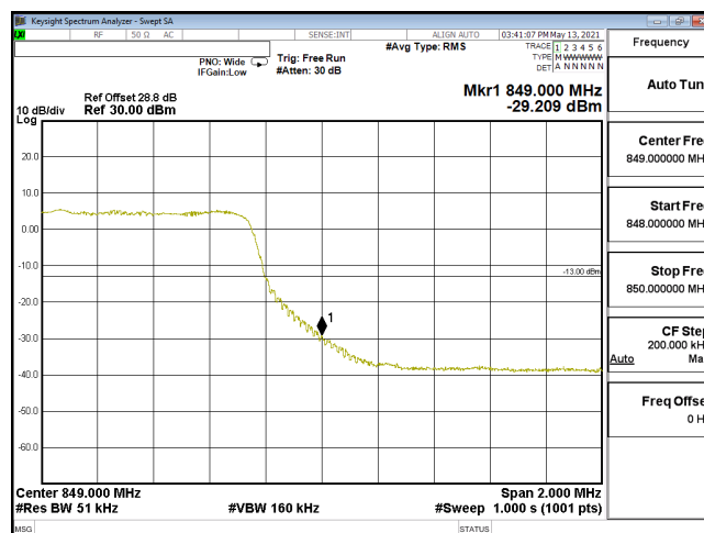
EDGE-ENDC 30A n5-PI2-BPSK 5M CH169300 846.5(25,0) SCS15KHz
