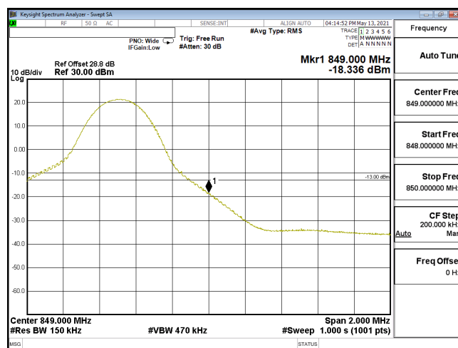
EDGE-ENDC 30A n5-16QAM 15M CH168300 841.5(1,78) SCS15KHz
