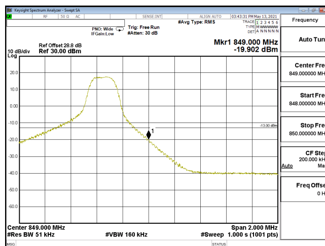
EDGE-ENDC 30A n5-64QAM 5M CH169300 846.5(1,24) SCS15KHz
