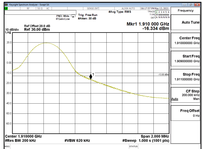
EDGE-ENDC_5A_n2-64QAM_20M_CH380000_1900(1,105)_SCS15KHz
