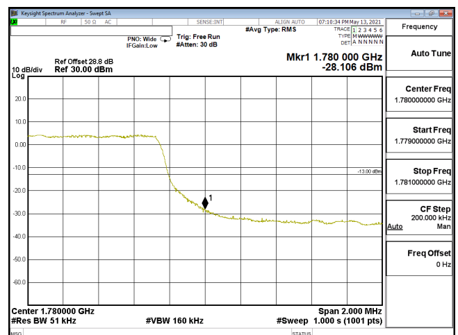
EDGE-ENDC 12A n66-PI2-BPSK 5M CH355500 1777.5(25,0) SCS15KHz
