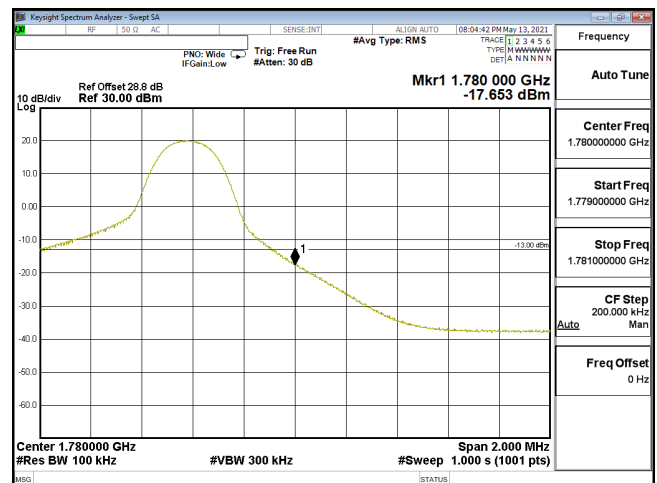
EDGE-ENDC_12A_n66-QPSK_10M_CH355000_1715(1,51)_SCS15KHz
