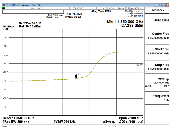
EDGE-ENDC_5A_n2-PI2-BPSK_20M_CH372000_1860(100,0)_SCS15KHz
