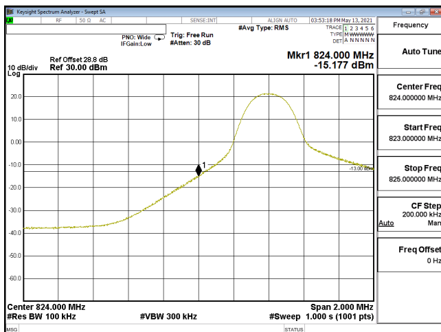
EDGE-ENDC_30A_n5-QPSK_10M_CH165800_829(1,0)_SCS15KHz
