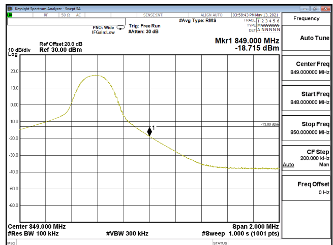
EDGE-ENDC_30A_n5-256QAM_10M_CH168800_844(1,51)_SCS15KHz
