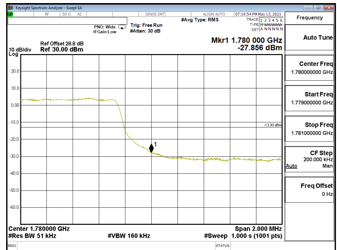
EDGE-ENDC_12A_n66-QPSK_5M_CH355500_1777.5(25,0)_SCS15KHz
