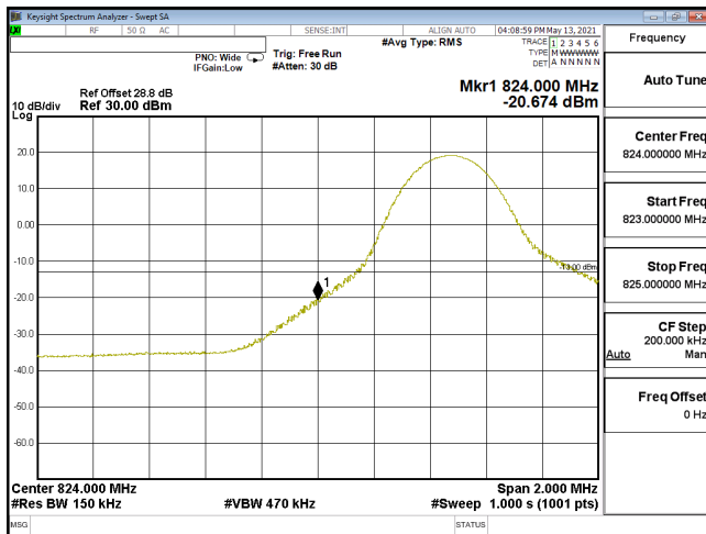
EDGE-ENDC_30A_n5-256QAM_15M_CH166300_831.5(1,0)_SCS15KHz
