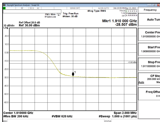
EDGE-ENDC_5A_n2-QPSK_20M_CH380000_1900(100,6)_SCS15KHz
