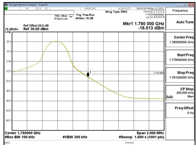
EDGE-ENDC_12A_n66-PI2-BPSK_10M_CH355000_1715(1,51)_SCS15KHz
