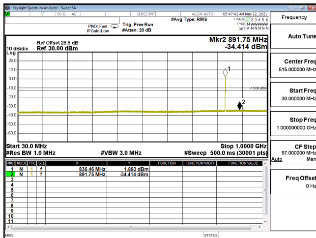
CSE-ENDC_5A_n2_QPSK_5M_CH370500_1852.5(1,12)-30M-1G
