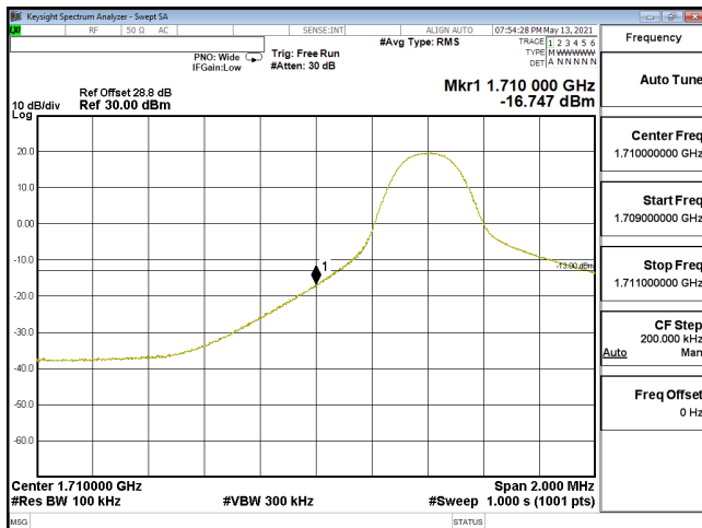
EDGE-ENDC_12A_n66-16QAM_10M_CH343000_1715(1,0)_SCS15KHz
