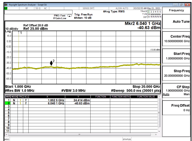
CSE-ENDC_5A_n2_QPSK_5M_CH370500_1852.5(1,12)-1G-20G
