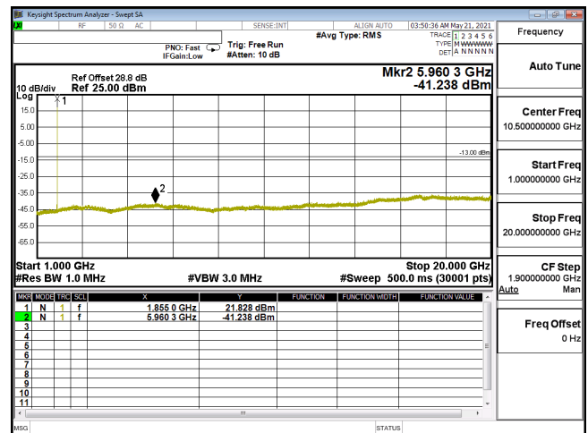
CSE-ENDC_5A_n2_256QAM_10M_CH371000_1855(1,26)-1G-20G
