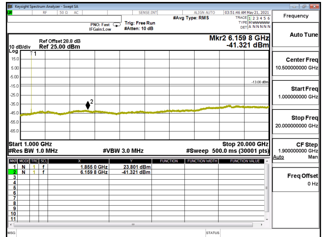
CSE-ENDC_5A_n2_P12-BPSK_10M_CH371000_1855(1,26)-1G-20G
