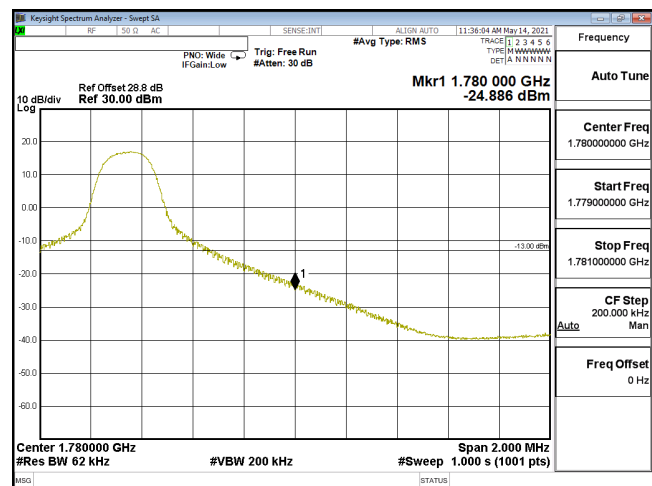
EDGE-ENDC_12A_n66-64QAM_40M_CH352000_1760(1,215)_SCS15KHz
