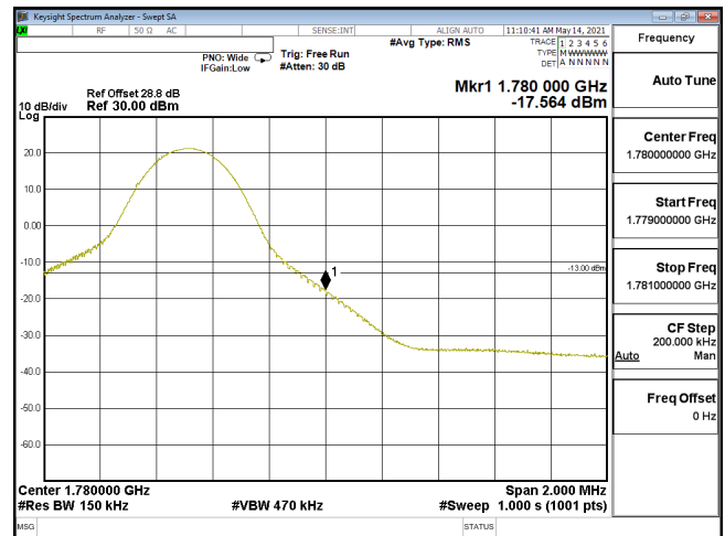
EDGE-ENDC_12A_n66-QPSK_15M_CH354500_1717.5(1,78)_SCS15KHz
