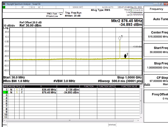
CSE-ENDC_5A_n2_PI2-BPSK_5M_CH370500_1852.5(1,12)-30M-1G
