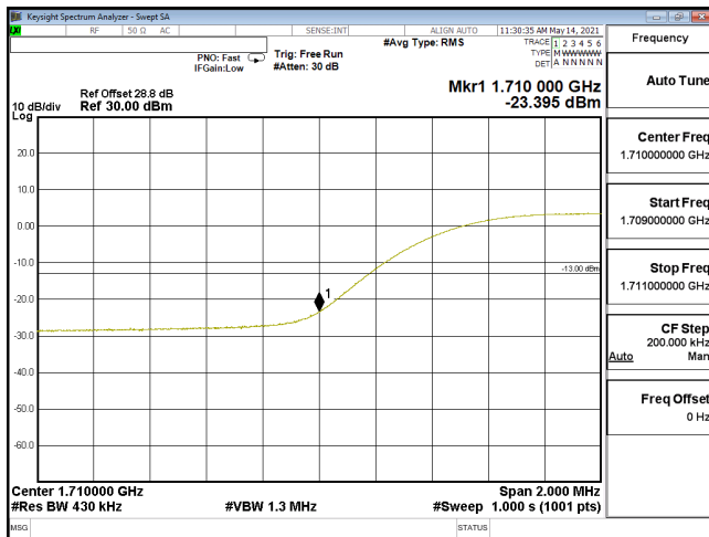
EDGE-ENDC_12A_n66-PI2-BPSK_40M_CH346000_1730(216,0)_SCS15KHz
