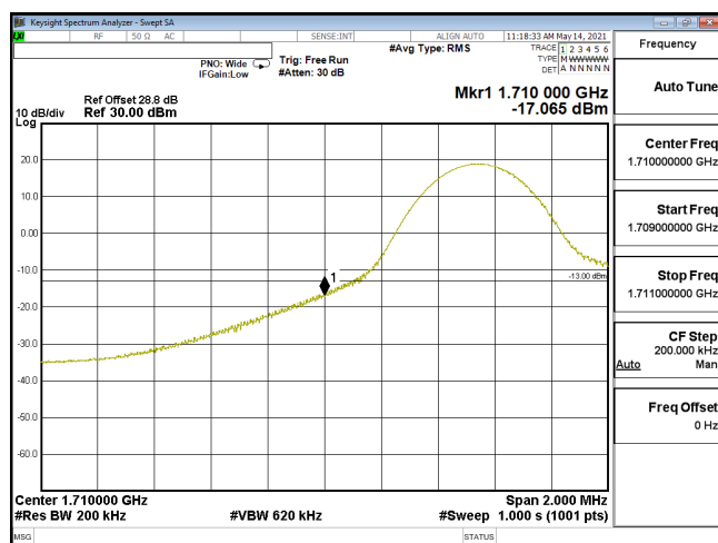
EDGE-ENDC_12A_n66-256QAM_20M_CH344000_1720(1,0)_SCS15KHz
