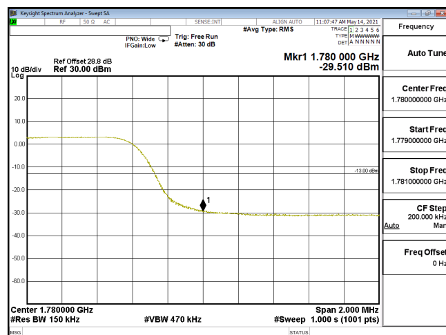
EDGE-ENDC_12A_n66-QPSK_15M_CH354500_1717.5(75,4)_SCS15KHz
