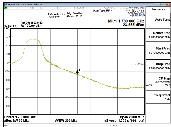
EDGE-ENDC_12A_n66-16QAM_40M_CH352000_1760(1,215)_SCS15KHz
