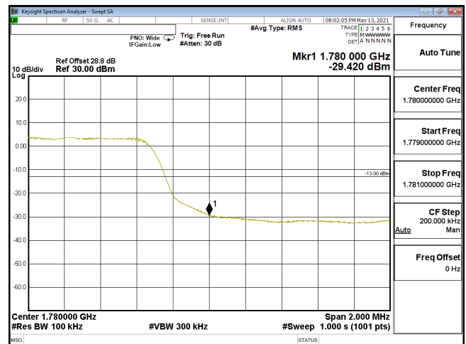
EDGE-ENDC_12A_n66-QPSK_10M_CH355000_1715(50,2)_SCS15KHz
