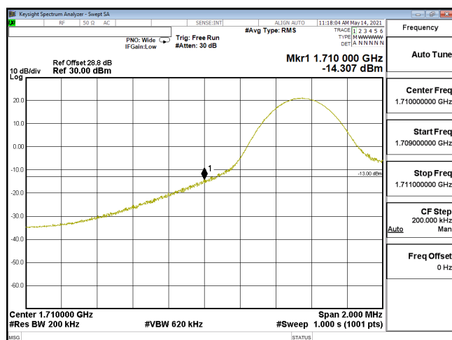
EDGE-ENDC_12A_n66-64QAM_20M_CH344000_1720(1,0)_SCS15KHz
