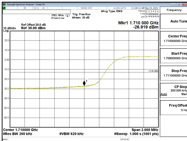
EDGE-ENDC_12A_n66-QPSK_20M_CH344000_1720(100,0)_SCS15KHz
