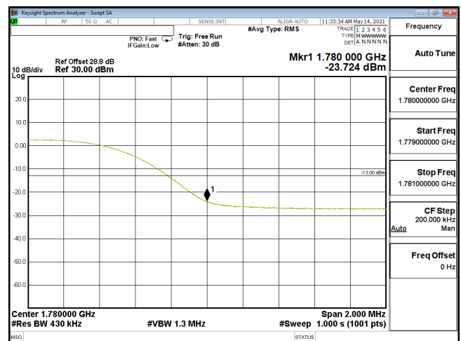
EDGE-ENDC_12A_n66-QPSK_40M_CH352000_1760(216,0)_SCS15KHz
