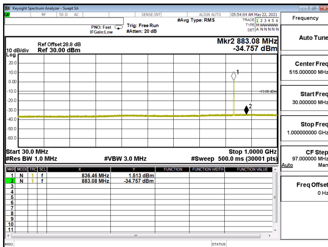
CSE-ENDC_5A_n2_256QAM_10M_CH371000_1855(1,26)-30M-1G
