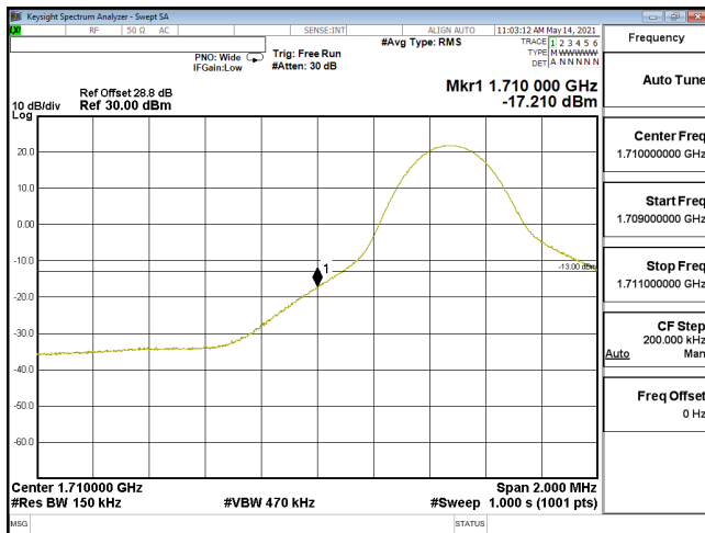
EDGE-ENDC_12A_n66-QPSK_15M_CH343500_1717.5(1,0)_SCS15KHz
