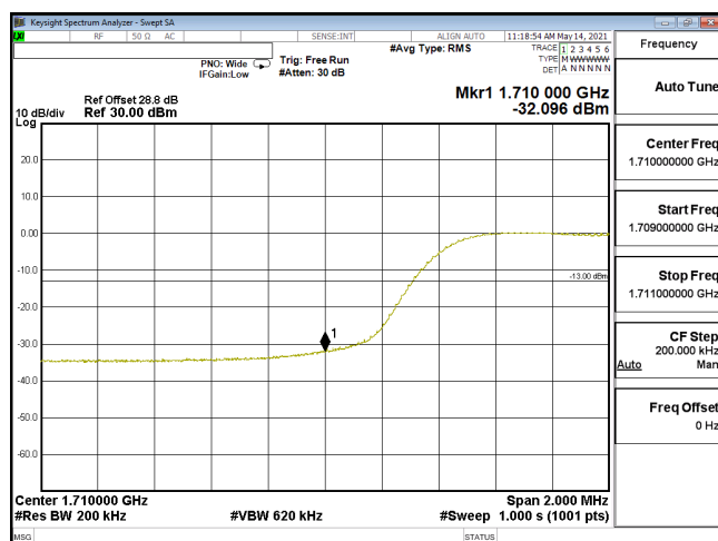
EDGE-ENDC_12A_n66-256QAM_20M_CH344000_1720(100,0)_SCS15KHz
