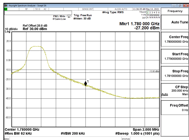
EDGE-ENDC_12A_n66-256QAM_40M_CH352000_1760(1,215)_SCS15KHz
