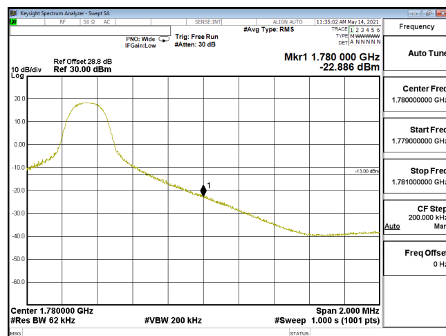
EDGE-ENDC_12A_n66-QPSK_40M_CH352000_1760(1,215)_SCS15KHz
