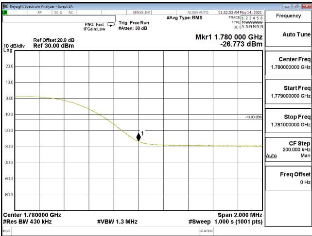
EDGE-ENDC_12A_n66-64QAM_40M_CH352000_1760(216,0)_SCS15KHz
