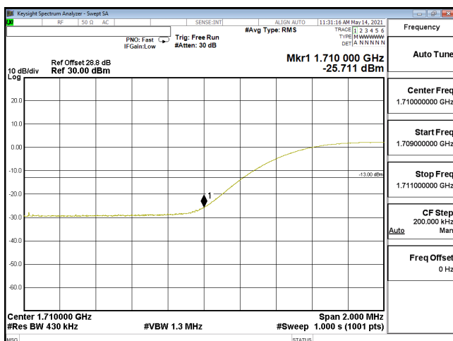
EDGE-ENDC_12A_n66-16QAM_40M_CH346000_1730(216,0)_SCS15KHz
