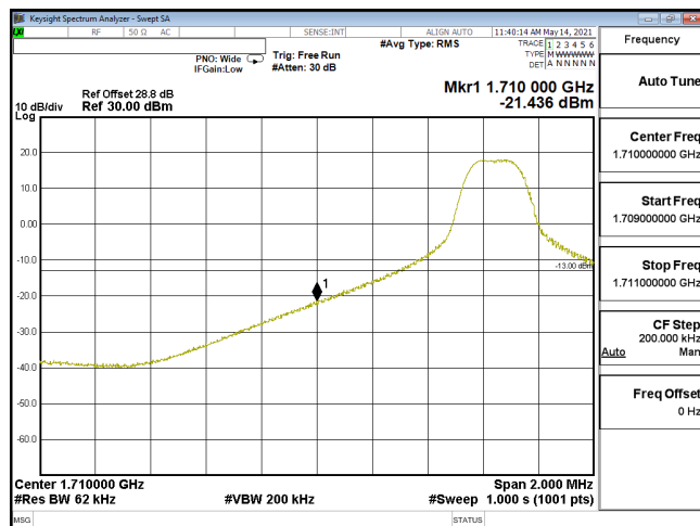
EDGE-ENDC_12A_n66-16QAM_40M_CH346000_1730(1,0)_SCS15KHz
