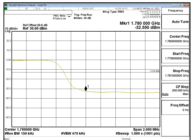
EDGE-ENDC_12A_n66-256QAM_15M_CH354500_1717.5(75,4)_SCS15KHz
