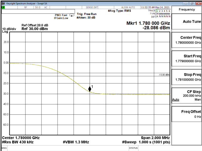
EDGE-ENDC_12A_n66-256QAM_40M_CH352000_1760(216,0)_SCS15KHz
