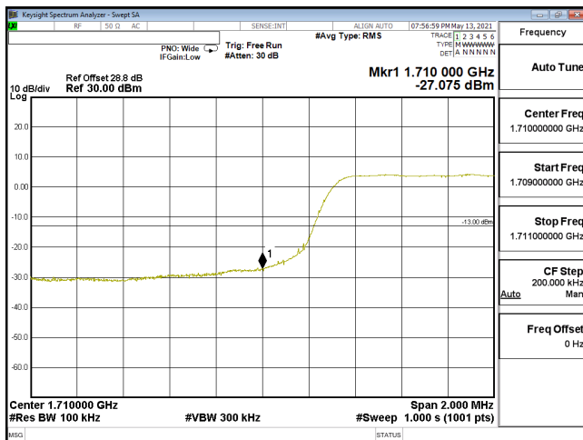
EDGE-ENDC_12A_n66-QPSK_10M_CH343000_1715(50,0)_SCS15KHz
