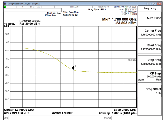
EDGE-ENDC_12A_n66-PI2-BPSK_40M_CH352000_1760(216,0)_SCS15KHz
