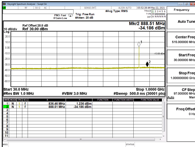
CSE-ENDC_5A_n2_P12-BPSK_10M_CH371000_1855(1,26)-30M-1G
