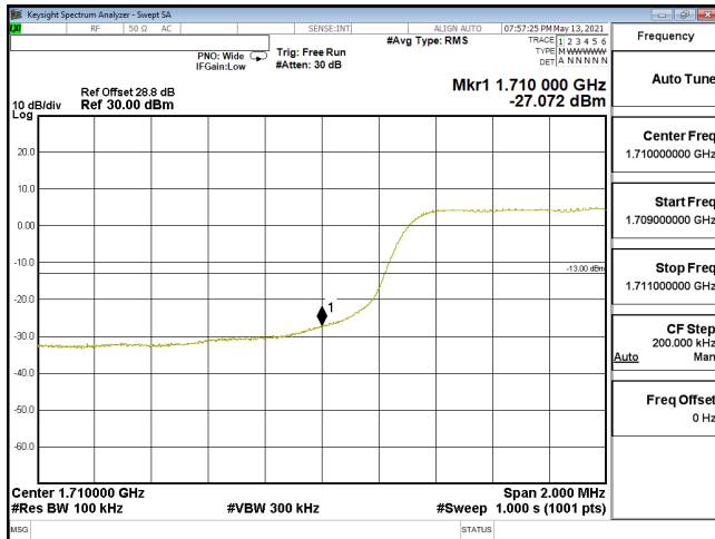
EDGE-ENDC_12A_n66-PI2-BPSK_10M_CH343000_1715(50,0)_SCS15KHz
