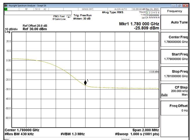
EDGE-ENDC_12A_n66-16QAM_40M_CH352000_1760(216,0)_SCS15KHz
