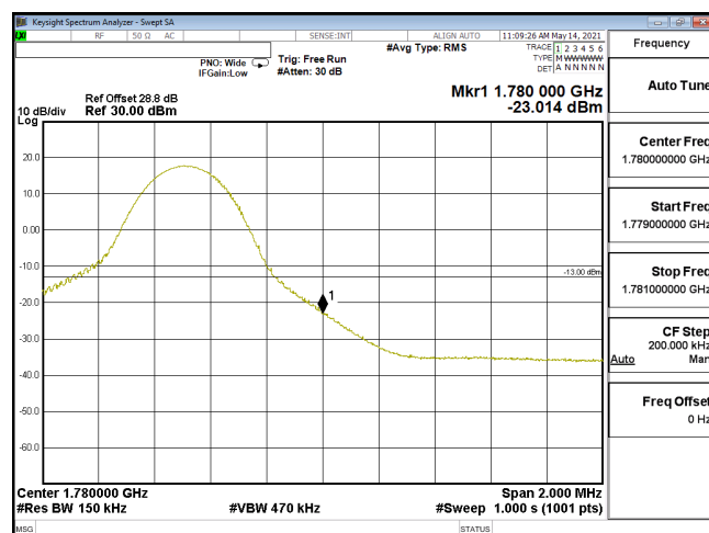
EDGE-ENDC_12A_n66-256QAM_15M_CH354500_1717.5(1,78)_SCS15KHz
