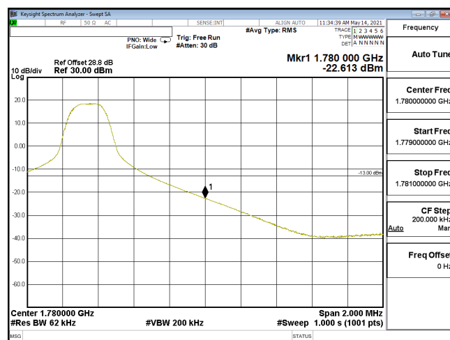
EDGE-ENDC_12A_n66-PI2-BPSK_40M_CH352000_1760(1,215)_SCS15KHz
