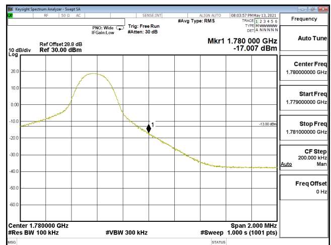
EDGE-ENDC_12A_n66-64QAM_10M_CH355000_1715(1,51)_SCS15KHz
