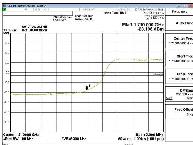
EDGE-ENDC_12A_n66-16QAM_10M_CH343000_1715(50,0)_SCS15KHz
