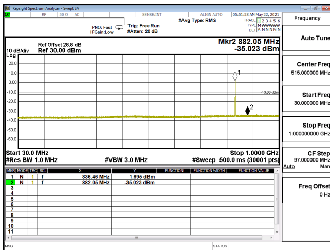
CSE-ENDC_5A_n2_64QAM_5M_CH381500_1907.5(1,12)-30M-1G
