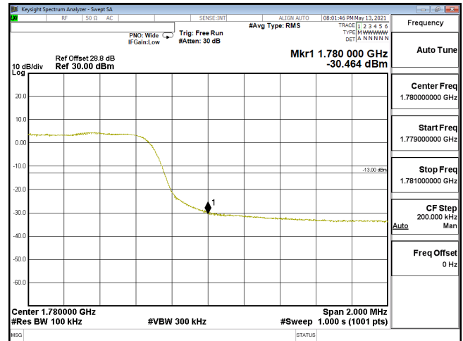
EDGE-ENDC_12A_n66-PI2-BPSK_10M_CH355000_1715(50,2)_SCS15KHz
