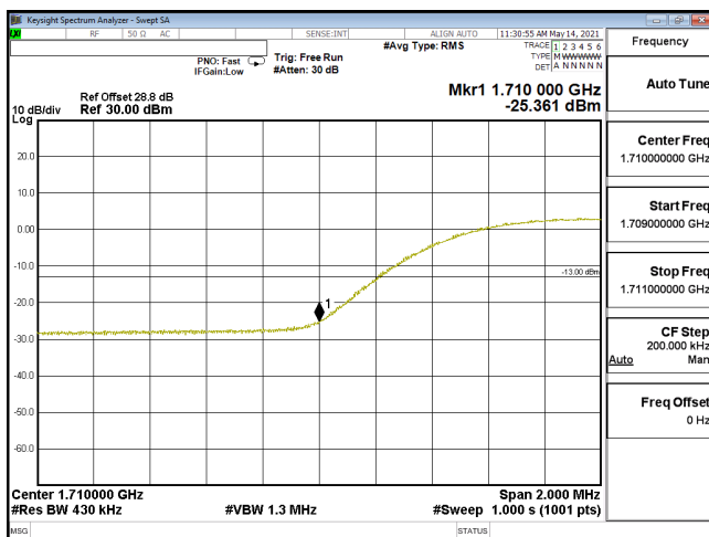
EDGE-ENDC_12A_n66-QPSK_40M_CH346000_1730(216,0)_SCS15KHz
