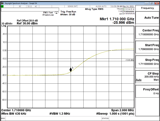
EDGE-ENDC_12A_n66-64QAM_40M_CH346000_1730(216,0)_SCS15KHz
