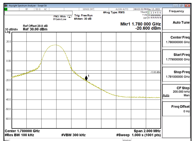
EDGE-ENDC_12A_n66-256QAM_10M_CH355000_1715(1,51)_SCS15KHz
