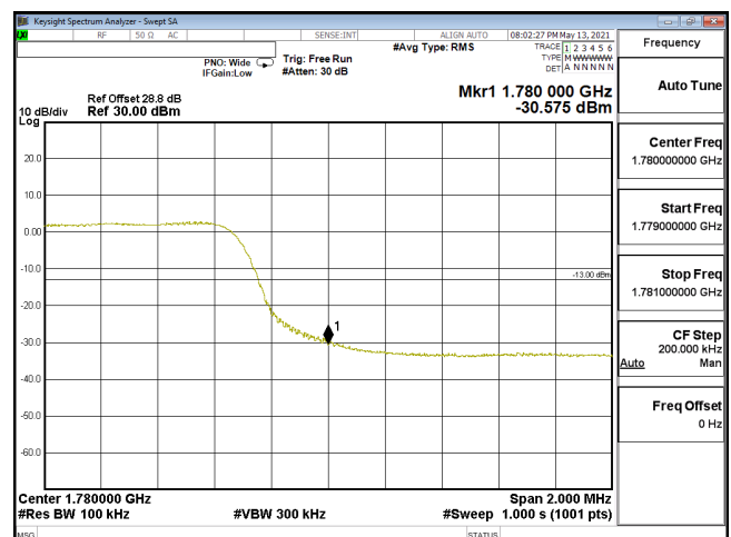
EDGE-ENDC_12A_n66-16QAM_10M_CH355000_1715(50,2)_SCS15KHz
