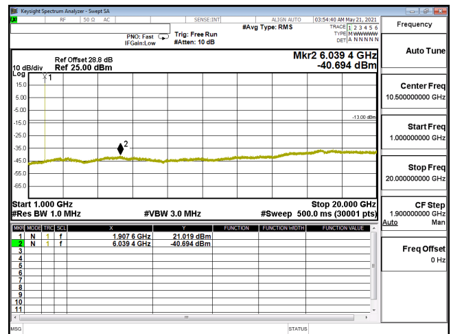
CSE-ENDC_5A_n2_64QAM_5M_CH381500_1907.5(1,12)-1G-20G
