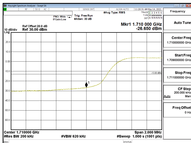
EDGE-ENDC_12A_n66-PI2-BPSK_20M_CH344000_1720(100,0)_SCS15KHz
