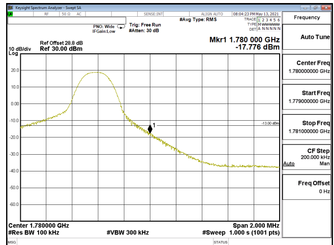
EDGE-ENDC_12A_n66-16QAM_10M_CH355000_1715(1,51)_SCS15KHz
