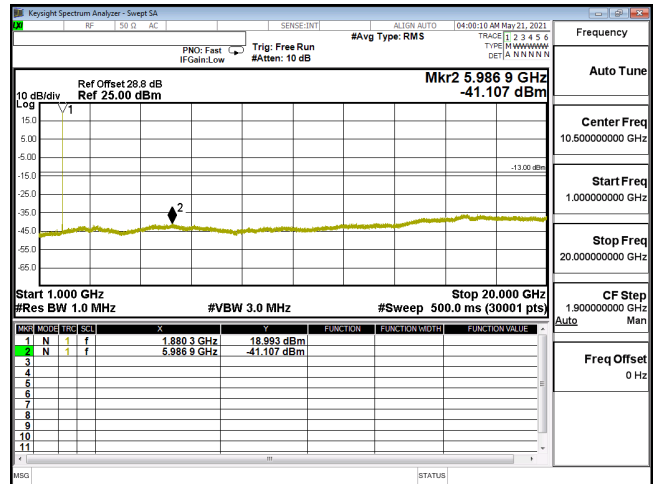
CSE-ENDC_5A_n2_256QAM_10M_CH376000_1880(1,26)-1G-20G
