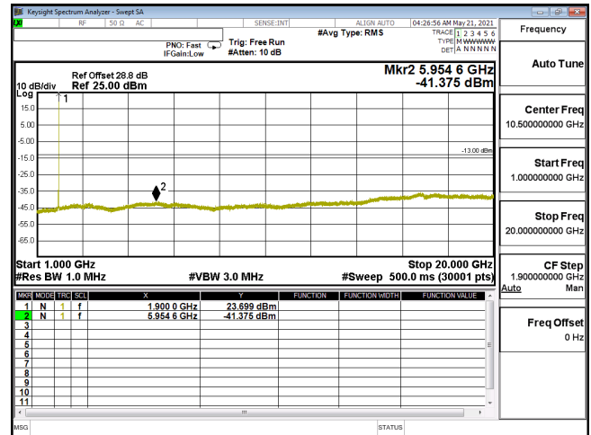
CSE-ENDC_5A_n2_16QAM_20M_CH380000_1900(1,53)-1G-20G
