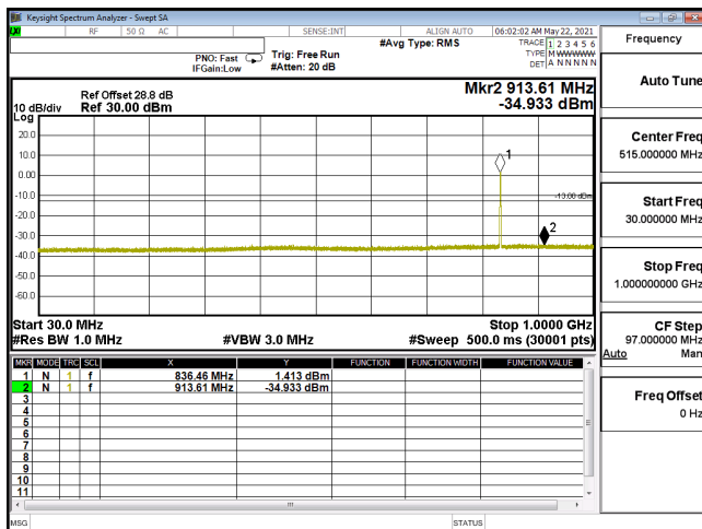
CSE-ENDC_5A_n2_64QAM_15M_CH380500_1902.5(1,39)-30M-1G
