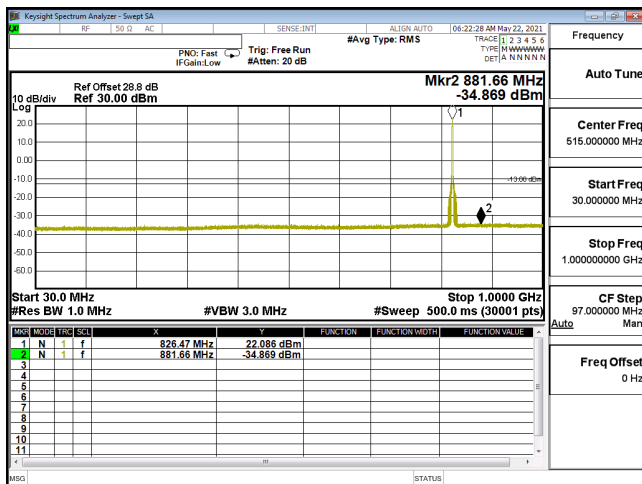
CSE-ENDC_30A_n5-256QAM_5M_CH165300_826.5(1,12)-30M-1G
