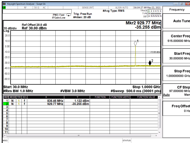
CSE-ENDC_5A_n2_QPSK_20M_CH376000_1880(1,53)-30M-1G
