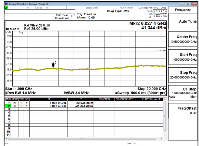
CSE-ENDC_5A_n2_16QAM_10M_CH381000_1905(1,26)-1G-20G
