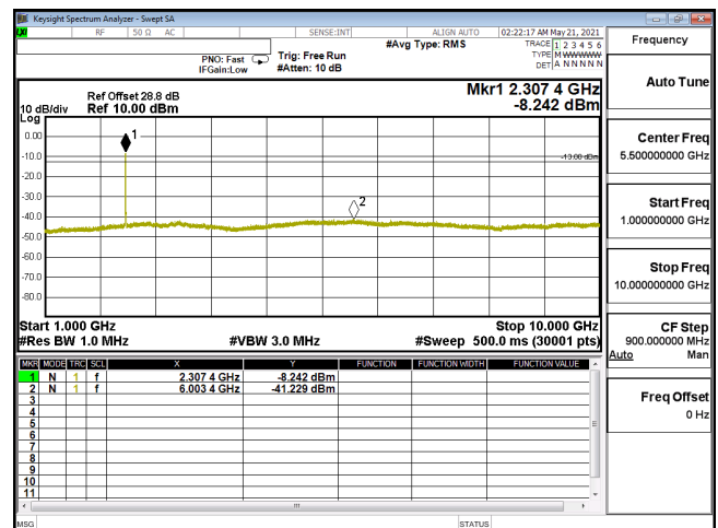
CSE-ENDC_30A_n5-64QAM_5M_CH167300_836.5(1,12)-1G-10G
