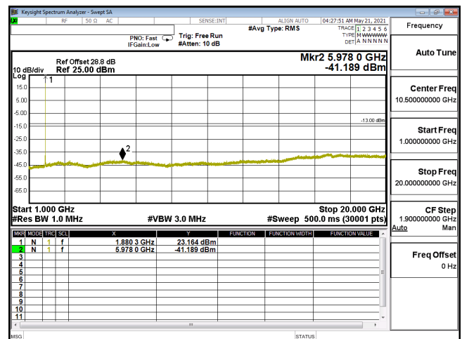
CSE-ENDC_5A_n2_PI2-BPSK_20M_CH376000_1880(1,53)-1G-20G
