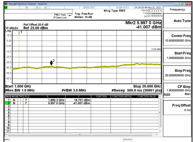
CSE-ENDC_5A_n2_256QAM_20M_CH376000_1880(1,53)-1G-20G
