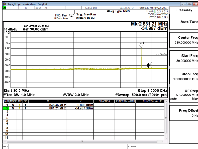
CSE-ENDC_5A_n2_16QAM_10M_CH381000_1905(1,26)-30M-1G
