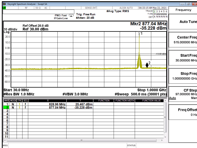
CSE-ENDC_30A_n5-PI2-BPSK_10M_CH165800_829(1,26)-30M-1G
