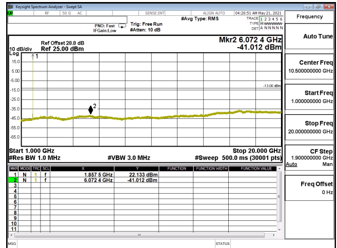
CSE-ENDC_5A_n2_64QAM_15M_CH371500_1857.5(1,39)-1G-20G
