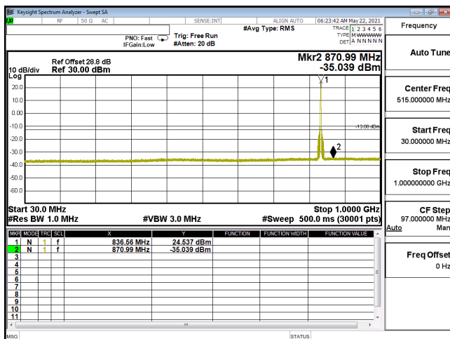
CSE-ENDC_30A_n5-64QAM_5M_CH167300_836.5(1,12)-30M-1G
