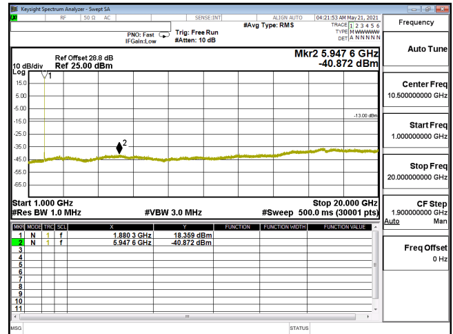
CSE-ENDC_5A_n2_256QAM_15M_CH376000_1880(1,39)-1G-20G
