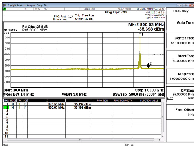
CSE-ENDC_30A_n5-QPSK_5M_CH169300_846.5(1,12)-30M-1G
