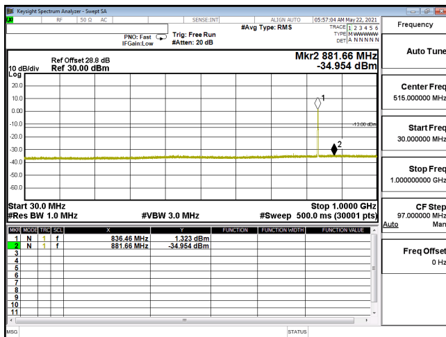
CSE-ENDC_5A_n2_64QAM_10M_CH381000_1905(1,26)-30M-1G
