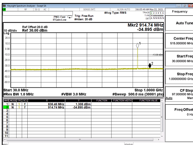
CSE-ENDC_5A_n2_QPSK_20M_CH380000_1900(1,53)-30M-1G
