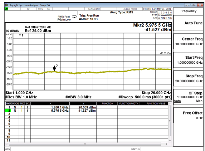
CSE-ENDC_5A_n2_256QAM_20M_CH372000_1860(1,53)-1G-20G
