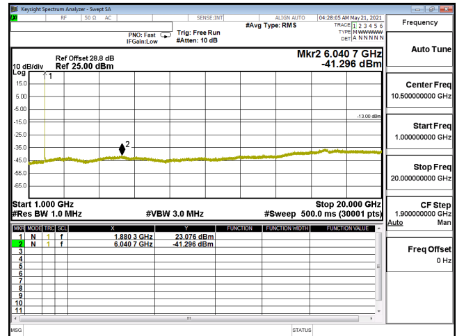
CSE-ENDC_5A_n2_QPSK_20M_CH376000_1880(1,53)-1G-20G
