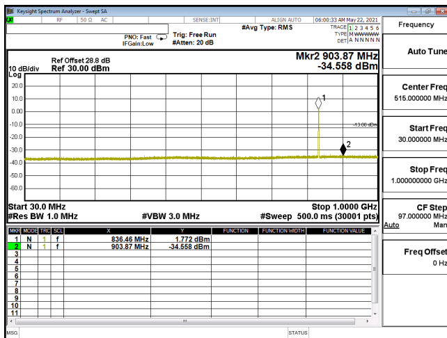
CSE-ENDC_5A_n2_PI2-BPSK_15M_CH380500_1902.5(1,39)-30M-1G
