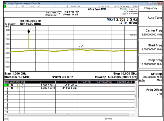
CSE-ENDC_30A_n5-64QAM_5M_CH165300_826.5(1,12)-1G-10G
