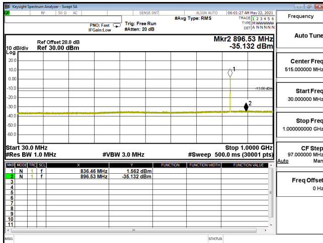
CSE-ENDC_5A_n2_16QAM_15M_CH380500_1902.5(1,39)-30M-1G
