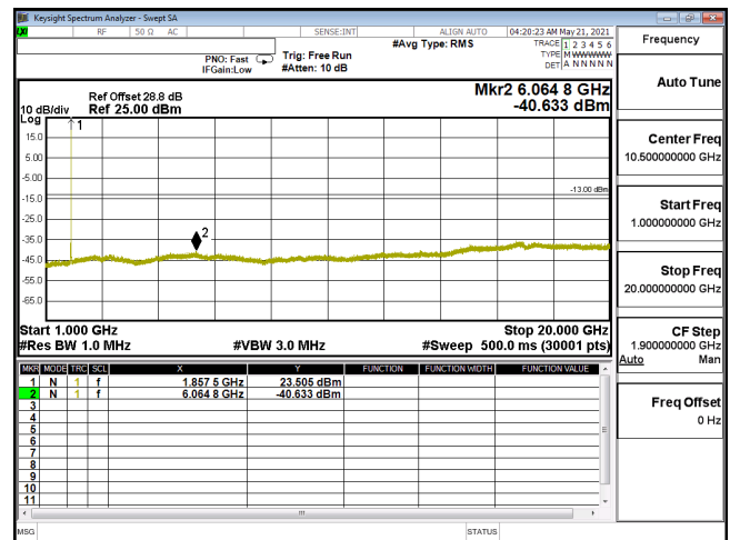
CSE-ENDC_5A_n2_QPSK_15M_CH371500_1857.5(1,39)-1G-20G
