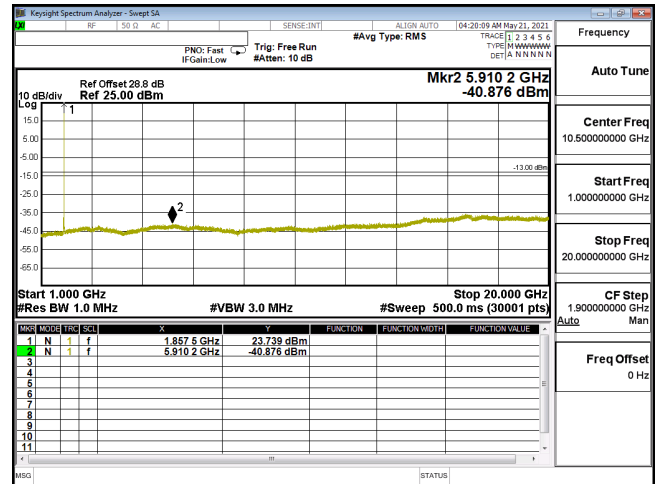
CSE-ENDC_5A_n2_PI2-BPSK_15M_CH371500_1857.5(1,39)-1G-20G
