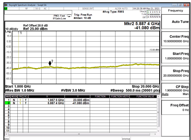
CSE-ENDC_5A_n2_16QAM_15M_CH371500_1857.5(1,39)-1G-20G
