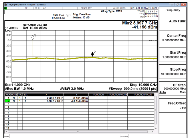
CSE-ENDC_30A_n5-16QAM_5M_CH165300_826.5(1,12)-1G-10G
