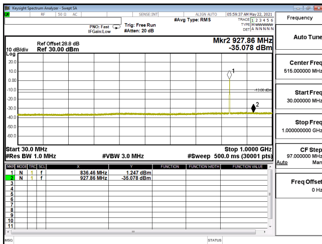
CSE-ENDC_5A_n2_16QAM_15M_CH376000_1880(1,39)-30M-1G
