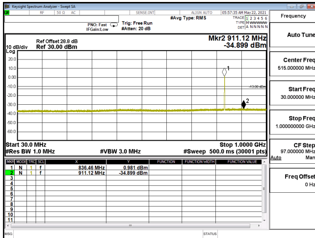
CSE-ENDC_5A_n2_PI2-BPSK_15M_CH371500_1857.5(1,39)-30M-1G
