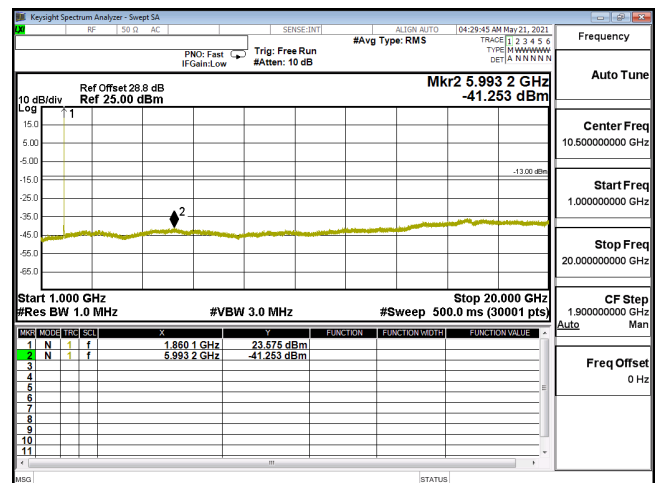
CSE-ENDC_5A_n2_16QAM_20M_CH372000_1860(1,53)-1G-20G
