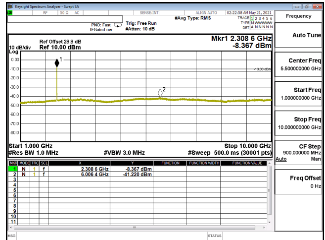
CSE-ENDC_30A_n5-QPSK_5M_CH167300_836.5(1,12)-1G-10G
