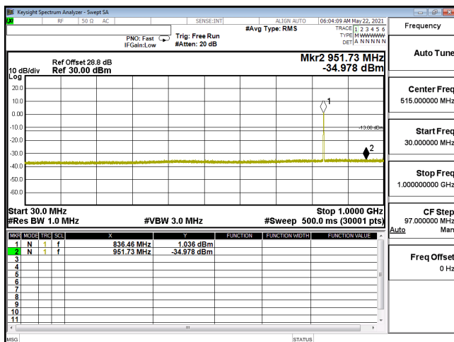
CSE-ENDC_5A_n2_PI2-BPSK_20M_CH376000_1880(1,53)-30M-1G
