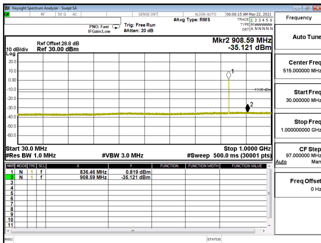
CSE-ENDC_5A_n2_64QAM_20M_CH380000_1900(1,53)-30M-1G
