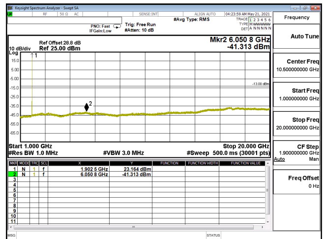
CSE-ENDC_5A_n2_PI2-BPSK_15M_CH380500_1902.5(1,39)-1G-20G
