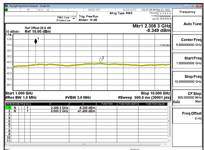
CSE-ENDC_30A_n5-16QAM_10M_CH165800_829(1,26)-1G-10G
