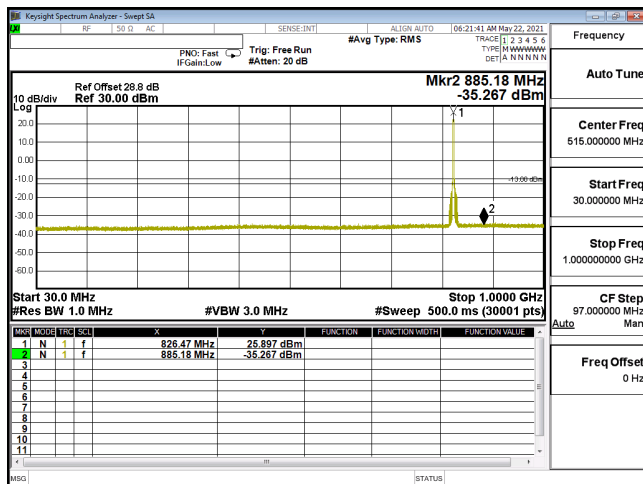
CSE-ENDC_30A_n5-16QAM_5M_CH165300_826.5(1,12)-30M-1G
