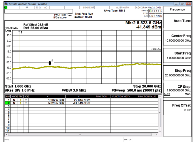
CSE-ENDC_5A_n2_16QAM_15M_CH380500_1902.5(1,39)-1G-20G
