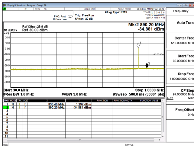
CSE-ENDC_5A_n2_16QAM_20M_CH372000_1860(1,53)-30M-1G
