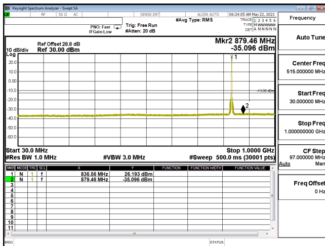
CSE-ENDC_30A_n5-16QAM_5M_CH167300_836.5(1,12)-30M-1G
