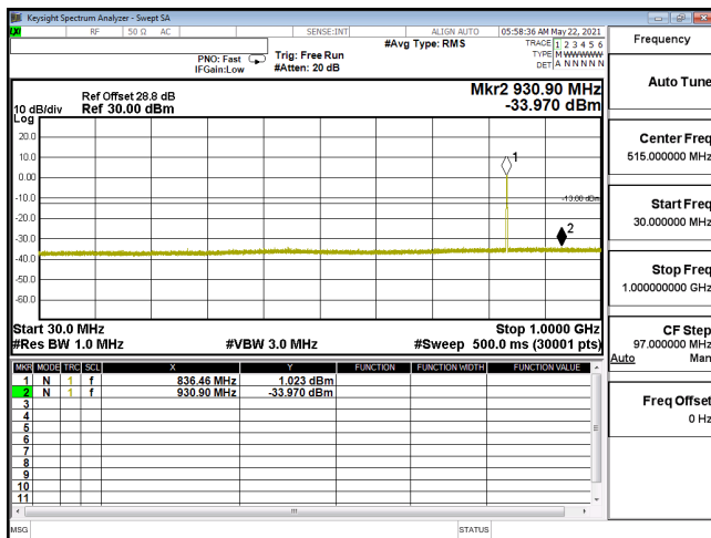
CSE-ENDC_5A_n2_256QAM_15M_CH371500_1857.5(1,39)-30M-1G
