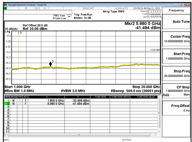
CSE-ENDC_5A_n2_PI2-BPSK_10M_CH381000_1905(1,26)-1G-20G
