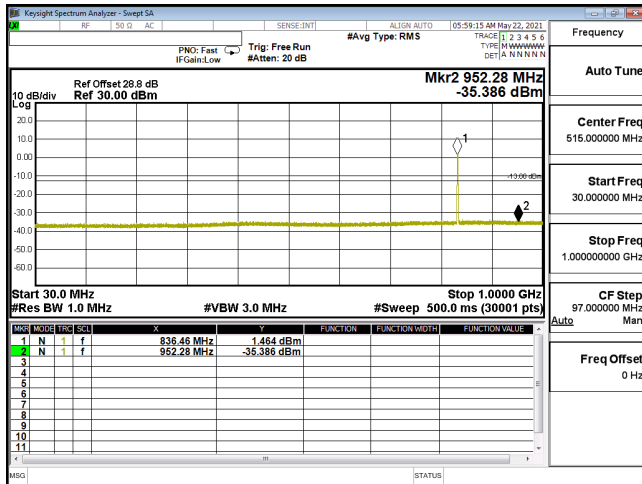
CSE-ENDC_5A_n2_QPSK_15M_CH376000_1880(1,39)-30M-1G
