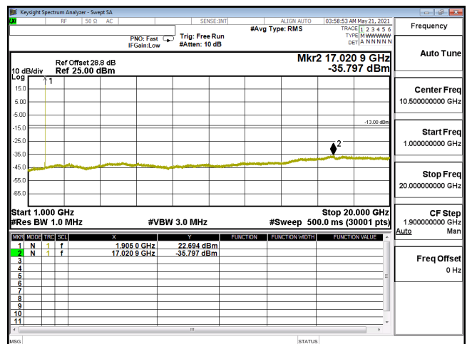
CSE-ENDC_5A_n2_QPSK_10M_CH381000_1905(1,26)-1G-20G
