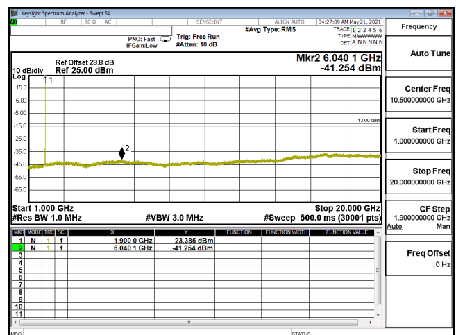
CSE-ENDC_5A_n2_QPSK_20M_CH380000_1900(1,53)-1G-20G
