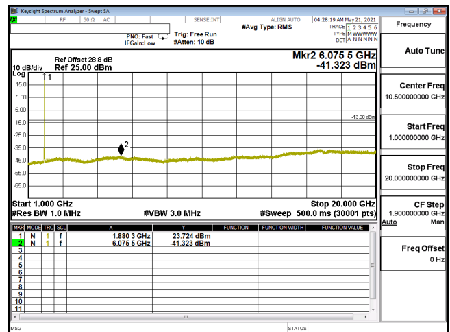
CSE-ENDC_5A_n2_16QAM_20M_CH376000_1880(1,53)-1G-20G
