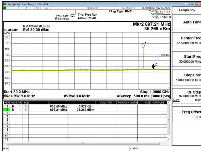
CSE-ENDC_5A_n2_PI2-BPSK_20M_CH372000_1860(1,53)-30M-1G
