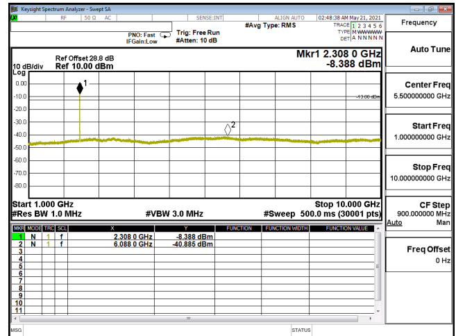
CSE-ENDC_30A_n5-PI2-BPSK_10M_CH165800_829(1,26)-1G-10G
