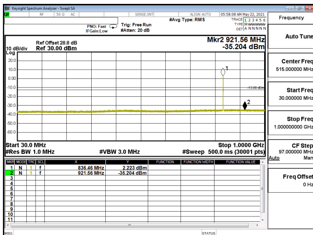
CSE-ENDC_5A_n2_16QAM_15M_CH371500_1857.5(1,39)-30M-1G
