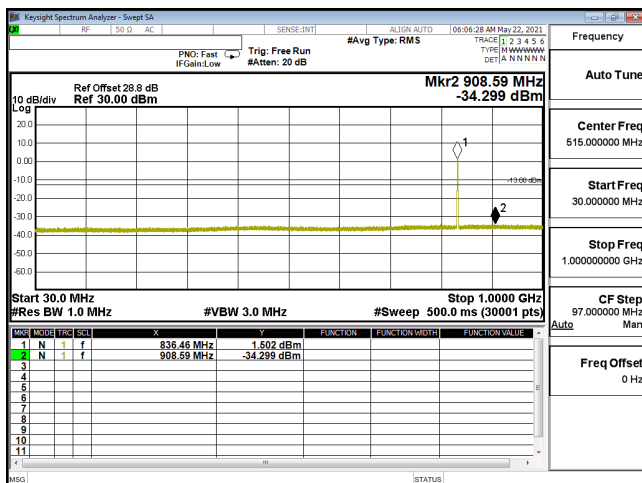
CSE-ENDC_5A_n2_256QAM_20M_CH380000_1900(1,53)-30M-1G
