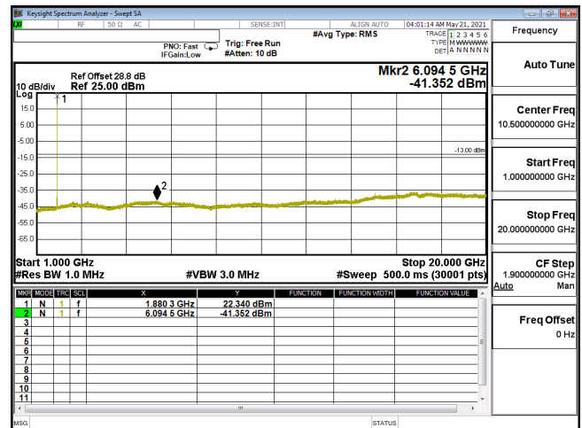
CSE-ENDC_5A_n2_QPSK_10M_CH376000_1880(1,26)-1G-20G
