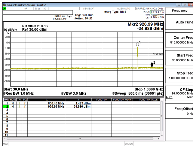
CSE-ENDC_5A_n2_QPSK_15M_CH371500_1857.5(1,39)-30M-1G
