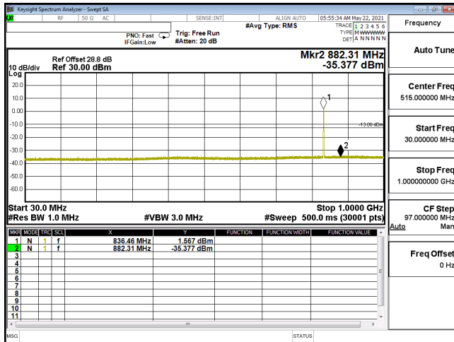
CSE-ENDC_5A_n2_256QAM_10M_CH376000_1880(1,26)-30M-1G
