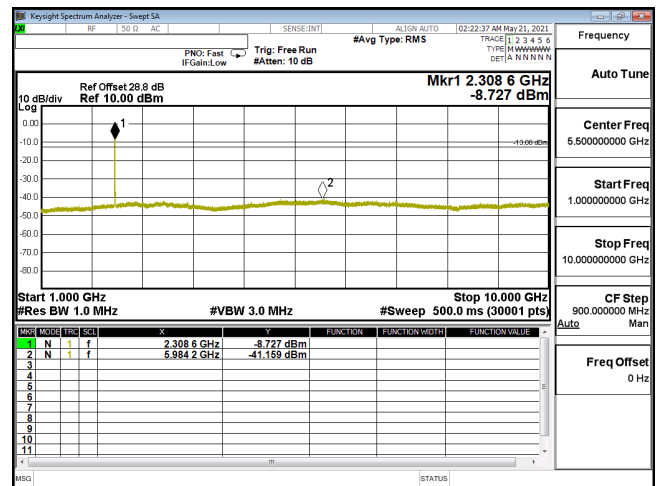
CSE-ENDC_30A_n5-16QAM_5M_CH167300_836.5(1,12)-1G-10G
