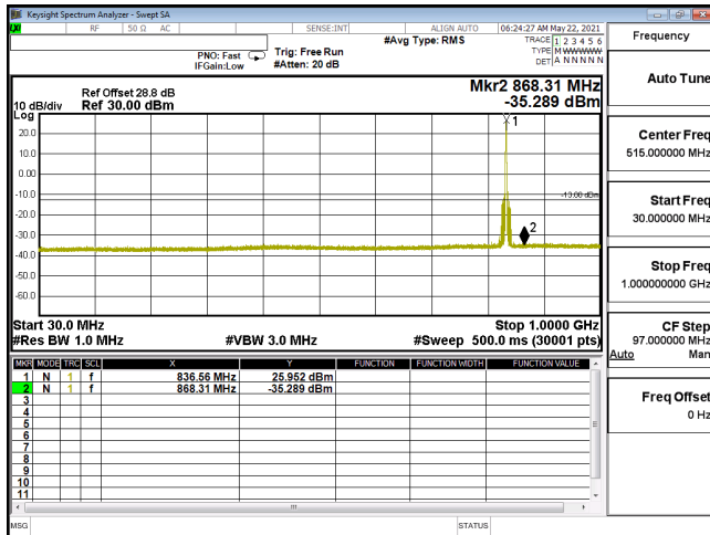
CSE-ENDC_30A_n5-QPSK_5M_CH167300_836.5(1,12)-30M-1G
