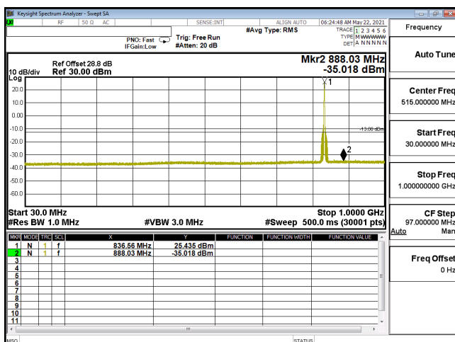
CSE-ENDC_30A_n5-PI2-BPSK_5M_CH167300_836.5(1,12)-30M-1G
