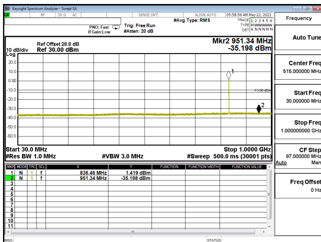
CSE-ENDC_5A_n2_PI2-BPSK_15M_CH376000_1880(1,39)-30M-1G
