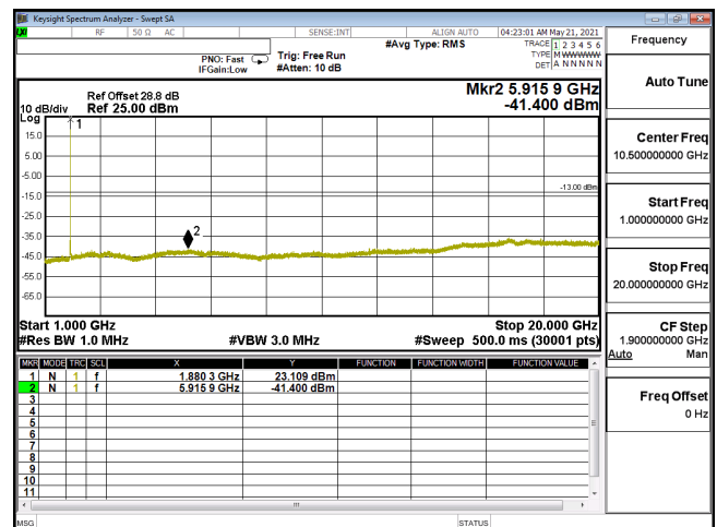
CSE-ENDC_5A_n2_PI2-BPSK_15M_CH376000_1880(1,39)-1G-20G
