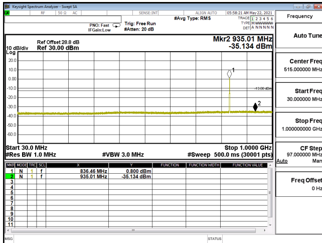
CSE-ENDC_5A_n2_64QAM_15M_CH371500_1857.5(1,39)-30M-1G
