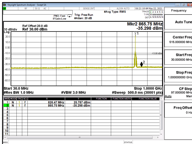
CSE-ENDC_30A_n5-QPSK_5M_CH165300_826.5(1,12)-30M-1G
