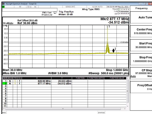
CSE-ENDC_30A_n5-QPSK_10M_CH165800_829(1,26)-30M-1G
