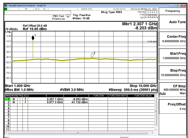
CSE-ENDC_30A_n5-PI2-BPSK_5M_CH167300_836.5(1,12)-1G-10G
