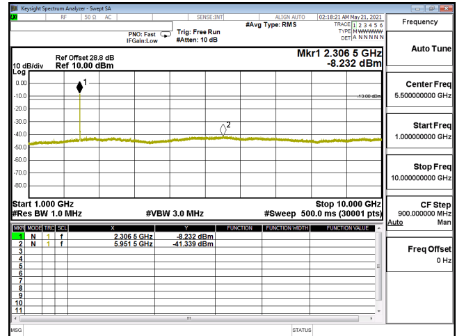
CSE-ENDC_30A_n5-PI2-BPSK_5M_CH165300_826.5(1,12)-1G-10G
