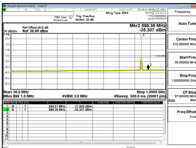
CSE-ENDC_30A_n5-256QAM_5M_CH169300_846.5(1,12)-30M-1G
