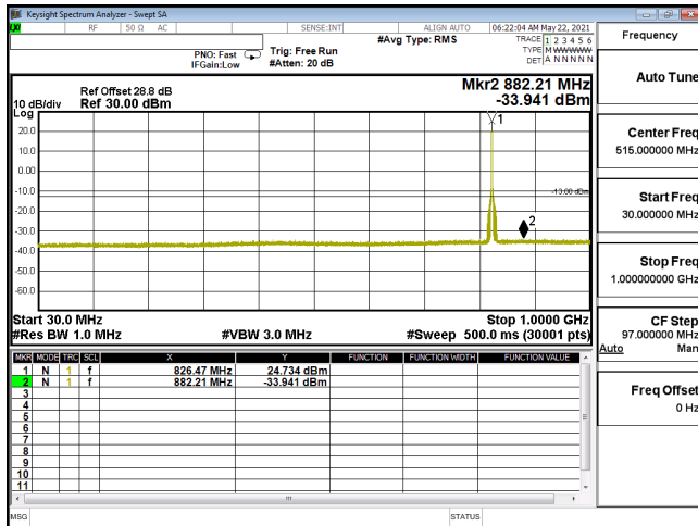
CSE-ENDC_30A_n5-64QAM_5M_CH165300_826.5(1,12)-30M-1G
