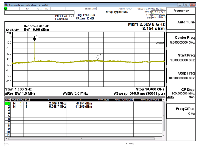
CSE-ENDC_30A_n5-PI2-BPSK_5M_CH169300_846.5(1,12)-1G-10G
