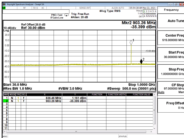
CSE-ENDC_5A_n2_QPSK_10M_CH376000_1880(1,26)-30M-1G
