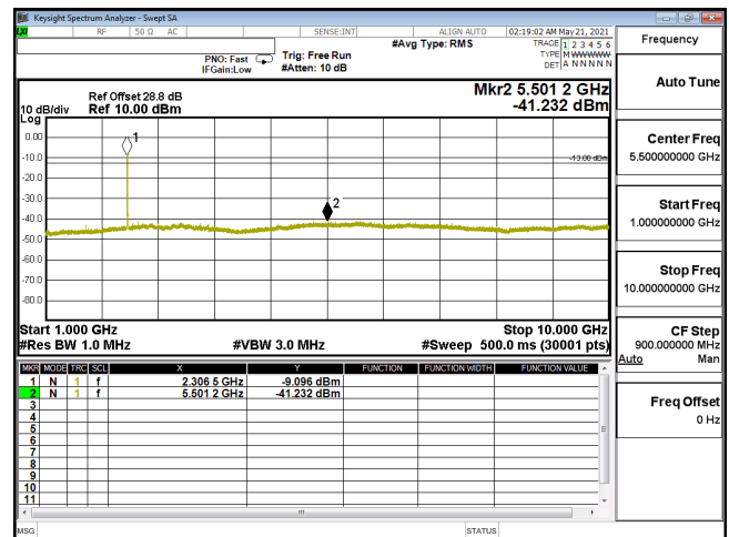
CSE-ENDC_30A_n5-QPSK_5M_CH165300_826.5(1,12)-1G-10G
