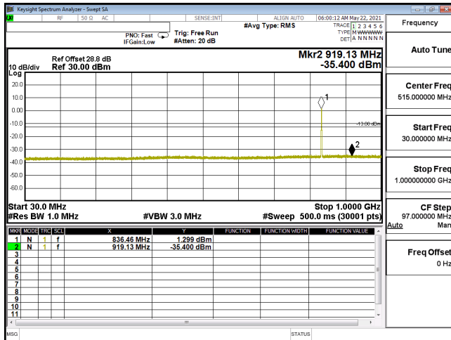
CSE-ENDC_5A_n2_256QAM_15M_CH376000_1880(1,39)-30M-1G
