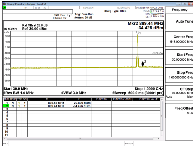
CSE-ENDC_30A_n5-256QAM_5M_CH167300_836.5(1,12)-30M-1G
