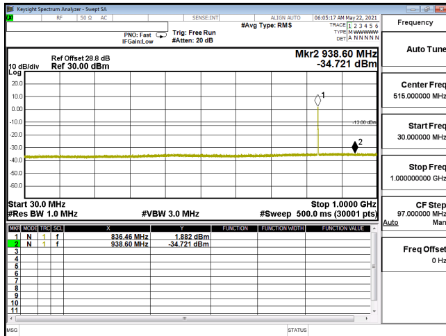
CSE-ENDC_5A_n2_256QAM_20M_CH376000_1880(1,53)-30M-1G
