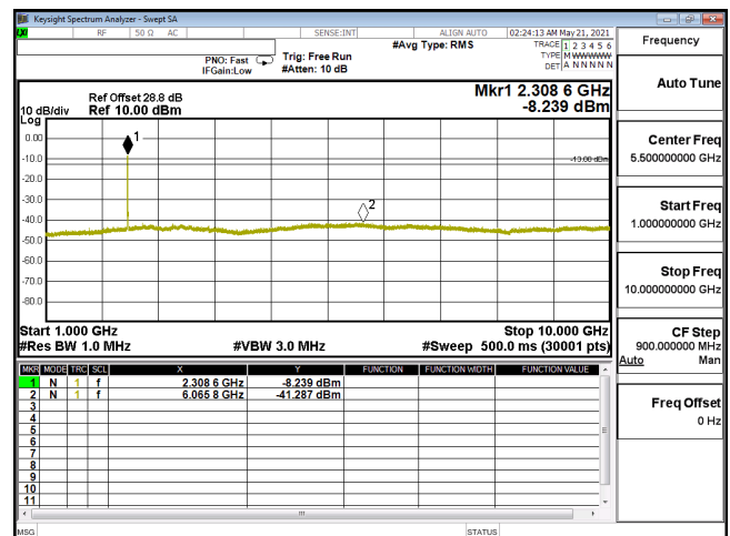
CSE-ENDC_30A_n5-QPSK_5M_CH169300_846.5(1,12)-1G-10G
