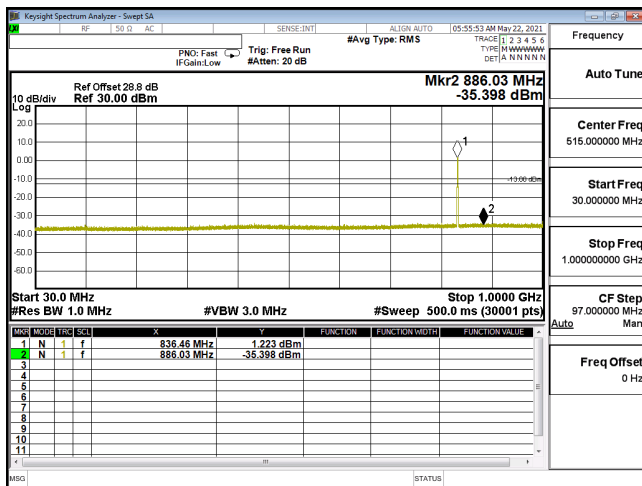
CSE-ENDC_5A_n2_PI2-BPSK_10M_CH381000_1905(1,26)-30M-1G
