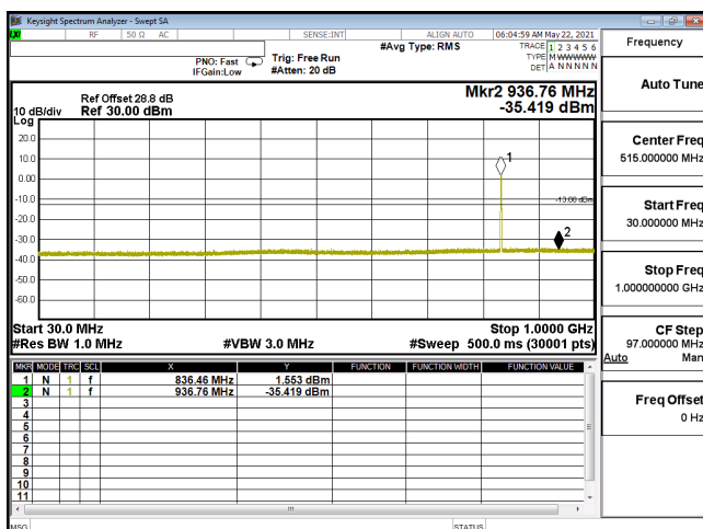
CSE-ENDC_5A_n2_64QAM_20M_CH376000_1880(1,53)-30M-1G
