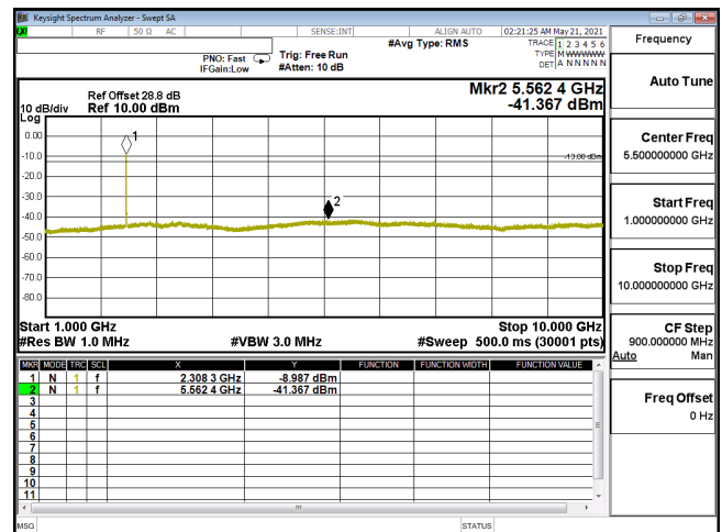
CSE-ENDC_30A_n5-256QAM_5M_CH165300_826.5(1,12)-1G-10G
