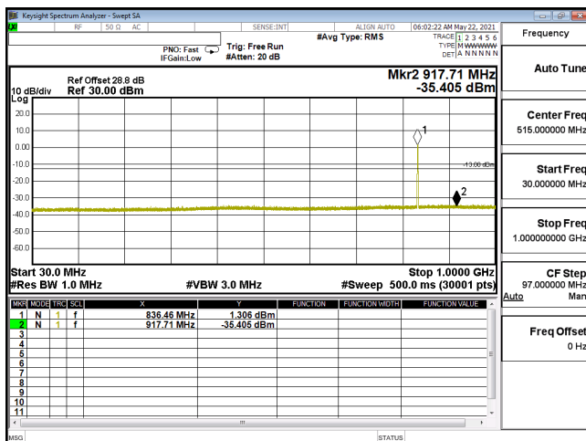
CSE-ENDC_5A_n2_256QAM_15M_CH380500_1902.5(1,39)-30M-1G
