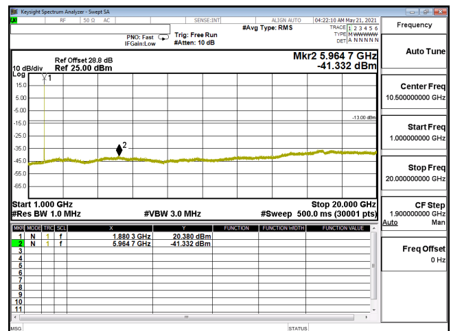
CSE-ENDC_5A_n2_64QAM_15M_CH376000_1880(1,39)-1G-20G
