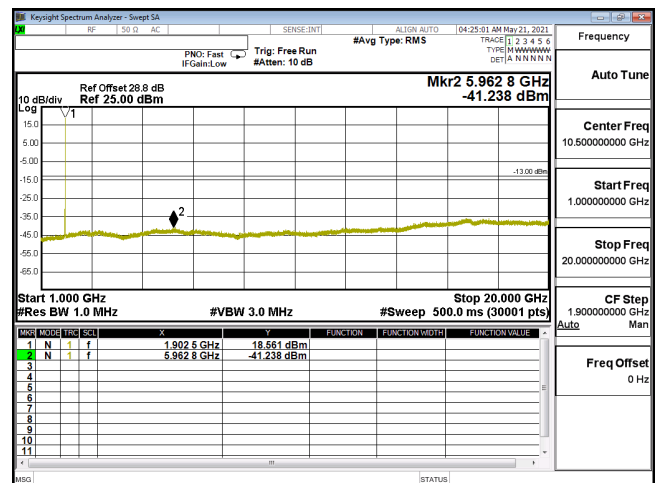
CSE-ENDC_5A_n2_256QAM_15M_CH380500_1902.5(1,39)-1G-20G
