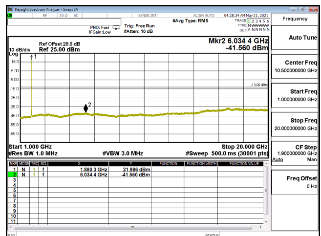
CSE-ENDC_5A_n2_64QAM_20M_CH376000_1880(1,53)-1G-20G
