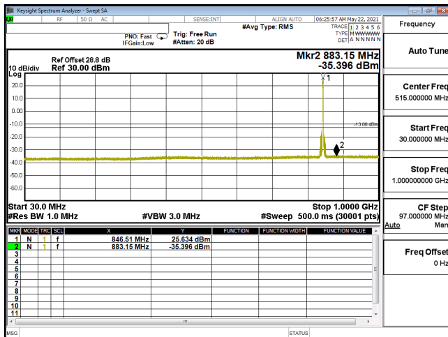
CSE-ENDC_30A_n5-16QAM_5M_CH169300_846.5(1,12)-30M-1G
