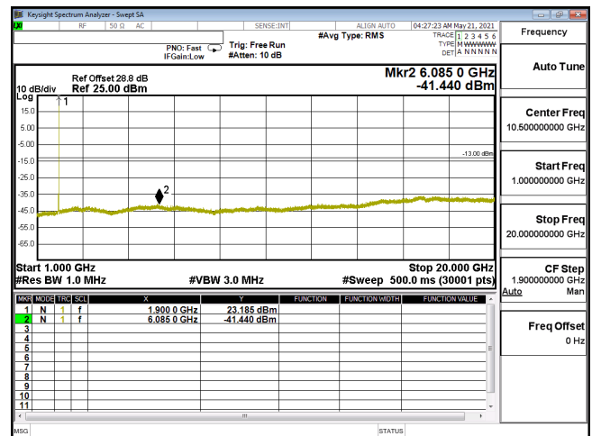
CSE-ENDC_5A_n2_PI2-BPSK_20M_CH380000_1900(1,53)-1G-20G
