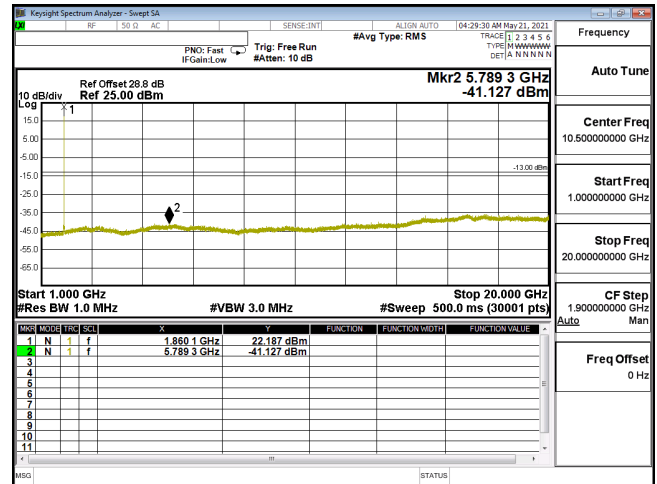
CSE-ENDC_5A_n2_64QAM_20M_CH372000_1860(1,53)-1G-20G
