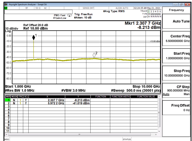
CSE-ENDC_30A_n5-16QAM_5M_CH169300_846.5(1,12)-1G-10G
