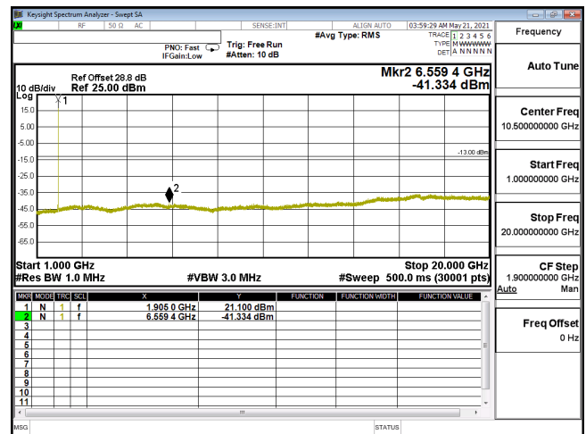
CSE-ENDC_5A_n2_64QAM_10M_CH381000_1905(1,26)-1G-20G
