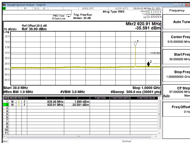
CSE-ENDC_5A_n2_16QAM_20M_CH376000_1880(1,53)-30M-1G
