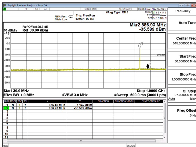
CSE-ENDC_5A_n2_QPSK_10M_CH381000_1905(1,26)-30M-1G
