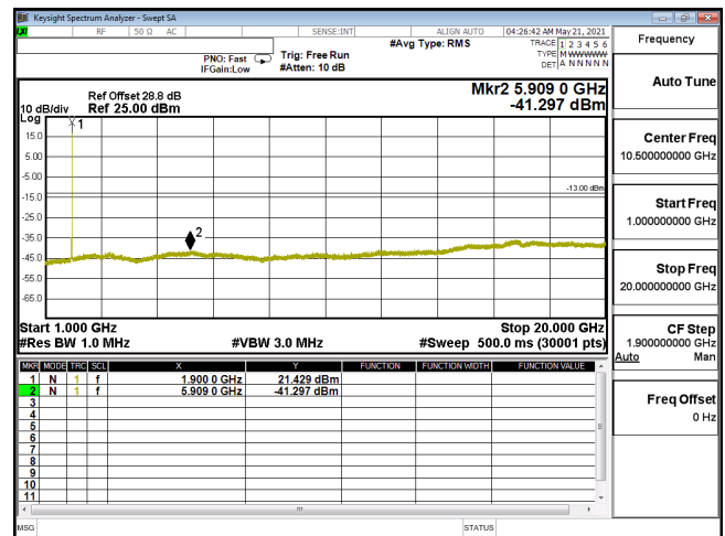
CSE-ENDC_5A_n2_64QAM_20M_CH380000_1900(1,53)-1G-20G
