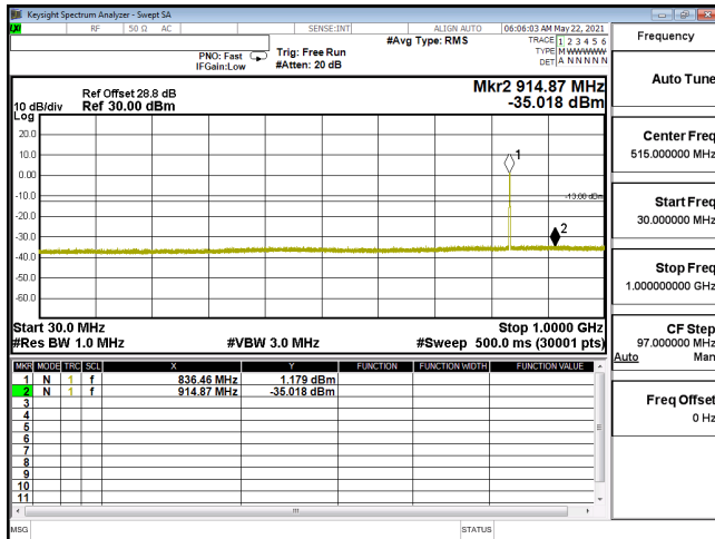
CSE-ENDC_5A_n2_16QAM_20M_CH380000_1900(1,53)-30M-1G
