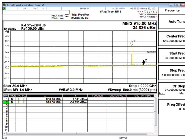
CSE-ENDC_5A_n2_64QAM_15M_CH376000_1880(1,39)-30M-1G
