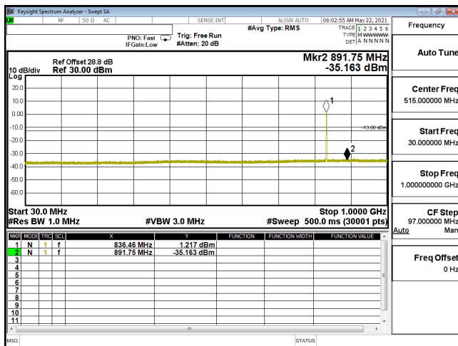
CSE-ENDC_5A_n2_QPSK_20M_CH372000_1860(1,53)-30M-1G
