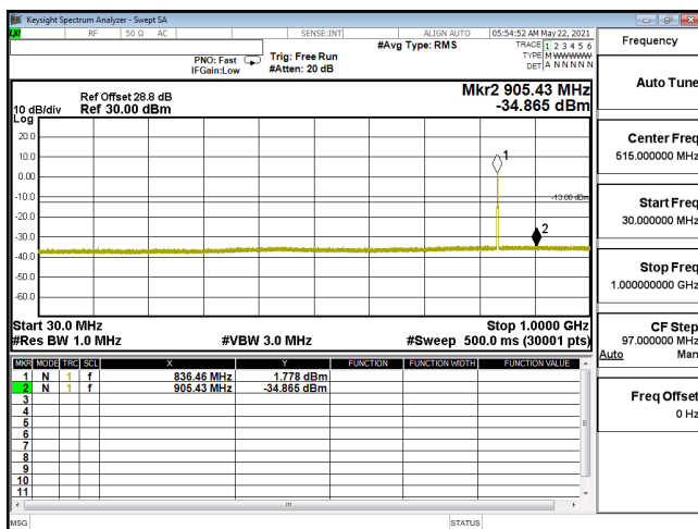
CSE-ENDC_5A_n2_16QAM_10M_CH376000_1880(1,26)-30M-1G
