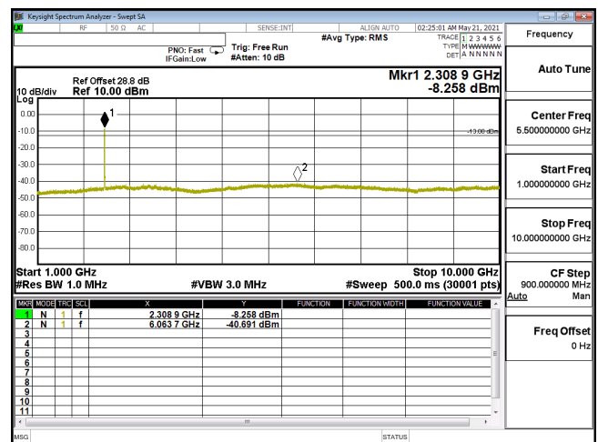
CSE-ENDC_30A_n5-64QAM_5M_CH169300_846.5(1,12)-1G-10G
