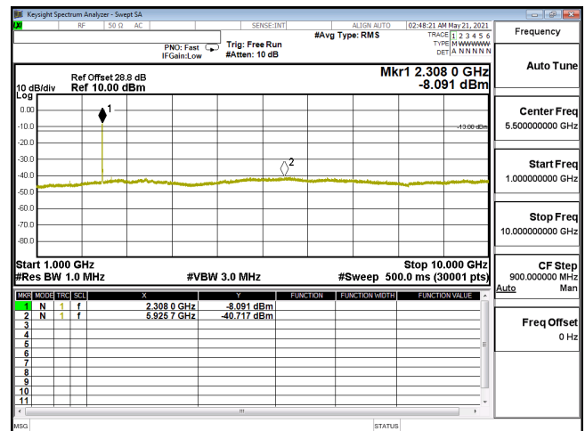
CSE-ENDC_30A_n5-QPSK_10M_CH165800_829(1,26)-1G-10G
