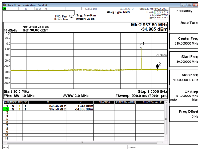
CSE-ENDC_5A_n2_PI2-BPSK_20M_CH380000_1900(1,53)-30M-1G
