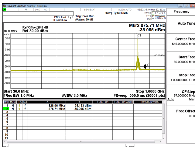
CSE-ENDC_30A_n5-16QAM_10M_CH165800_829(1,26)-30M-1G
