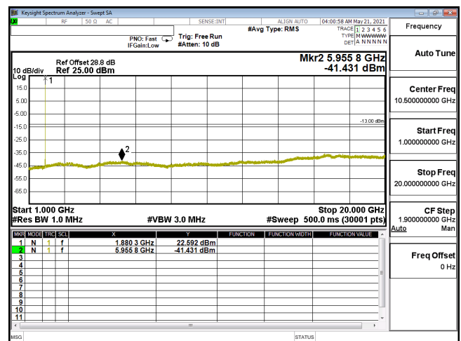
CSE-ENDC_5A_n2_16QAM_10M_CH376000_1880(1,26)-1G-20G
