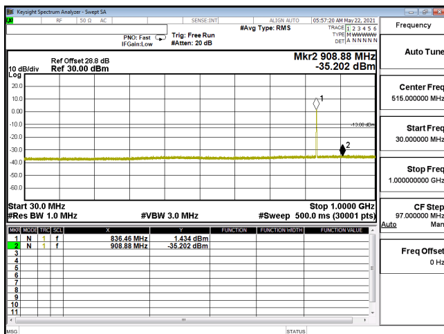
CSE-ENDC_5A_n2_256QAM_10M_CH381000_1905(1,26)-30M-1G
