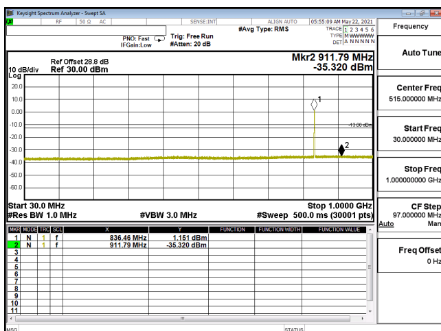
CSE-ENDC_5A_n2_64QAM_10M_CH376000_1880(1,26)-30M-1G
