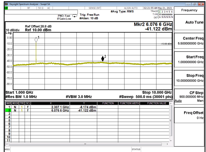
CSE-ENDC_30A_n5-256QAM_5M_CH167300_836.5(1,12)-1G-10G
