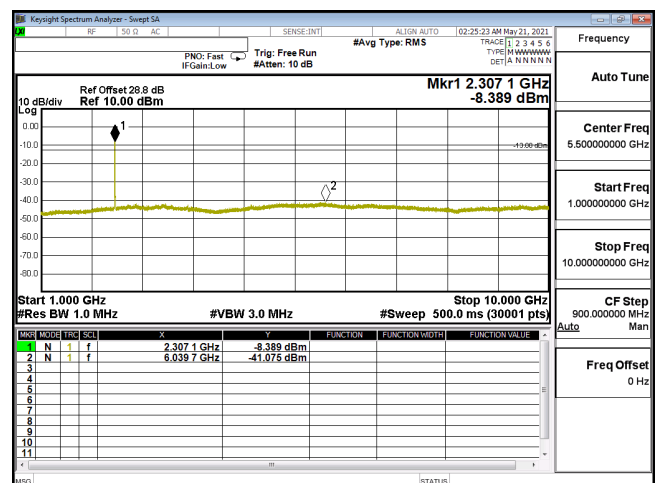
CSE-ENDC_30A_n5-256QAM_5M_CH169300_846.5(1,12)-1G-10G
