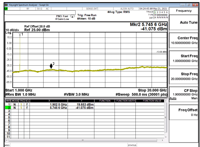
CSE-ENDC_5A_n2_64QAM_15M_CH380500_1902.5(1,39)-1G-20G
