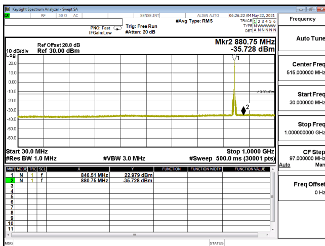
CSE-ENDC_30A_n5-64QAM_5M_CH169300_846.5(1,12)-30M-1G
