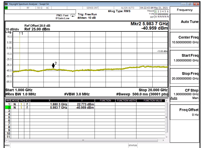
CSE-ENDC_5A_n2_QPSK_15M_CH376000_1880(1,39)-1G-20G
