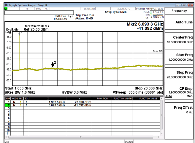
CSE-ENDC_5A_n2_QPSK_15M_CH380500_1902.5(1,39)-1G-20G
