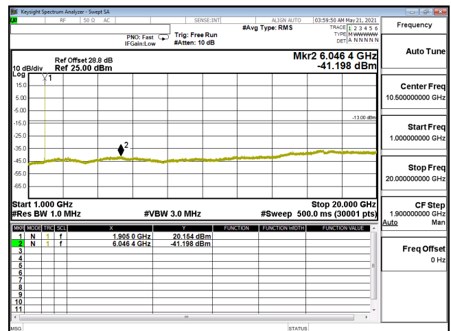
CSE-ENDC_5A_n2_256QAM_10M_CH381000_1905(1,26)-1G-20G
