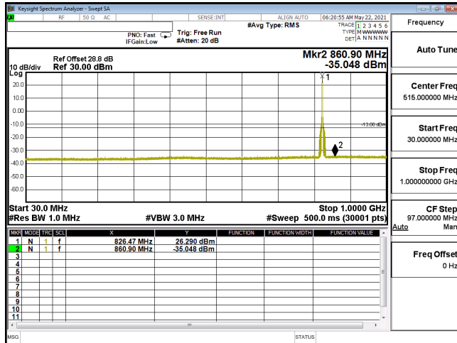
CSE-ENDC_30A_n5-PI2-BPSK_5M_CH165300_826.5(1,12)-30M-1G
