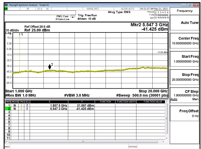
CSE-ENDC_5A_n2_256QAM_15M_CH371500_1857.5(1,39)-1G-20G
