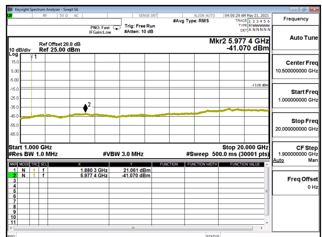
CSE-ENDC_5A_n2_64QAM_10M_CH376000_1880(1,26)-1G-20G
