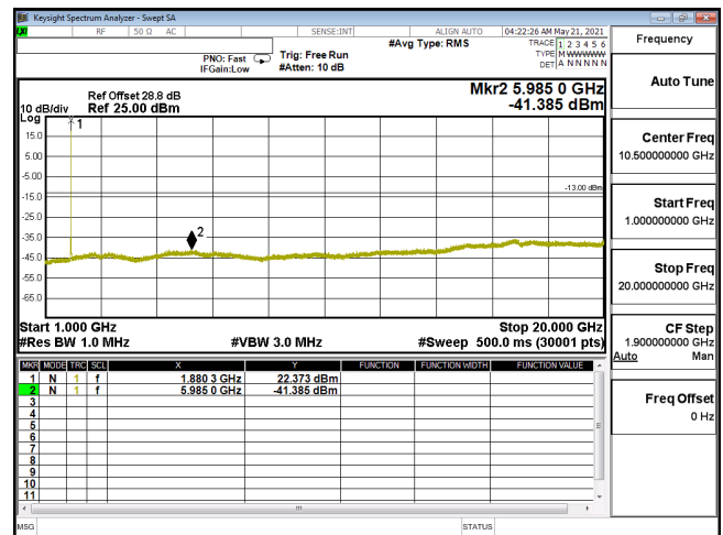
CSE-ENDC_5A_n2_16QAM_15M_CH376000_1880(1,39)-1G-20G
