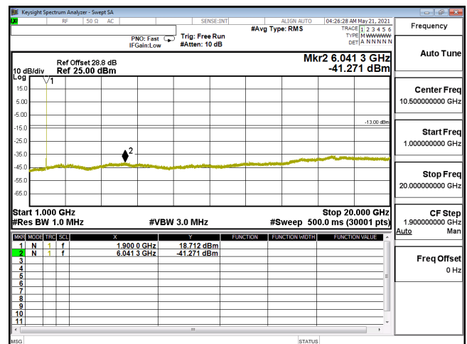
CSE-ENDC_5A_n2_256QAM_20M_CH380000_1900(1,53)-1G-20G
