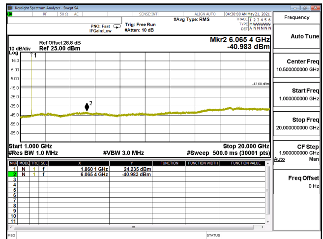
CSE-ENDC_5A_n2_QPSK_20M_CH372000_1860(1,53)-1G-20G
