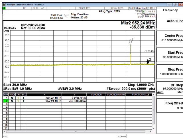
CSE-ENDC_5A_n2_256QAM_20M_CH372000_1860(1,53)-30M-1G
