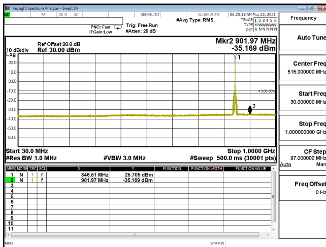
CSE-ENDC_30A_n5-PI2-BPSK_5M_CH169300_846.5(1,12)-30M-1G
