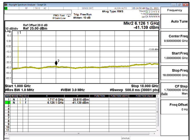
CSE-ENDC_12A_n66_256QAM_15M_CH343500_1717.5(1,39)-1G-18G
