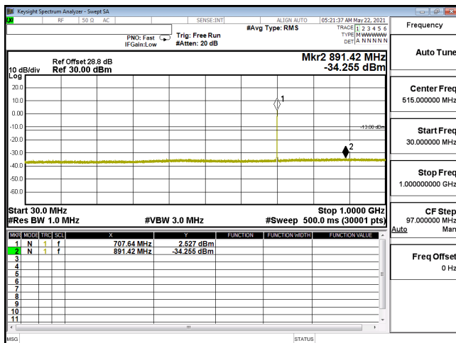
CSE-ENDC_12A_n66_16QAM_40M_CH349000_1745(1,108)-30M-1G
