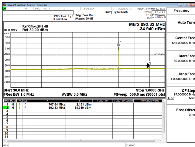
CSE-ENDC_12A_n66_QPSK_15M_CH343500_1717.5(1,39)-30M-1G
