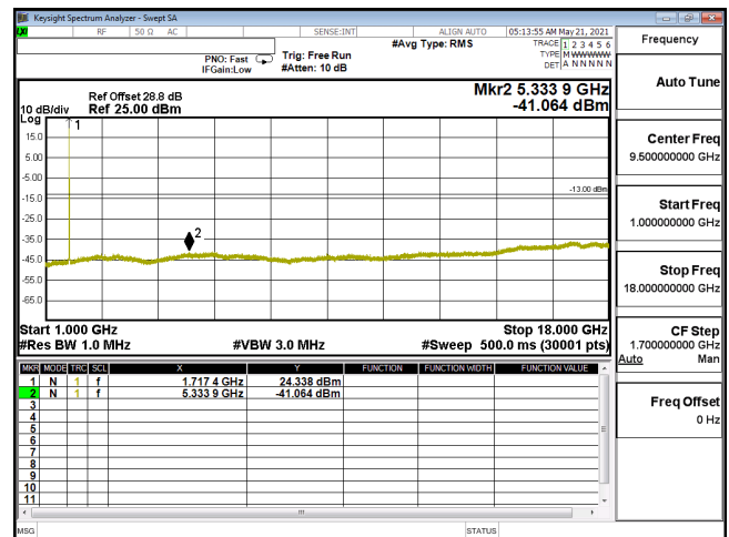
CSE-ENDC_12A_n66_QPSK_15M_CH343500_1717.5(1,39)-1G-18G
