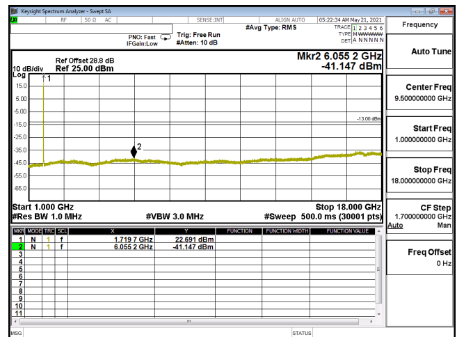
CSE-ENDC_12A_n66_QPSK_20M_CH344000_1720(1,53)-1G-18G
