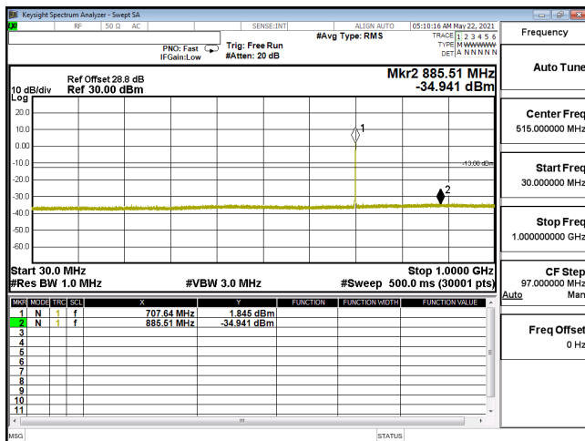
CSE-ENDC_12A_n66_256QAM_15M_CH343500_1717.5(1,39)-30M-1G
