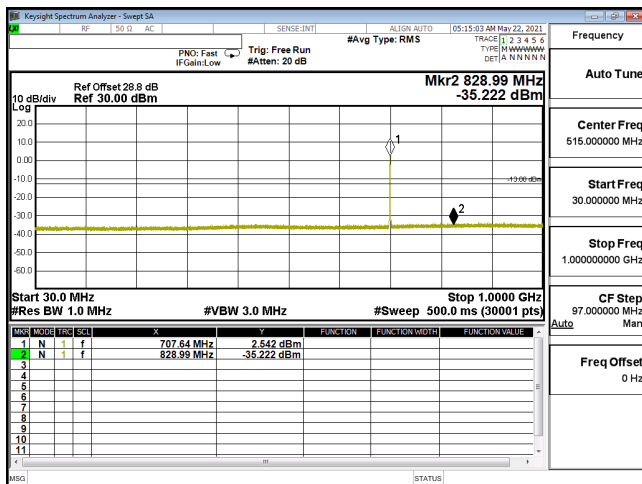
CSE-ENDC_12A_n66_QPSK_20M_CH344000_1720(1,53)-30M-1G
