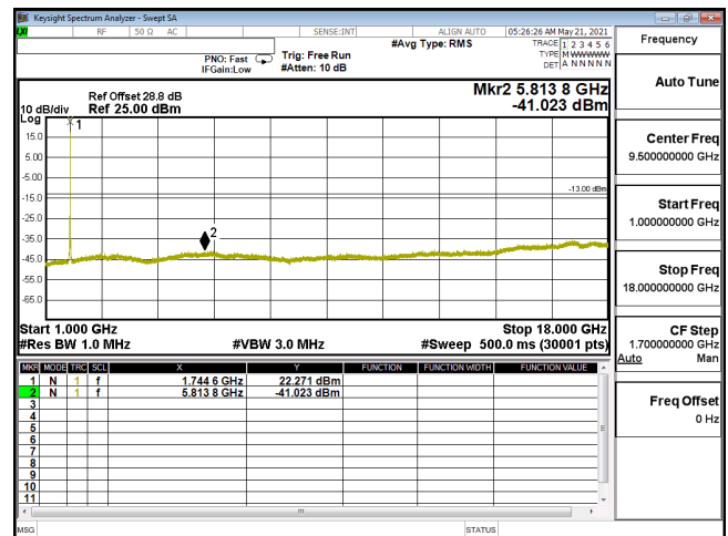
CSE-ENDC_12A_n66_16QAM_40M_CH349000_1745(1,108)-1G-18G
