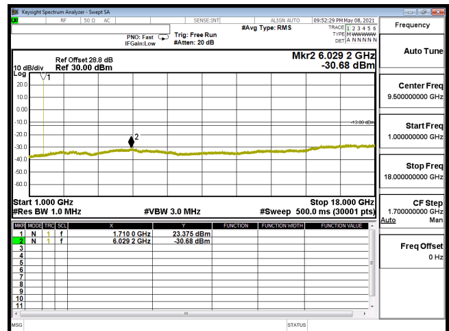
CSE-B66_1.4M-CH131979-16QAM(1,0)-1G-18G
