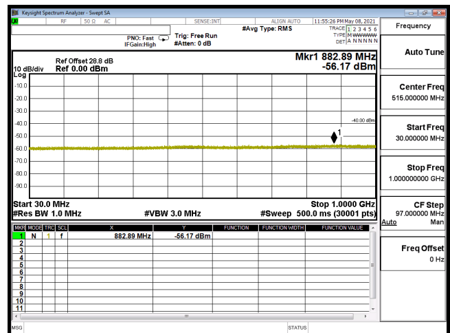
CSE-B30_5M-CH27685-16QAM(1,24)-30M-1G
