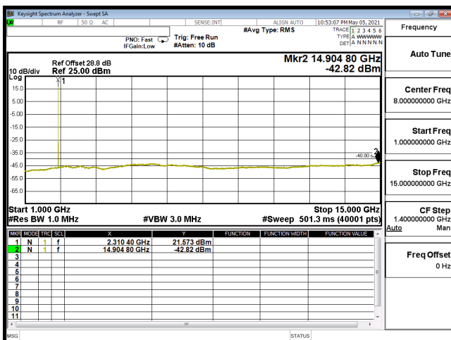
CSE-B30_5M-CH27735-16QAM(1,0)-1G-15G
