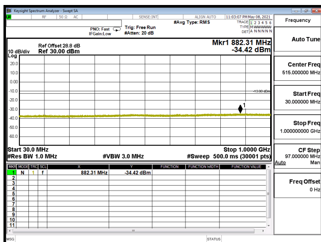
CSE-B66_3M-CH131987-64QAM(1,14)-30M-1G
