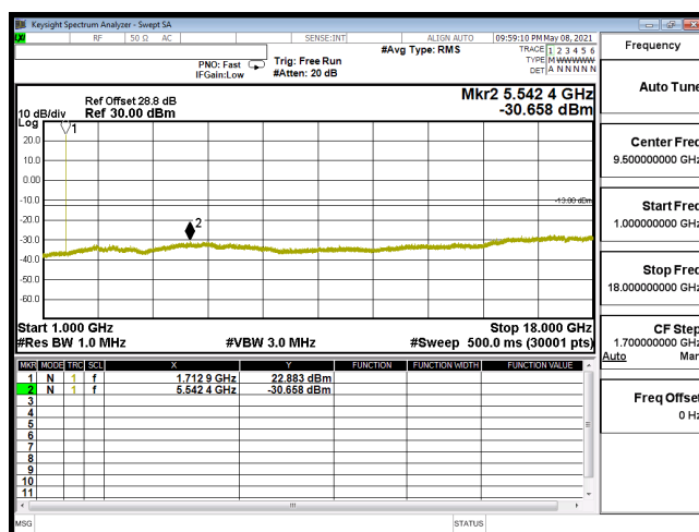
CSE-B66_3M-CH131987-16QAM(1,14)-1G-18G
