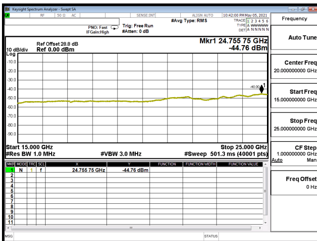
CSE-B30_5M-CH27735-64QAM(1,12)-15G-25G
