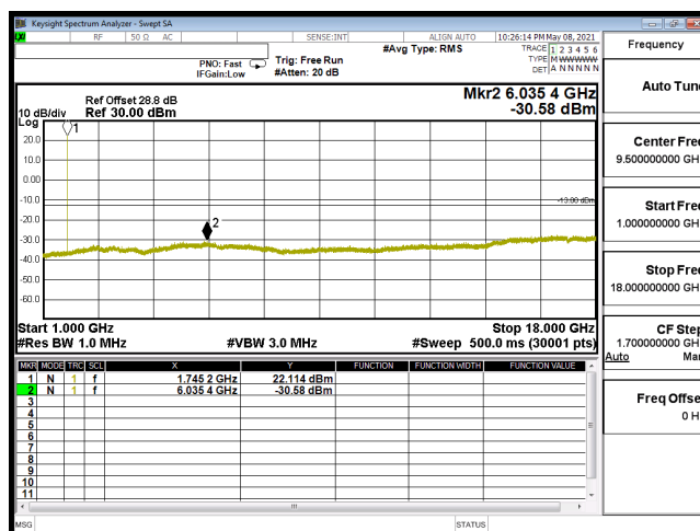
CSE-B66_5M-CH132322-64QAM(1,12)-1G-18G
