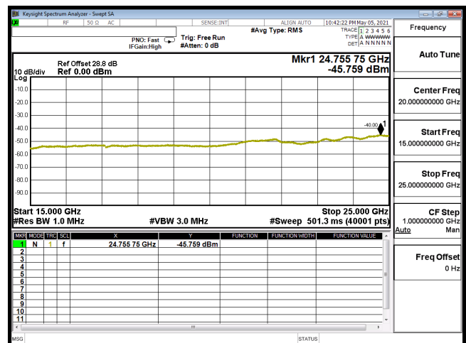
CSE-B30_5M-CH27735-16QAM(1,0)-15G-25G
