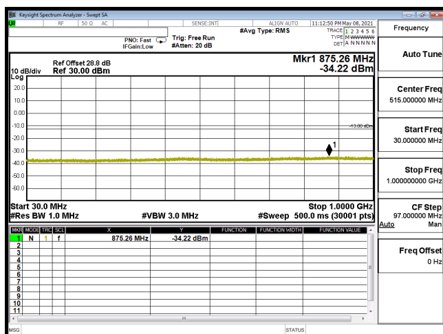
CSE-B66_10M-CH132022-QPSK(1,25)-30M-1G
