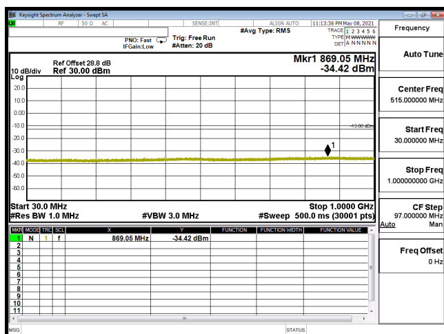
CSE-B66_10M-CH132322-64QAM(1,25)-30M-1G
