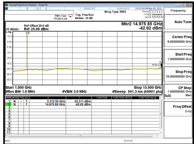
CSE-B30_5M-CH27735-QPSK(1,12)-1G-15G
