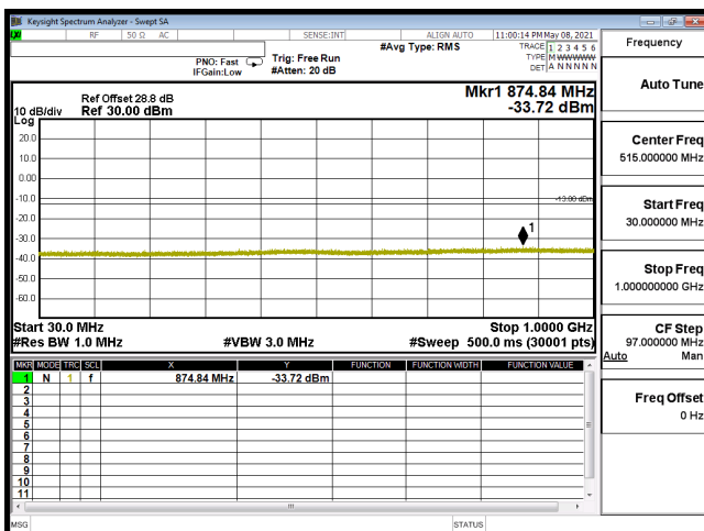
CSE-B66_1.4M-CH132665-64QAM(1,2)-30M-1G
