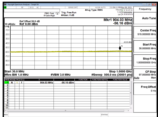
CSE-B30_5M-CH27710-64QAM(1,0)-30M-1G
