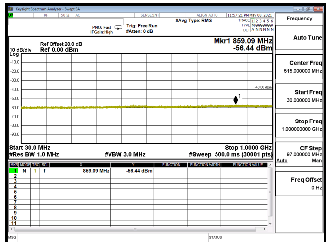
CSE-B30_10M-CH27710-64QAM(1,25)-30M-1G
