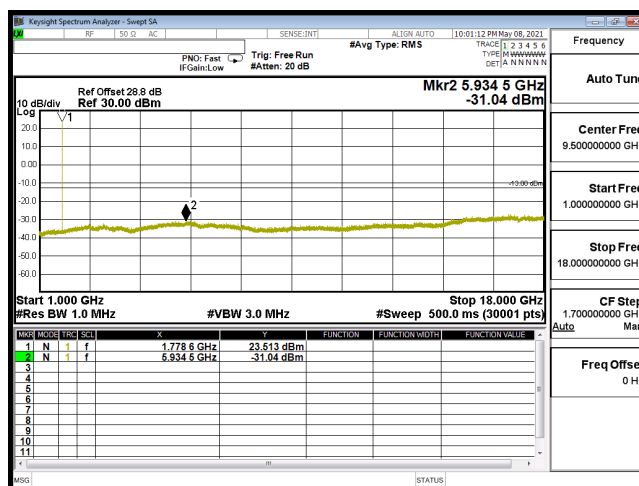
CSE-B66_3M-CH132657-QPSK(1,7)-1G-18G
