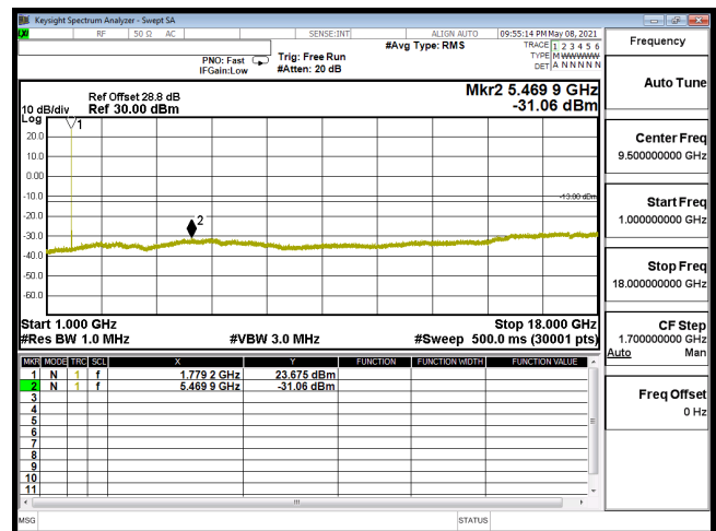
CSE-B66_1.4M-CH132665-16QAM(1,2)-1G-18G
