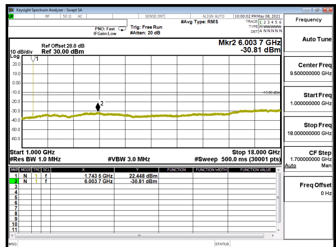
CSE-B66_3M-CH132322-64QAM(1,0)-1G-18G
