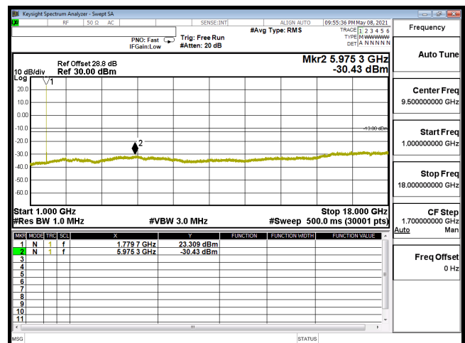
CSE-B66_1.4M-CH132665-64QAM(1,2)-1G-18G
