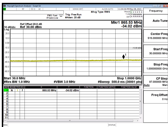
CSE-B66_3M-CH132657-16QAM(1,7)-30M-1G
