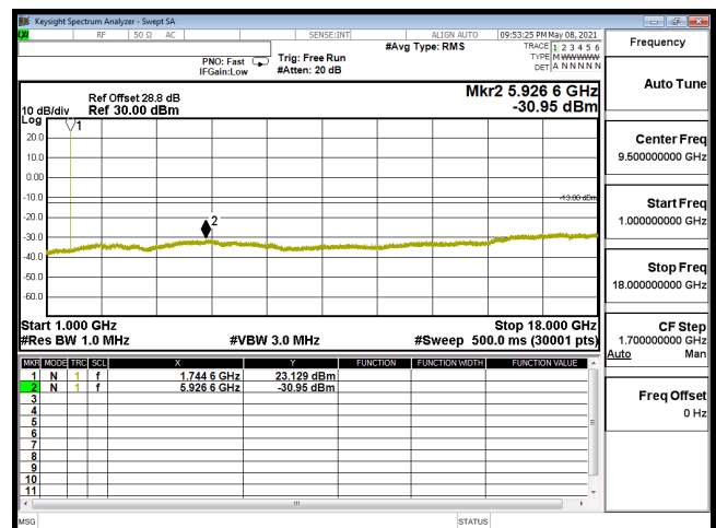
CSE-B66_1.4M-CH132322-64QAM(1,0)-1G-18G
