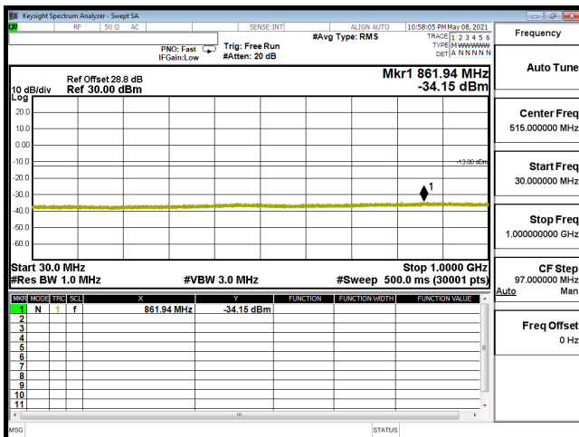
CSE-B66_1.4M-CH131979-64QAM(1,0)-30M-1G
