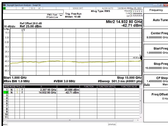
CSE-B30_5M-CH27710-64QAM(1,0)-1G-15G
