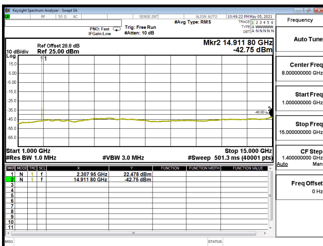
CSE-B30_5M-CH27710-QPSK(1,0)-1G-15G
