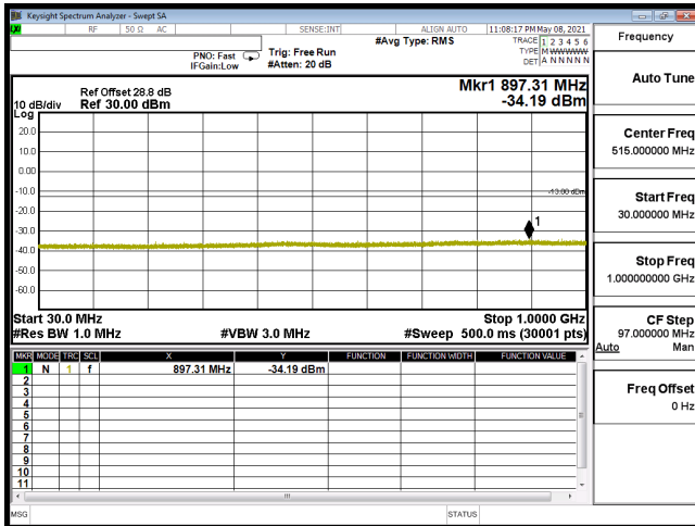
CSE-B66_5M-CH131997-QPSK(1,12)-30M-1G
