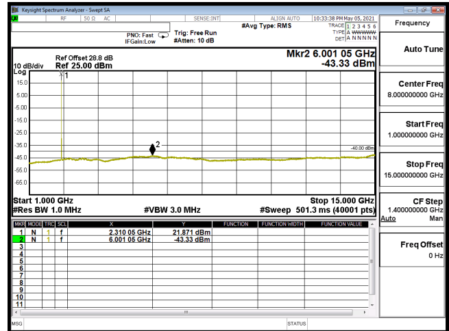
CSE-B30_10M-CH27710-16QAM(1,25)-1G-15G
