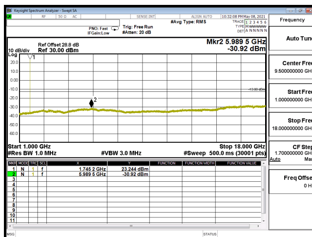
CSE-B66_10M-CH132322-64QAM(1,25)-1G-18G
