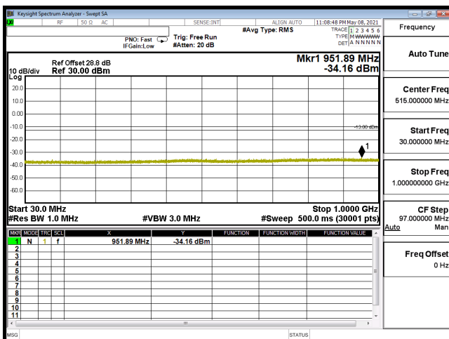
CSE-B66_5M-CH131997-64QAM(1,24)-30M-1G
