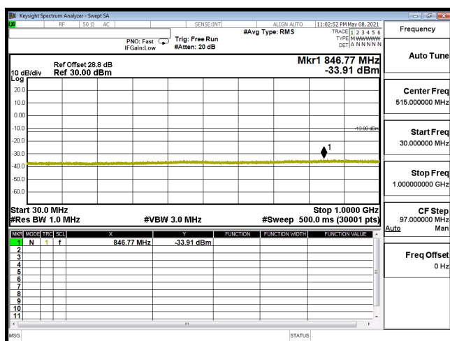
CSE-B66_3M-CH131987-16QAM(1,14)-30M-1G
