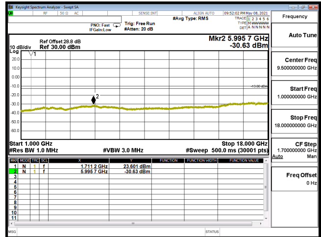
CSE-B66_1.4M-CH131979-QPSK(1,5)-1G-18G
