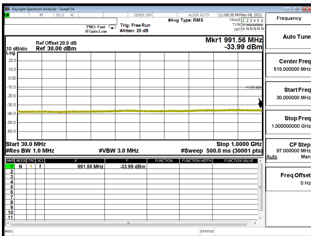
CSE-B66_5M-CH131997-16QAM(1,12)-30M-1G
