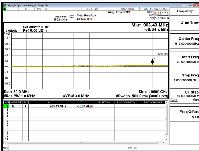
CSE-B30_5M-CH27735-QPSK(1,12)-30M-1G
