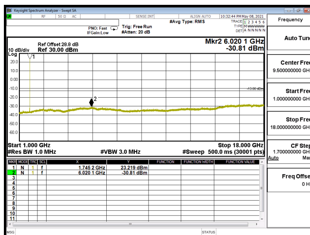
CSE-B66_10M-CH132322-QPSK(1,25)-1G-18G
