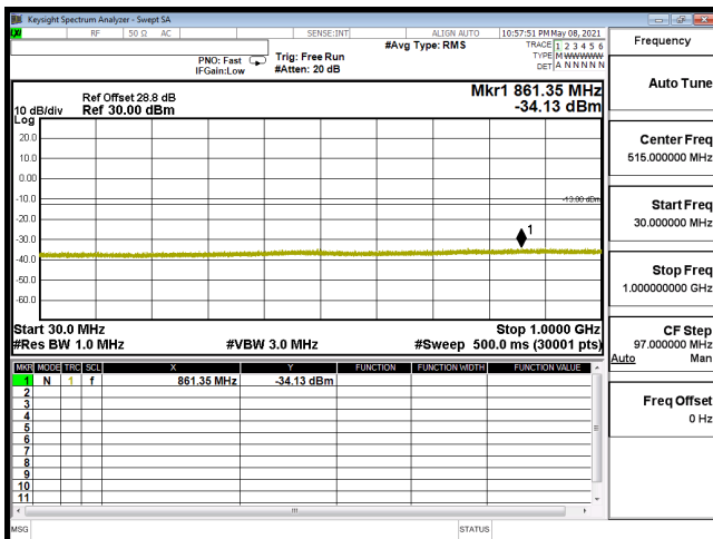
CSE-B66_1.4M-CH131979-16QAM(1,0)-30M-1G
