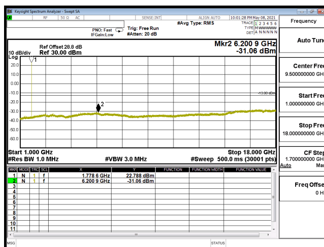
CSE-B66_3M-CH132657-16QAM(1,7)-1G-18G
