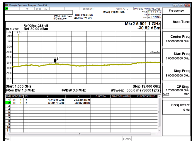
CSE-B66_1.4M-CH131979-64QAM(1,0)-1G-18G
