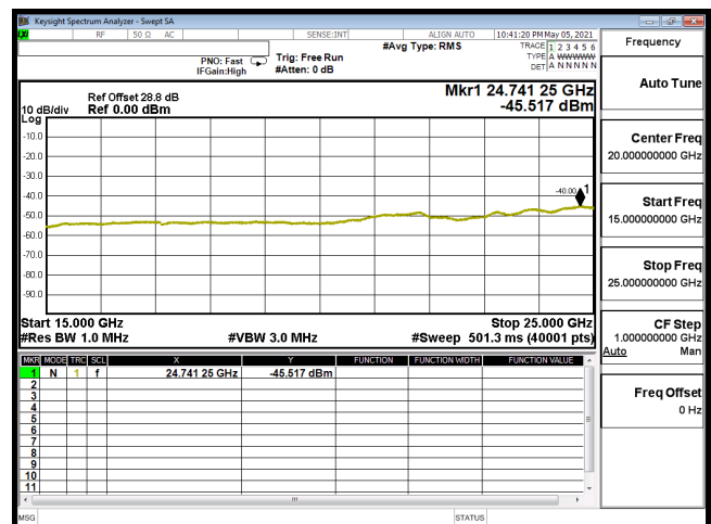
CSE-B30_5M-CH27710-64QAM(1,0)-15G-25G
