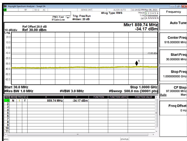
CSE-B66_10M-CH132322-QPSK(1,25)-30M-1G
