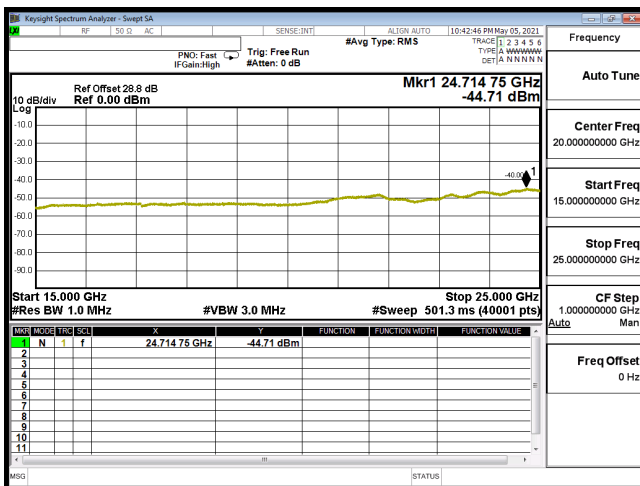
CSE-B30_5M-CH27735-QPSK(1,12)-15G-25G
