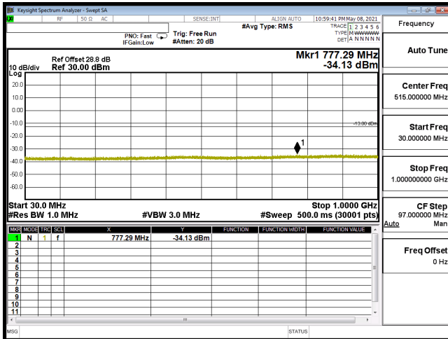
CSE-B66_1.4M-CH132665-QPSK(3,2)-30M-1G
