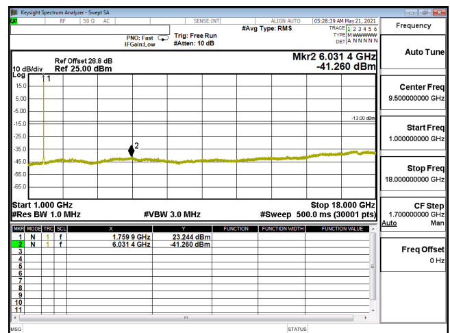
CSE-ENDC_12A_n66_64QAM_40M_CH352000_1760(1,108)-1G-18G
