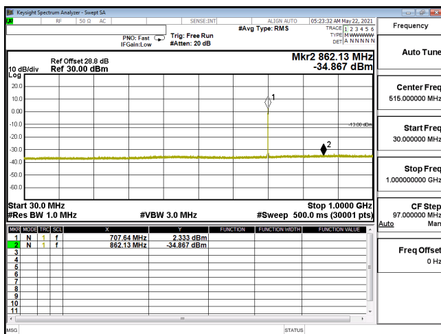
CSE-ENDC_12A_n66_64QAM_40M_CH352000_1760(1,108)-30M-1G
