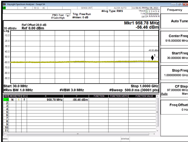
CSE-B30_5M-CH27735-64QAM(1,12)-30M-1G
