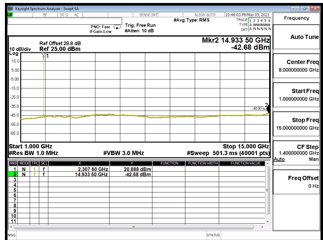
CSE-B30_5M-CH27685-64QAM(1,12)-1G-15G
