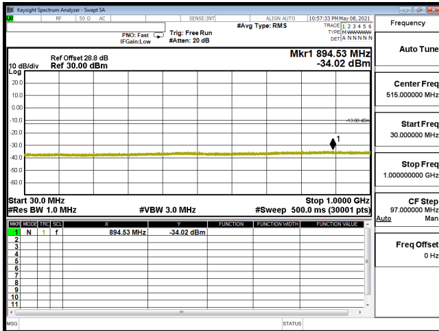
CSE-B66_1.4M-CH131979-QPSK(1,5)-30M-1G
