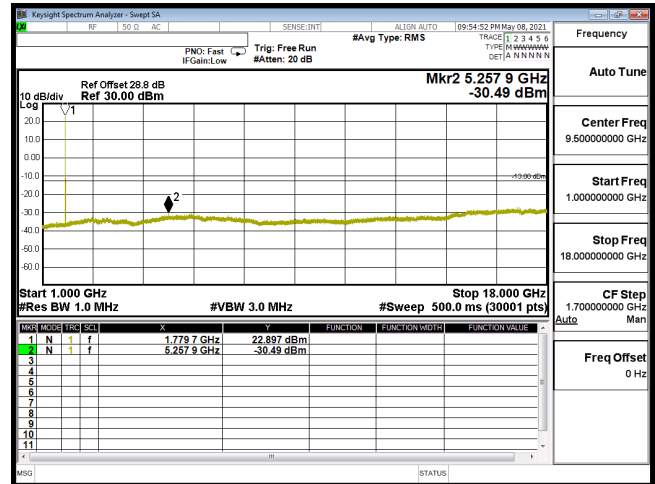
CSE-B66_1.4M-CH132665-QPSK(3,2)-1G-18G
