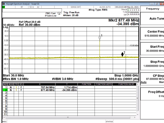
CSE-ENDC_12A_n66_16QAM_40M_CH352000_1760(1,108)-30M-1G
