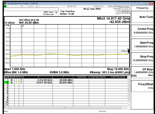
CSE-B30_5M-CH27735-64QAM(1,12)-1G-15G
