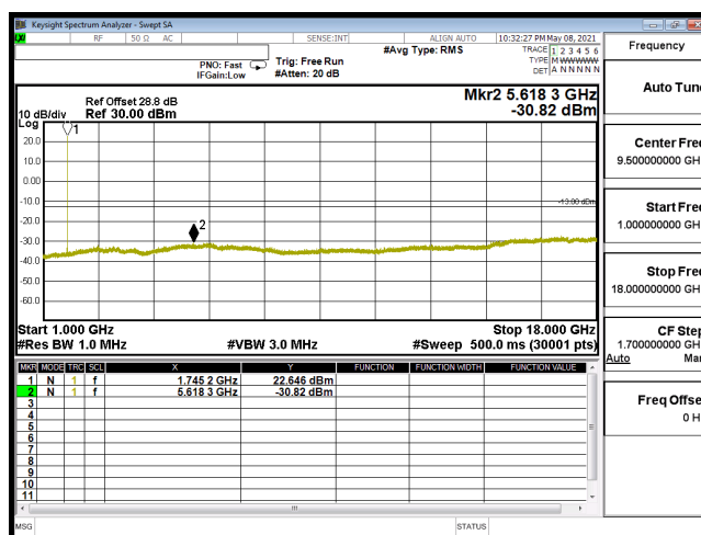
CSE-B66_10M-CH132322-16QAM(1,25)-1G-18G
