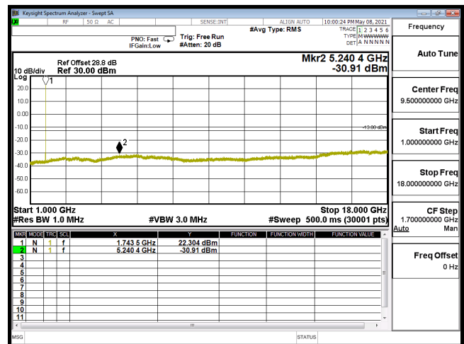
CSE-B66_3M-CH132322-16QAM(1,0)-1G-18G
