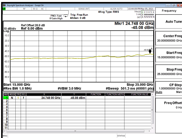
CSE-B30_5M-CH27685-QPSK(1,0)-15G-25G
