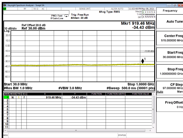
CSE-B66_3M-CH132322-16QAM(1,0)-30M-1G
