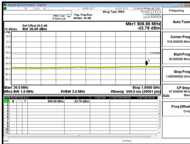
CSE-B66_3M-CH132322-QPSK(1,7)-30M-1G
