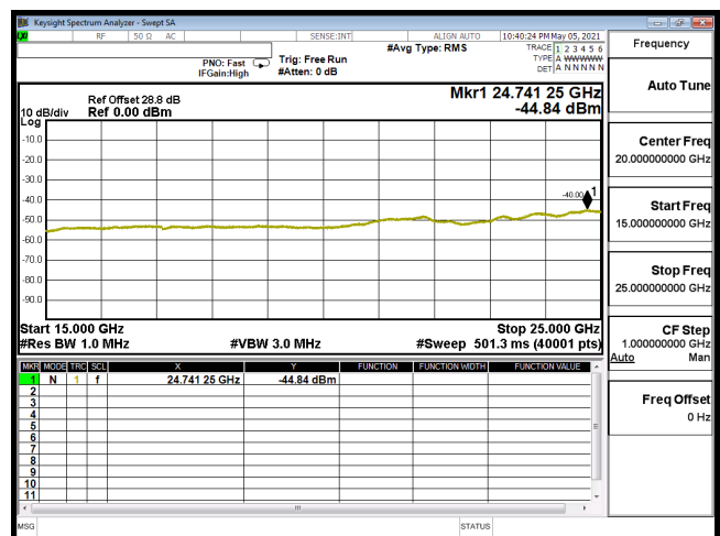
CSE-B30_5M-CH27710-QPSK(1,0)-15G-25G
