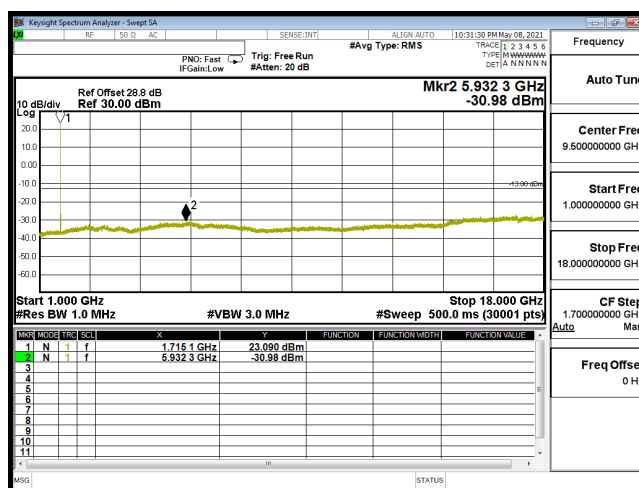
CSE-B66_10M-CH132022-16QAM(1,25)-1G-18G
