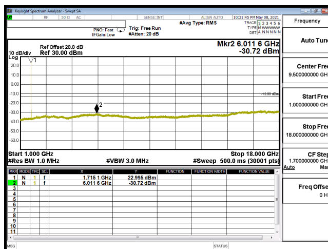
CSE-B66_10M-CH132022-64QAM(1,25)-1G-18G
