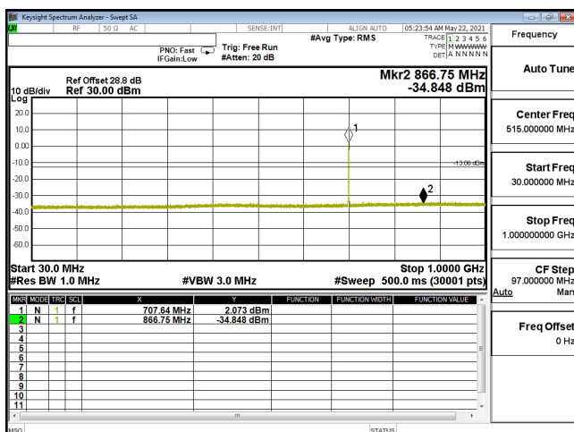
CSE-ENDC_12A_n66_256QAM_40M_CH352000_1760(1,108)-30M-1G
