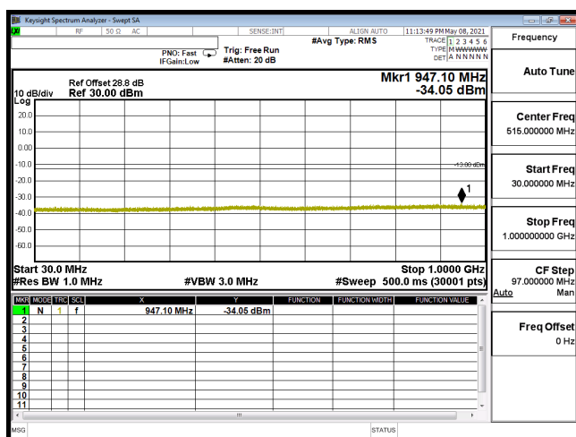
CSE-B66_10M-CH132322-16QAM(1,25)-30M-1G
