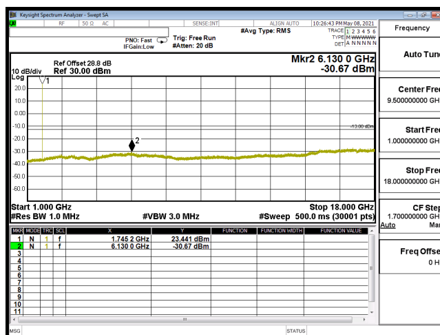
CSE-B66_5M-CH132322-QPSK(1,12)-1G-18G
