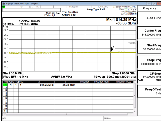
CSE-B30_5M-CH27685-QPSK(1,0)-30M-1G
