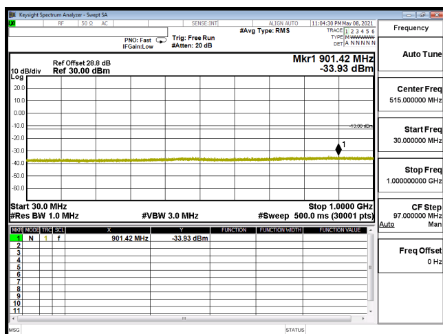
CSE-B66_3M-CH132657-QPSK(1,7)-30M-1G
