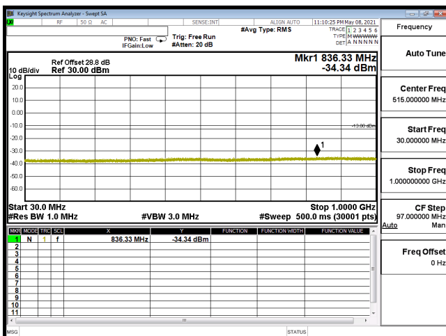
CSE-B66_5M-CH132647-64QAM(1,12)-30M-1G
