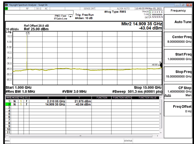
CSE-B30_5M-CH27710-16QAM(1,12)-1G-15G
