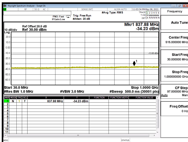
CSE-B66_3M-CH132322-64QAM(1,0)-30M-1G
