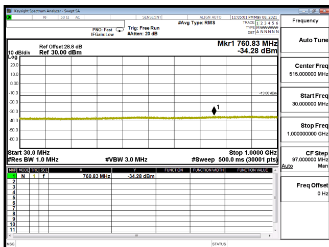
CSE-B66_3M-CH132657-64QAM(1,7)-30M-1G
