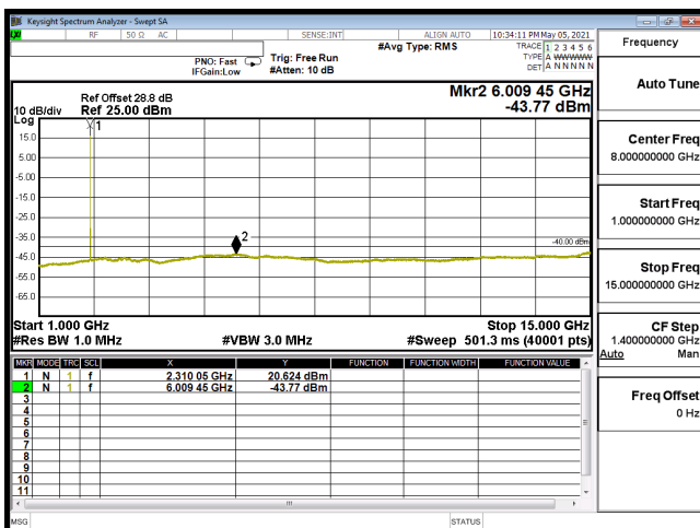
CSE-B30_10M-CH27710-64QAM(1,25)-1G-15G
