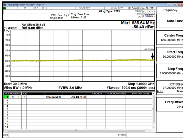
CSE-B30_5M-CH27710-16QAM(1,12)-30M-1G
