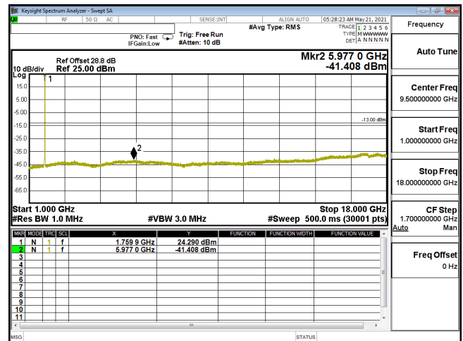
CSE-ENDC_12A_n66_16QAM_40M_CH352000_1760(1,108)-1G-18G
