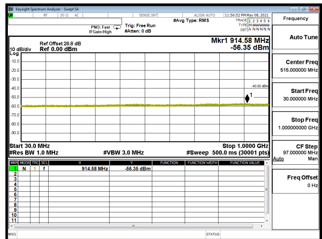
CSE-B30_10M-CH27710-QPSK(1,25)-30M-1G
