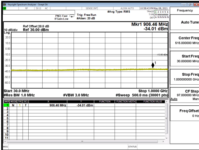
CSE-B66_1.4M-CH132322-QPSK(3,3)-30M-1G
