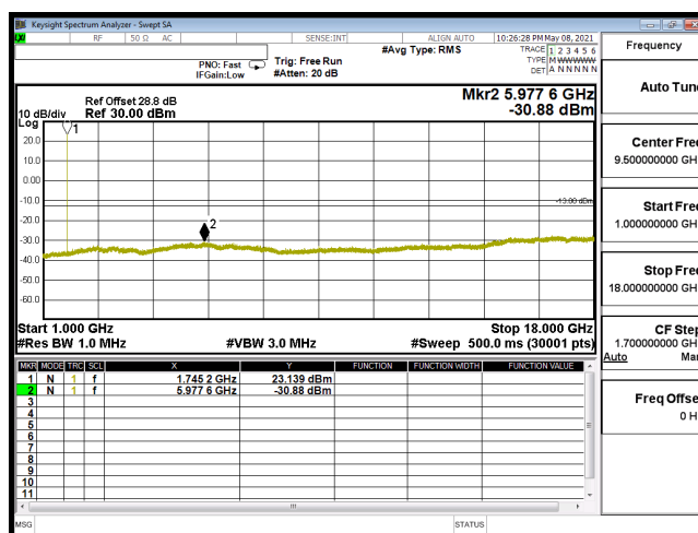
CSE-B66_5M-CH132322-16QAM(1,12)-1G-18G
