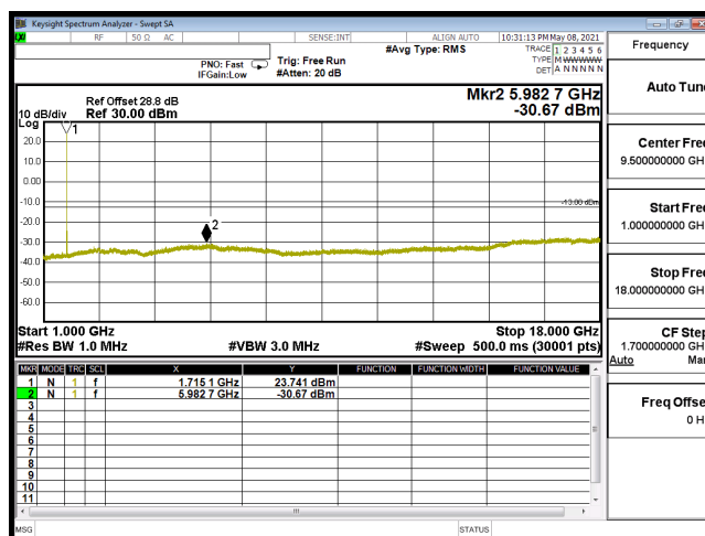
CSE-B66_10M-CH132022-QPSK(1,25)-1G-18G
