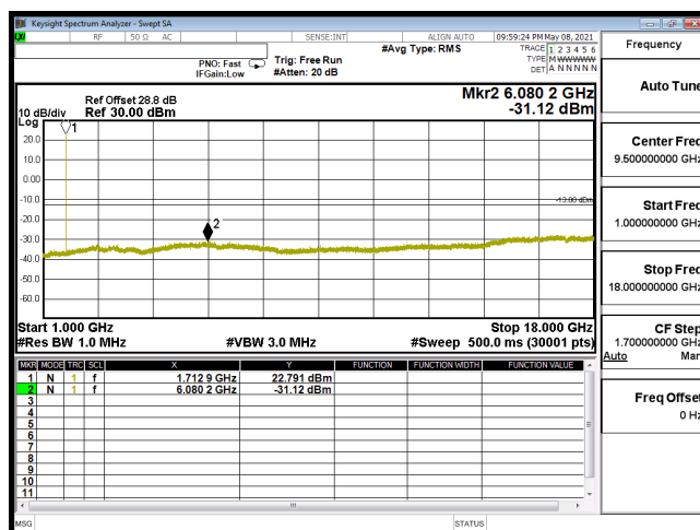
CSE-B66_3M-CH131987-64QAM(1,14)-1G-18G
