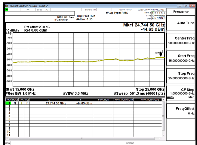
CSE-B30_10M-CH27710-QPSK(1,25)-15G-25G
