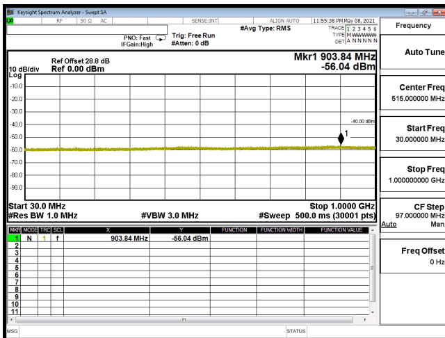
CSE-B30_5M-CH27685-64QAM(1,12)-30M-1G
