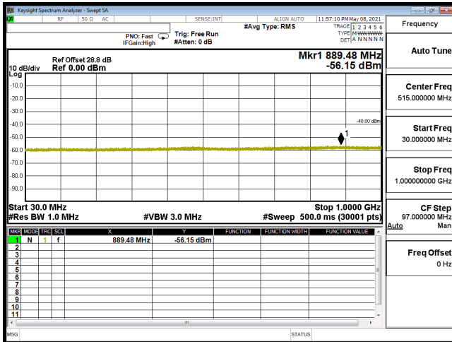
CSE-B30_10M-CH27710-16QAM(1,25)-30M-1G
