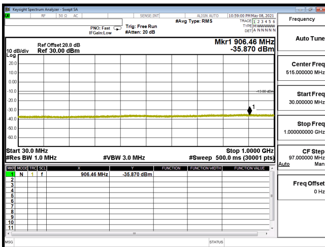
CSE-B66_1.4M-CH132322-16QAM(1,2)-30M-1G
