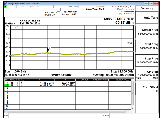
CSE-B66_1.4M-CH132322-QPSK(3,3)-1G-18G
