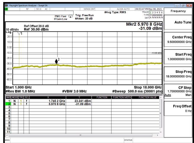
CSE-B66_1.4M-CH132322-16QAM(1,2)-1G-18G
