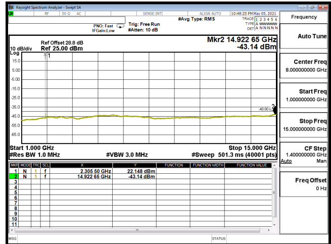
CSE-B30_5M-CH27685-QPSK(1,0)-1G-15G
