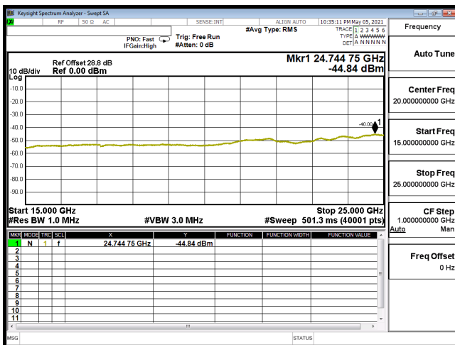
CSE-B30_10M-CH27710-16QAM(1,25)-15G-25G
