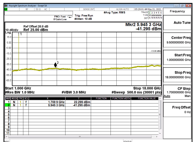
CSE-ENDC_12A_n66_256QAM_40M_CH352000_1760(1,108)-1G-18G
