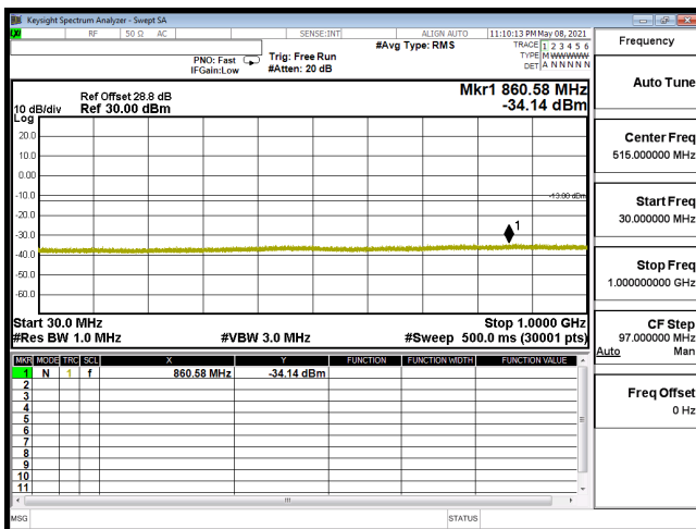
CSE-B66_5M-CH132647-16QAM(1,0)-30M-1G
