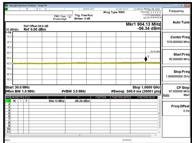
CSE-B30_5M-CH27735-16QAM(1,0)-30M-1G
