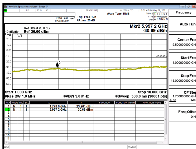
CSE-B66_3M-CH132657-64QAM(1,7)-1G-18G
