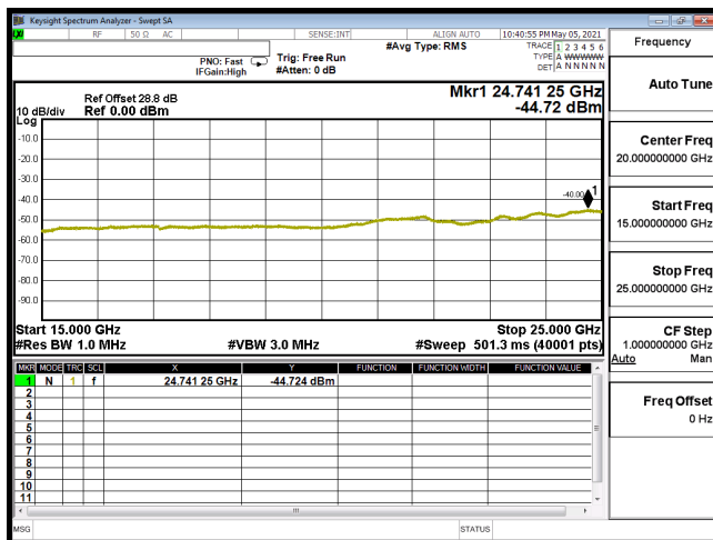
CSE-B30_5M-CH27710-16QAM(1,12)-15G-25G
