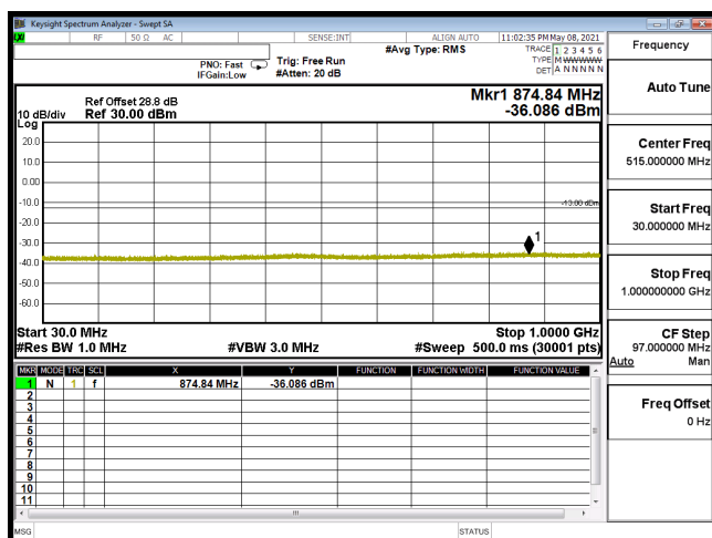
CSE-B66_3M-CH131987-QPSK(1,7)-30M-1G
