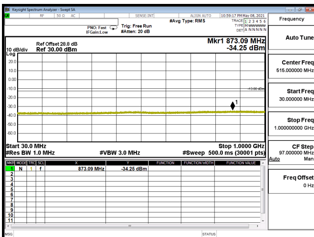
CSE-B66_1.4M-CH132322-64QAM(1,0)-30M-1G
