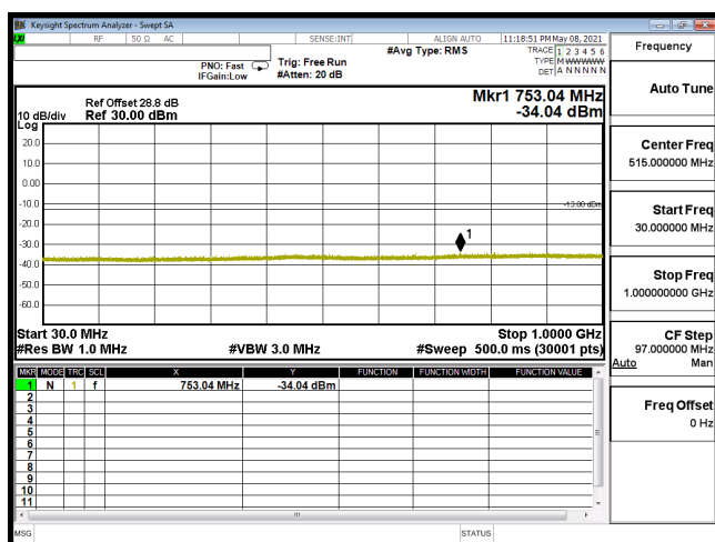
CSE-B66_15M-CH132597-16QAM(1,37)-30M-1G
