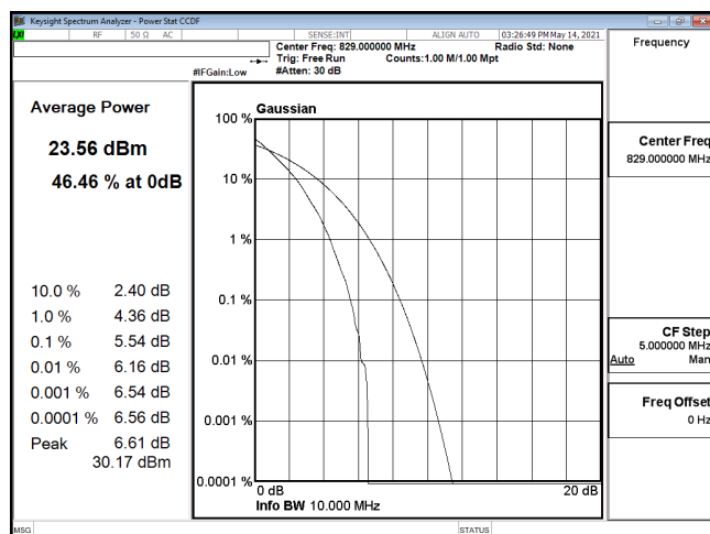
PTAR-ENDC_30A_n5-QPSK_10M_CH165800_829(50,0)
