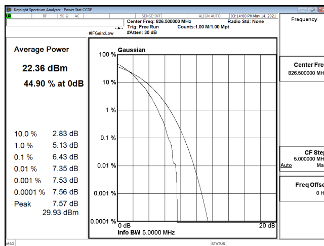
PTAR-ENDC_30A_n5-64QAM_5M_CH165300_826.5(25,0)
