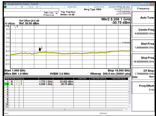
CSE-B66_20M-CH132572-QPSK(1,50)-1G-18G
