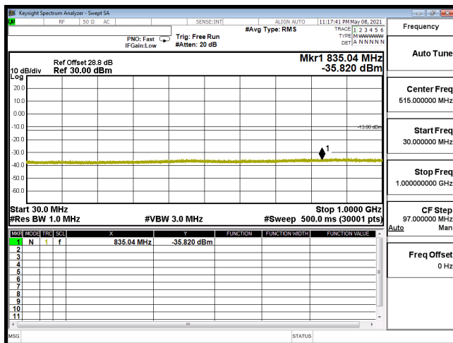
CSE-B66_15M-CH132322-16QAM(1,37)-30M-1G
