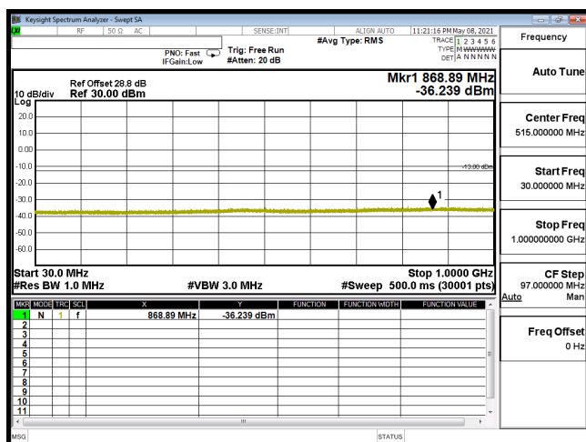
CSE-B66_20M-CH132072-QPSK(1,50)-30M-1G
