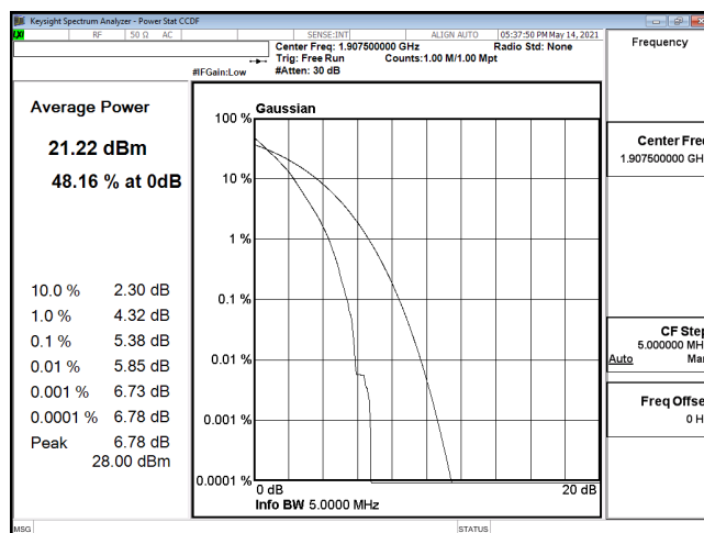
PTAR-ENDC_5A_n2-QPSK_5M_CH381500_1907.5(25,0)
