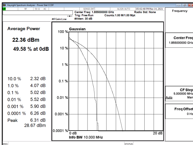
PTAR-ENDC_5A_n2-QPSK_10M_CH371000_1855(50,0)
