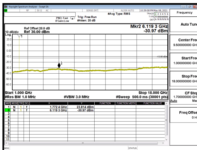
CSE-B66_15M-CH132597-64QAM(1,37)-1G-18G
