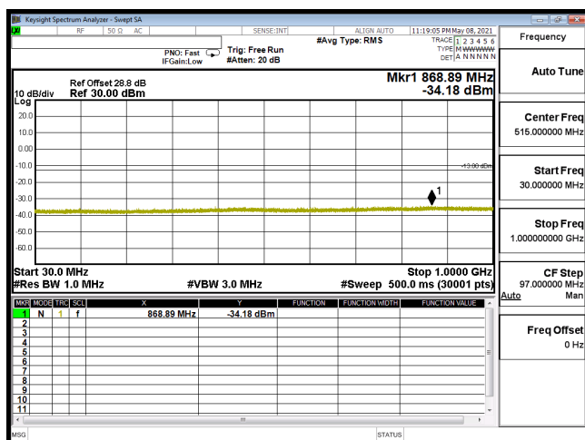
CSE-B66_15M-CH132597-64QAM(1,37)-30M-1G
