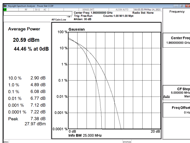
PTAR-ENDC_5A_n2-64QAM_20M_CH372000_1860(100,0)
