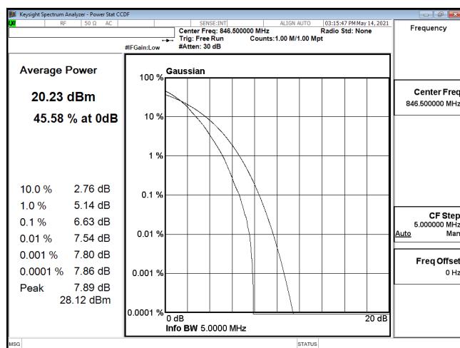
PTAR-ENDC_30A_n5-256QAM_5M_CH169300_846.5(25,0)
