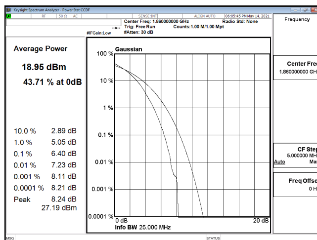
PTAR-ENDC_5A_n2-256QAM_20M_CH372000_1860(100,0)
