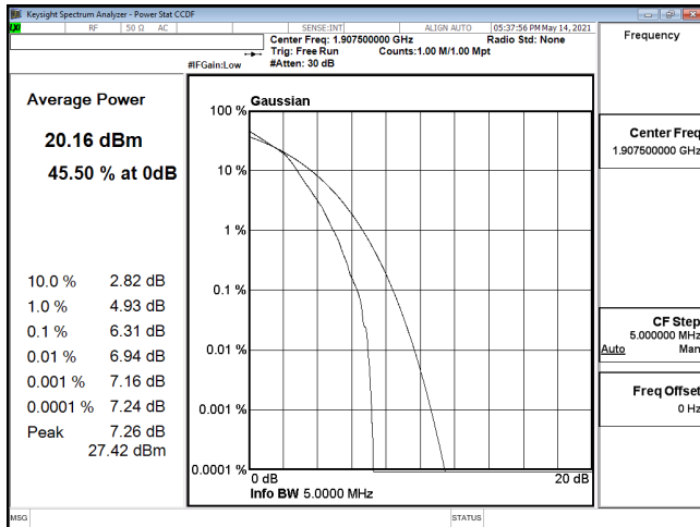
PTAR-ENDC_5A_n2-16QAM_5M_CH381500_1907.5(25,0)
