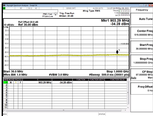
CSE-B66_20M-CH132072-16QAM(1,50)-30M-1G
