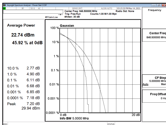
PTAR-ENDC_30A_n5-16QAM_5M_CH169300_846.5(25,0)
