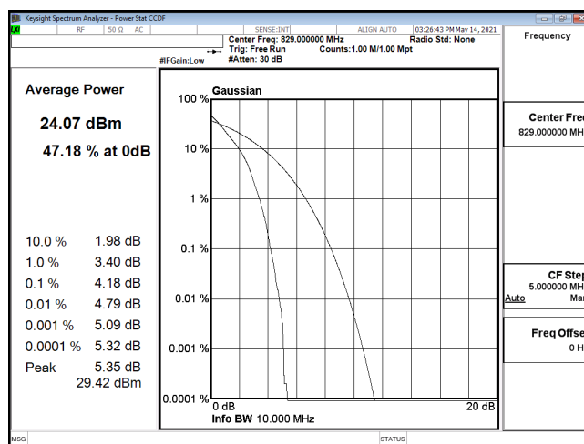
PTAR-ENDC_30A_n5-PI2-BPSK_10M_CH165800_829(50,0)
