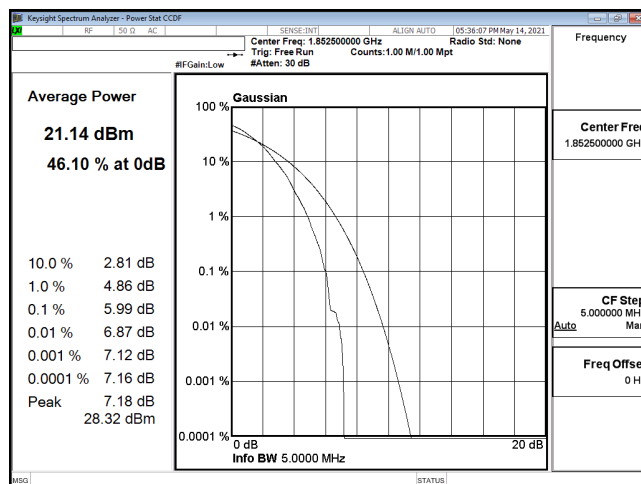
PTAR-ENDC_5A_n2-64QAM_5M_CH370500_1852.5(25,0)
