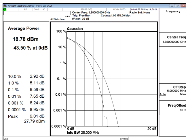
PTAR-ENDC_5A_n2-256QAM_20M_CH376000_1880(100,0)
