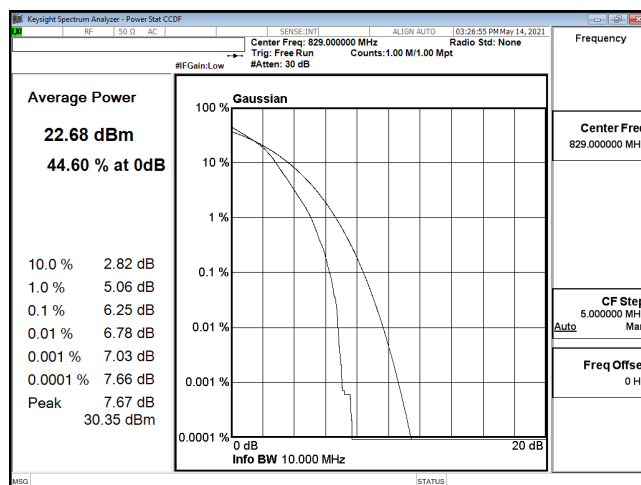
PTAR-ENDC_30A_n5-16QAM_10M_CH165800_829(50,0)
