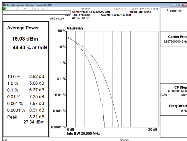
PTAR-ENDC_5A_n2-256QAM_15M_CH371500_1857.5(75,0)
