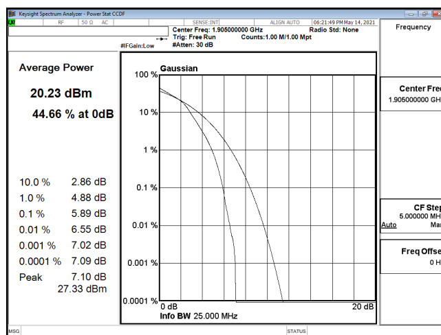
PTAR-ENDC_5A_n2-16QAM_10M_CH381000_1905(50,0)
