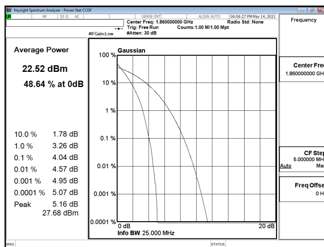
PTAR-ENDC_5A_n2-PI2-BPSK_20M_CH372000_1860(100,0)
