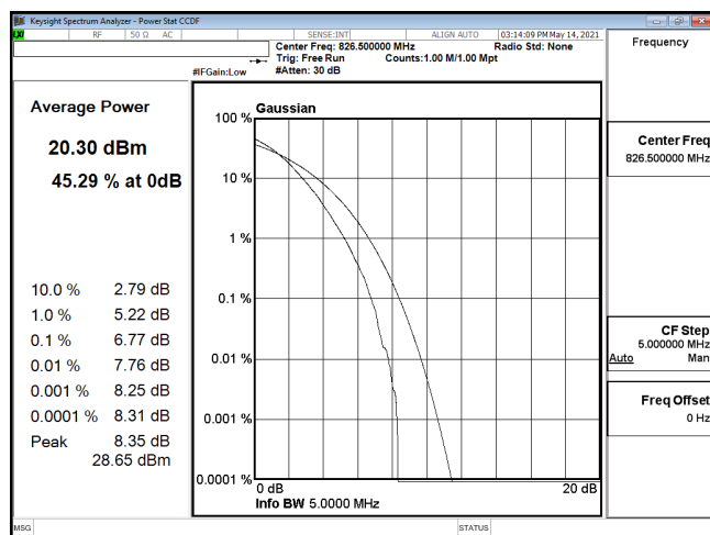
PTAR-ENDC_30A_n5-256QAM_5M_CH165300_826.5(25,0)
