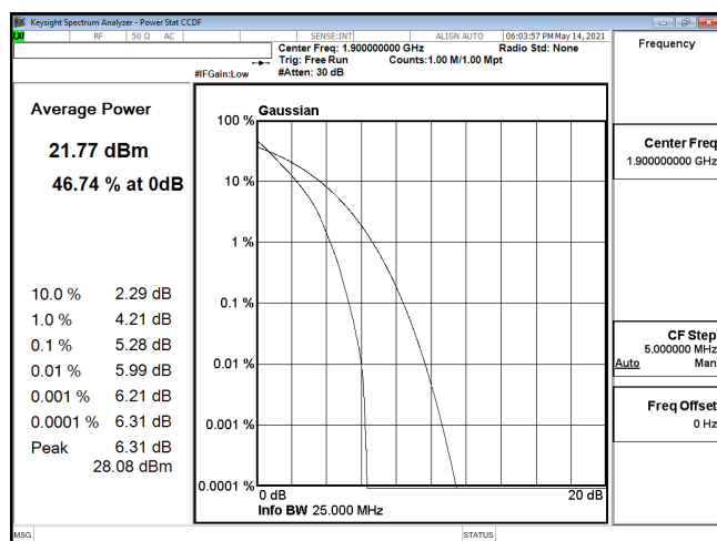
PTAR-ENDC_5A_n2-QPSK_20M_CH380000_1900(100,0)
