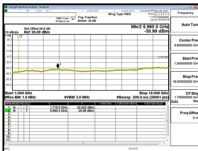
CSE-B66_15M-CH132047-16QAM(1,37)-1G-18G
