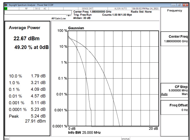
PTAR-ENDC_5A_n2-PI2-BPSK_15M_CH376000_1880(75,0)
