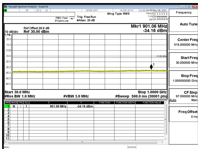
CSE-B66_20M-CH132072-64QAM(1,50)-30M-1G
