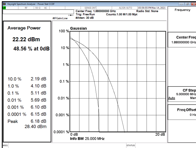
PTAR-ENDC_5A_n2-QPSK_15M_CH376000_1880(75,0)
