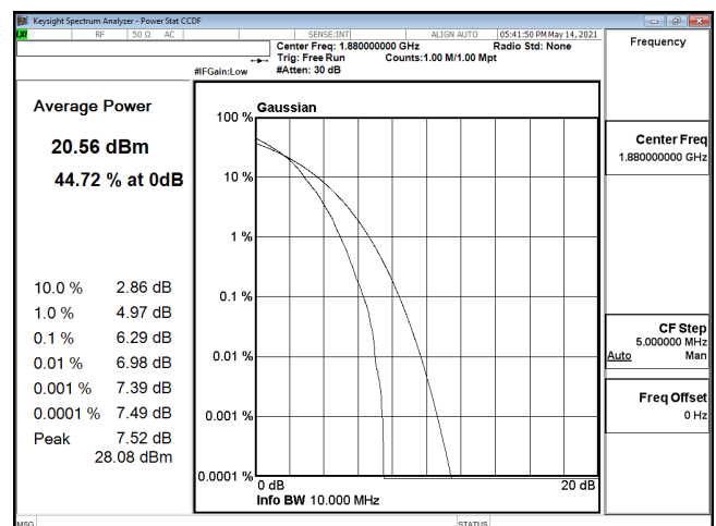
PTAR-ENDC_5A_n2-64QAM_10M_CH376000_1880(50,0)
