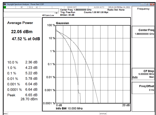
PTAR-ENDC_5A_n2-QPSK_10M_CH376000_1880(50,0)
