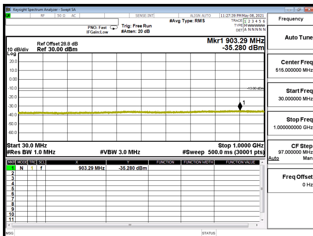
CSE-B66_20M-CH132572-64QAM(1,50)-30M-1G
