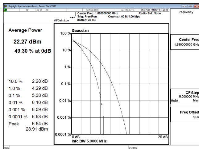
PTAR-ENDC_5A_n2-QPSK_5M_CH376000_1880(25,0)
