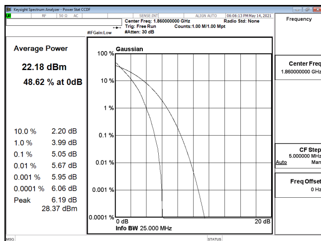
PTAR-ENDC_5A_n2-QPSK_20M_CH372000_1860(100,0)
