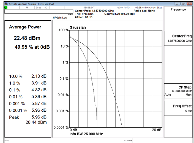
PTAR-ENDC_5A_n2-QPSK_15M_CH371500_1857.5(75,0)
