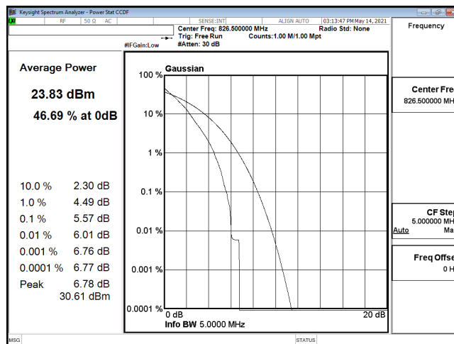
PTAR-ENDC_30A_n5-QPSK_5M_CH165300_826.5(25,0)
