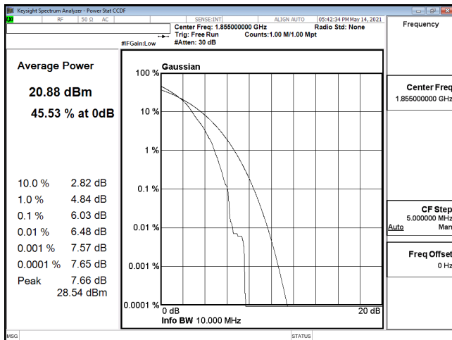
PTAR-ENDC_5A_n2-64QAM_10M_CH371000_1855(50,0)
