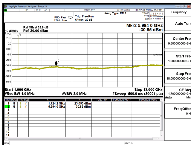
CSE-B66_15M-CH132047-64QAM(1,74)-1G-18G
