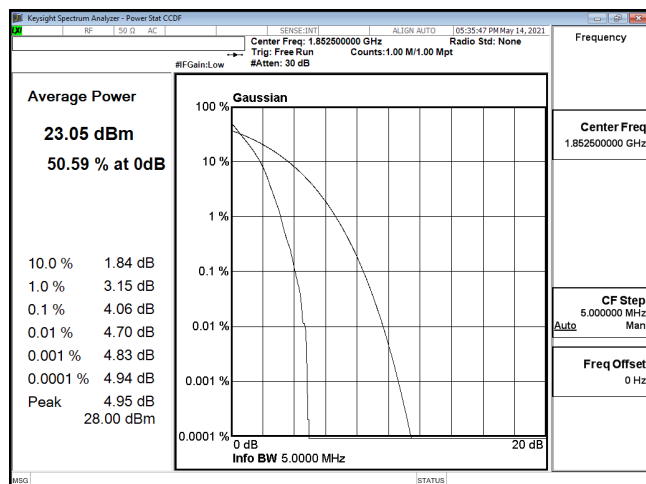
PTAR-ENDC_5A_n2-PI2-BPSK_5M_CH370500_1852.5(25,0)
