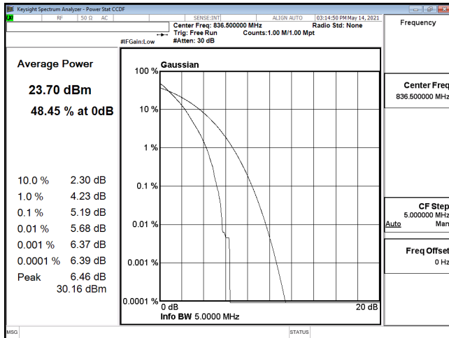
PTAR-ENDC_30A_n5-QPSK_5M_CH167300_836.5(25,0)
