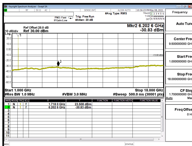
CSE-B66_15M-CH132047-QPSK(1,37)-1G-18G
