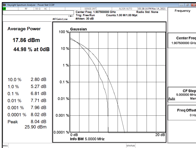
PTAR-ENDC_5A_n2-256QAM_5M_CH381500_1907.5(25,0)
