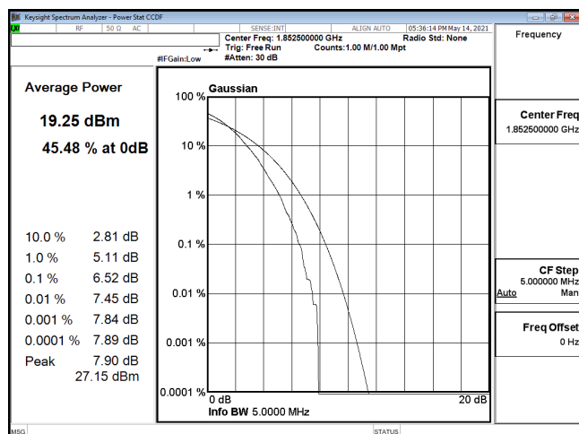
PTAR-ENDC_5A_n2-256QAM_5M_CH370500_1852.5(25,0)
