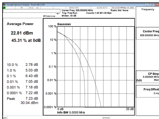
PTAR-ENDC_30A_n5-16QAM_5M_CH165300_826.5(25,0)
