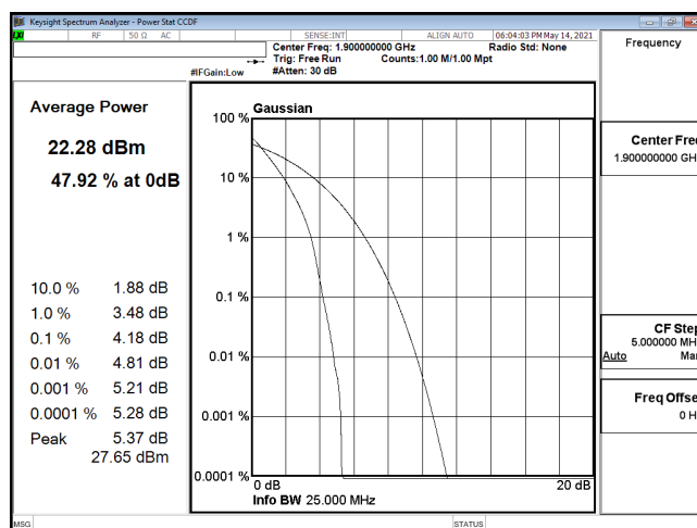
PTAR-ENDC_5A_n2-PI2-BPSK_20M_CH380000_1900(100,0)
