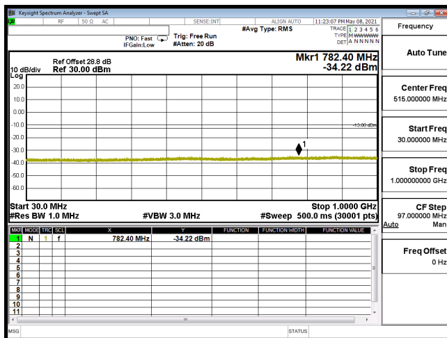
CSE-B66_20M-CH132572-16QAM(1,50)-30M-1G
