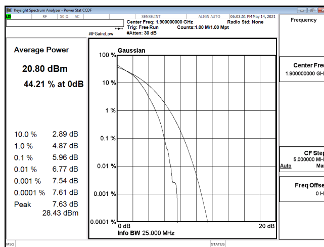
PTAR-ENDC_5A_n2-16QAM_20M_CH380000_1900(100,0)
