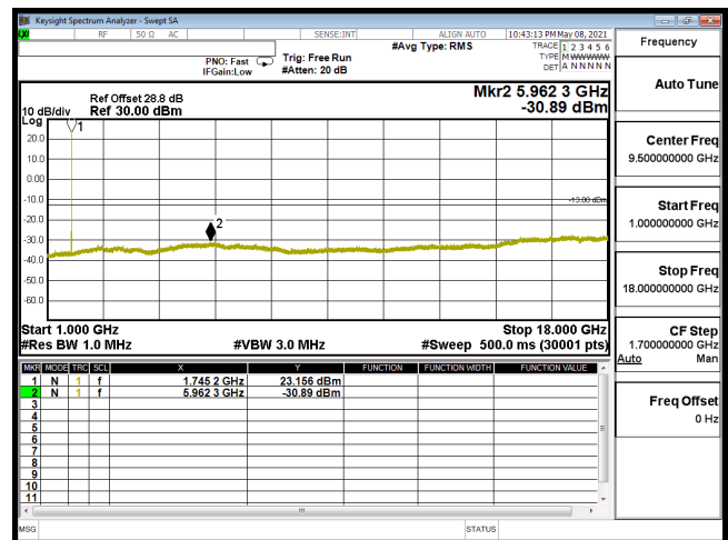
CSE-B66_20M-CH132322-16QAM(1,50)-1G-18G
