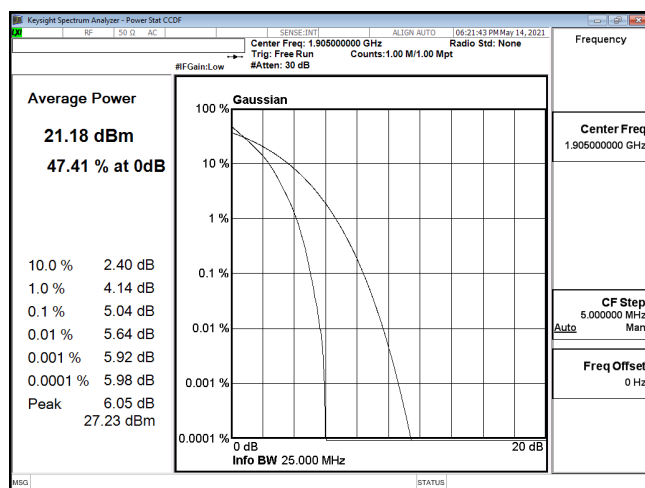
PTAR-ENDC_5A_n2-QPSK_10M_CH381000_1905(50,0)
