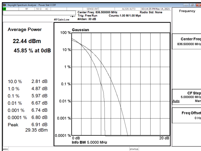
PTAR-ENDC_30A_n5-64QAM_5M_CH167300_836.5(25,0)
