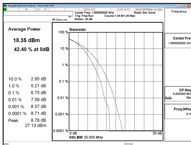
PTAR-ENDC_5A_n2-256QAM_20M_CH380000_1900(100,0)
