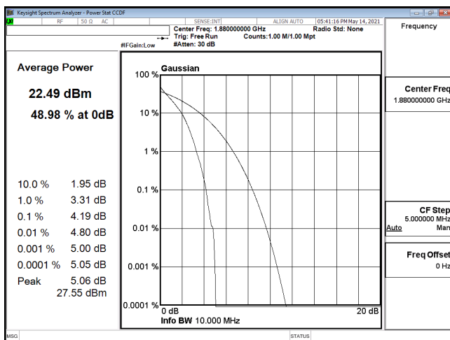
PTAR-ENDC_5A_n2-PI2-BPSK_10M_CH376000_1880(50,0)
