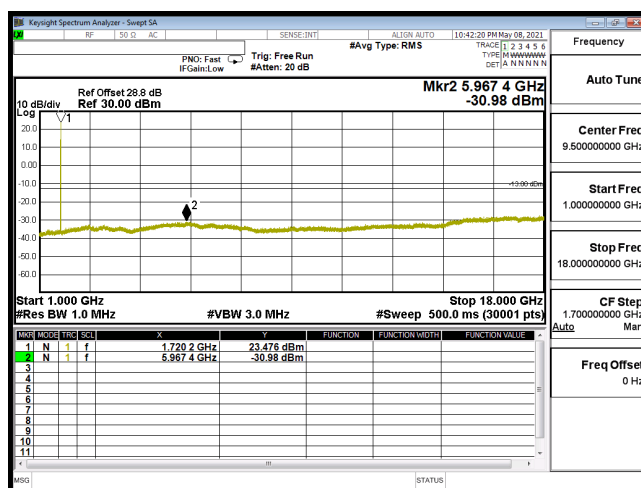
CSE-B66_20M-CH132072-16QAM(1,50)-1G-18G
