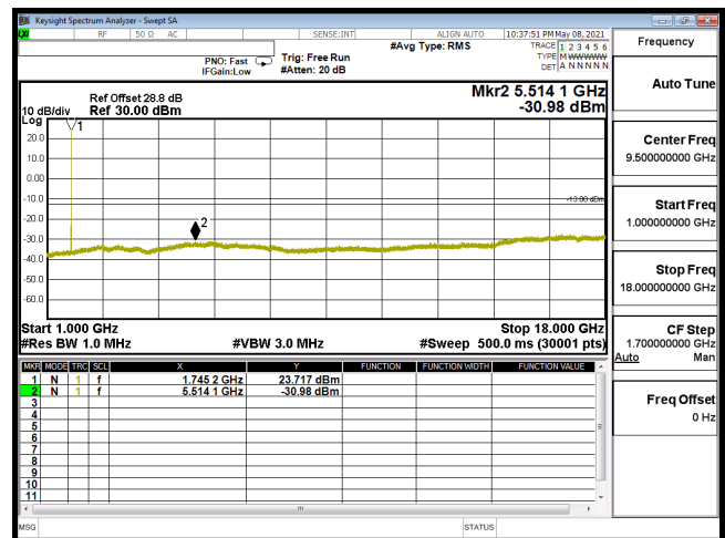
CSE-B66_15M-CH132322-16QAM(1,37)-1G-18G
