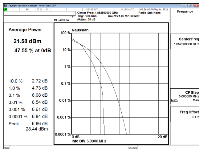
PTAR-ENDC_5A_n2-16QAM_5M_CH370500_1852.5(25,0)
