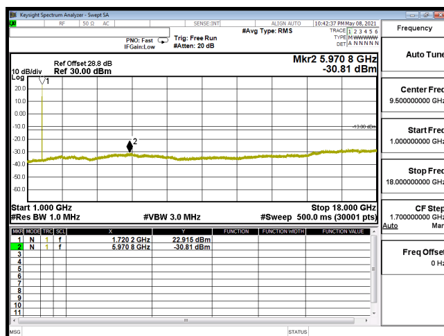
CSE-B66_20M-CH132072-64QAM(1,50)-1G-18G
