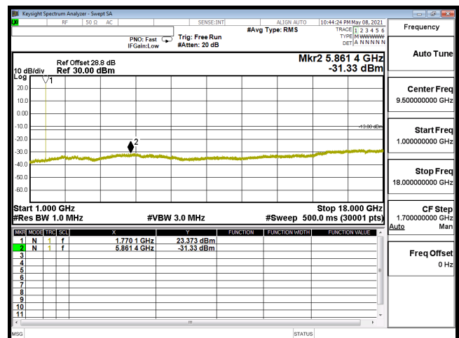
CSE-B66_20M-CH132572-64QAM(1,50)-1G-18G
