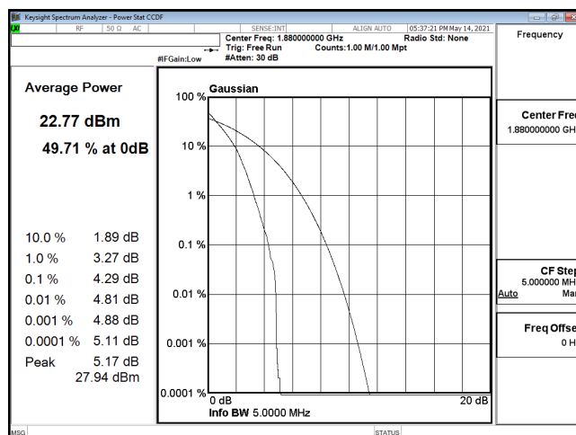
PTAR-ENDC_5A_n2-PI2-BPSK_5M_CH376000_1880(25,0)
