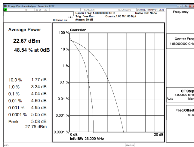
PTAR-ENDC_5A_n2-PI2-BPSK_20M_CH376000_1880(100,0)
