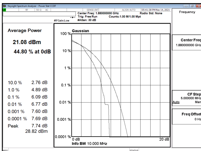
PTAR-ENDC_5A_n2-16QAM_10M_CH376000_1880(50,0)
