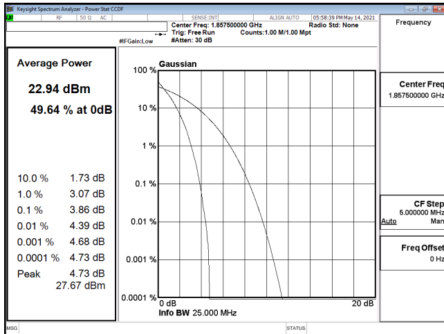
PTAR-ENDC_5A_n2-PI2-BPSK_15M_CH371500_1857.5(75,0)
