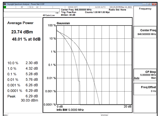
PTAR-ENDC_30A_n5-QPSK_5M_CH169300_846.5(25,0)
