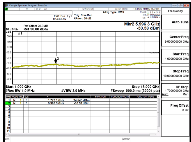
CSE-B66_20M-CH132572-16QAM(1,50)-1G-18G
