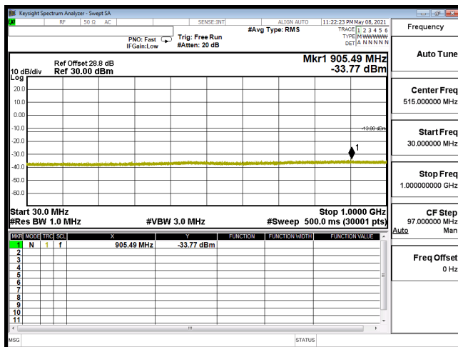
CSE-B66_20M-CH132322-16QAM(1,50)-30M-1G
