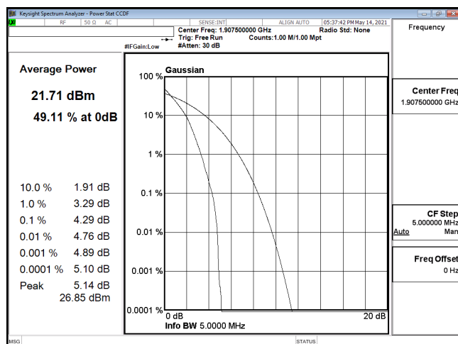
PTAR-ENDC_5A_n2-PI2-BPSK_5M_CH381500_1907.5(25,0)
