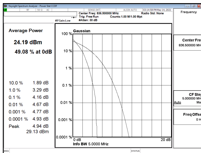
PTAR-ENDC_30A_n5-PI2-BPSK_5M_CH167300_836.5(25,0)
