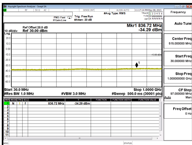
CSE-B66_15M-CH132047-64QAM(1,74)-30M-1G
