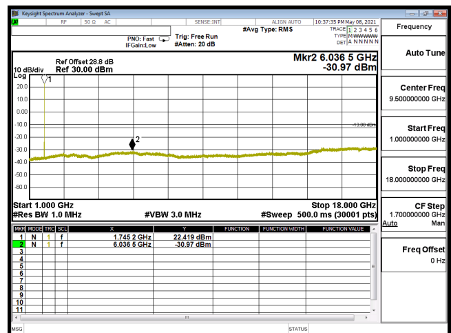
CSE-B66_15M-CH132322-64QAM(1,37)-1G-18G
