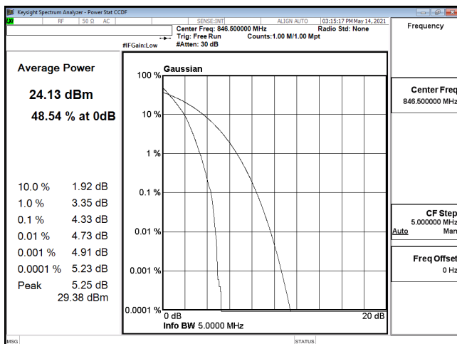
PTAR-ENDC_30A_n5-PI2-BPSK_5M_CH169300_846.5(25,0)
