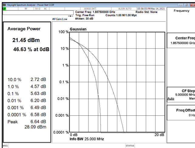
PTAR-ENDC_5A_n2-16QAM_15M_CH371500_1857.5(75,0)
