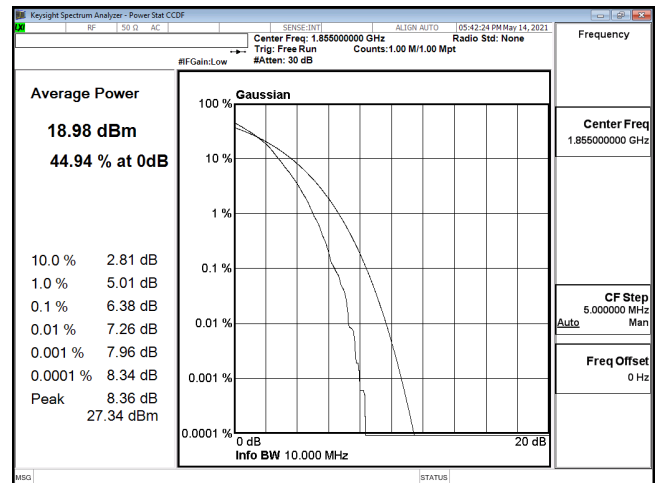
PTAR-ENDC_5A_n2-256QAM_10M_CH371000_1855(50,0)
