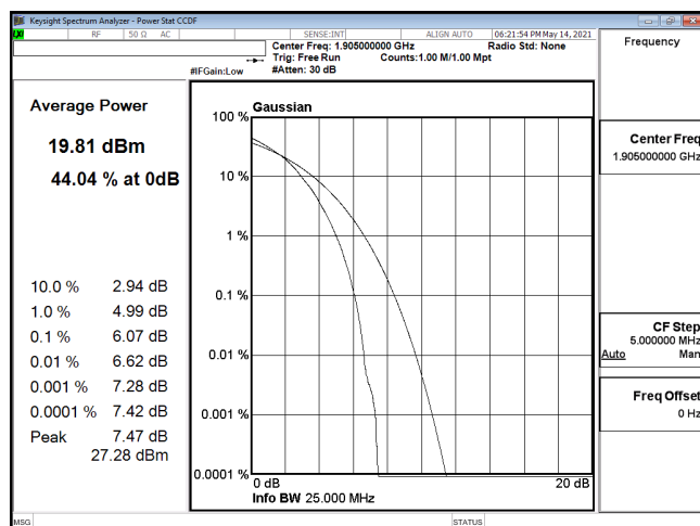
PTAR-ENDC_5A_n2-64QAM_10M_CH381000_1905(50,0)
