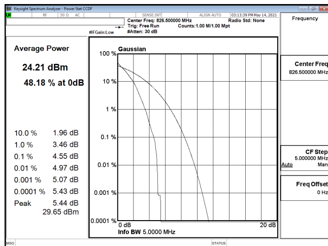
PTAR-ENDC_30A_n5-PI2-BPSK_5M_CH165300_826.5(25,0)
