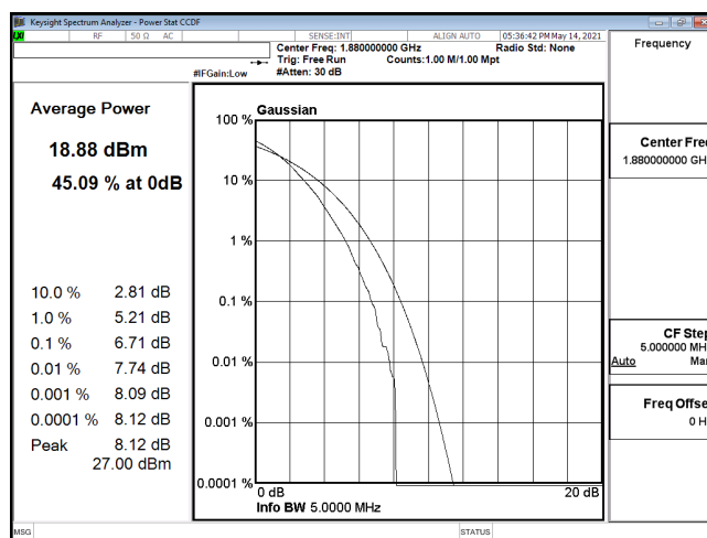
PTAR-ENDC_5A_n2-256QAM_5M_CH376000_1880(25,0)
