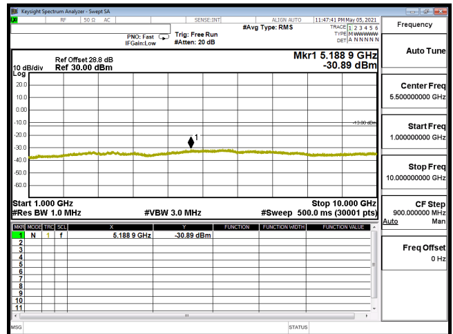
CSE-B14_5M-CH23330-QPSK(1,12)-1G-10G
