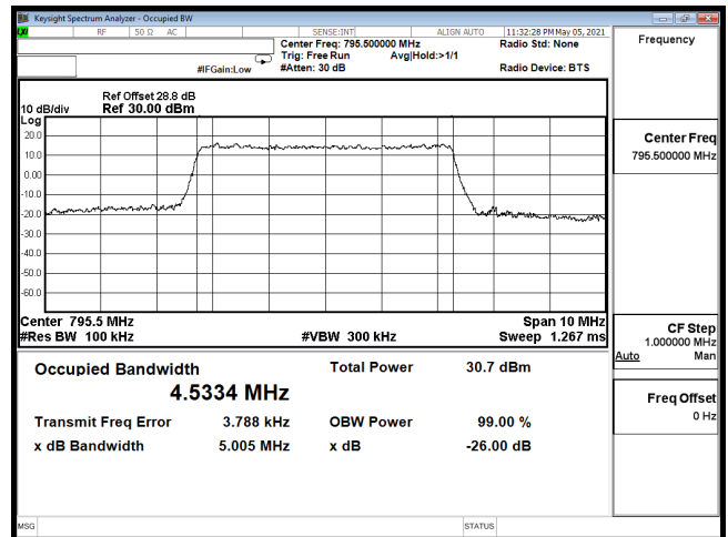
OCC-B14_5M-CH23355-16QAM
