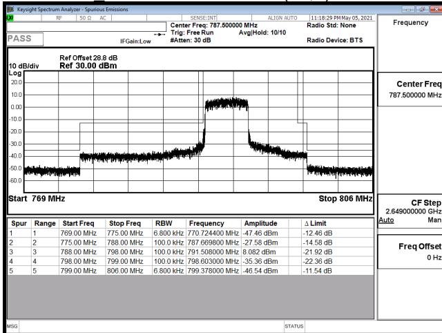
EDGE-B14_5M-CH23305-64QAM(25,0)
