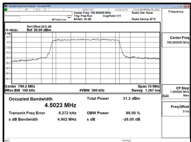
OCC-B14_5M-CH23305-QPSK
