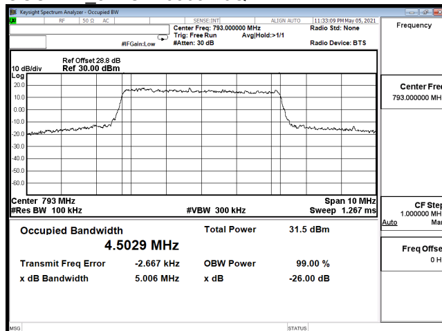
OCC-B14_5M-CH23330-QPSK
