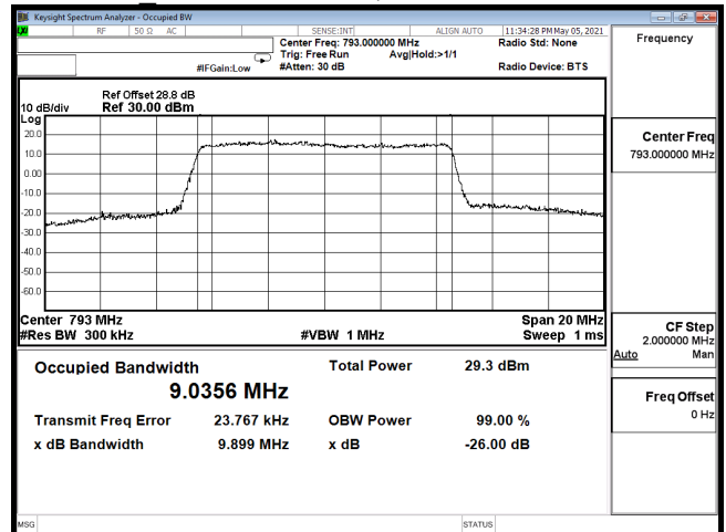
OCC-B14_10M-CH23330-64QAM
