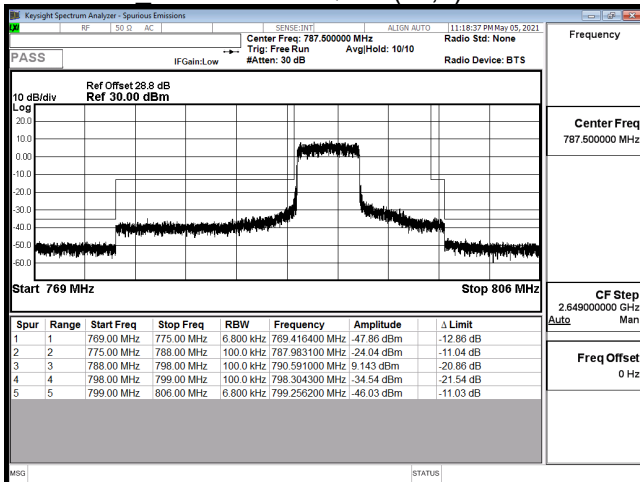
EDGE-B14 5M-CH23305-16QAM(25,0)
