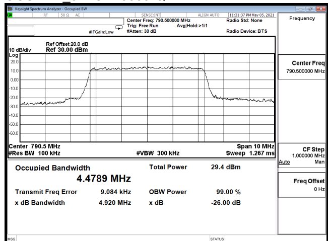
OCC-B14_5M-CH23305-64QAM
