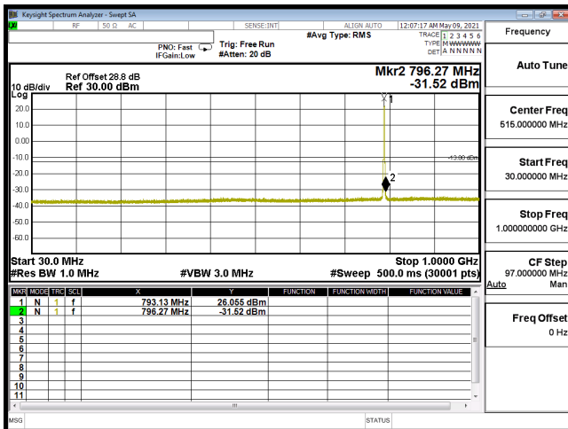
CSE-B14_5M-CH23330-QPSK(1,12)-30M-1G
