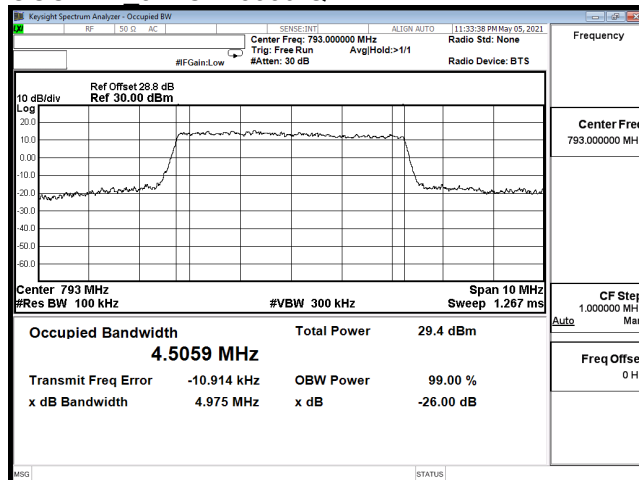
OCC-B14_5M-CH23330-64QAM
