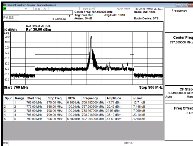
EDGE-B14 10M-CH23330-QPSK(1,0)
