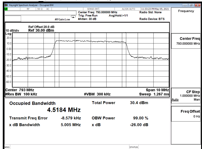
OCC-B14_5M-CH23330-16QAM
