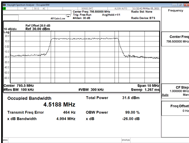
OCC-B14_5M-CH23355-QPSK
