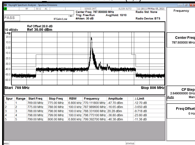
EDGE-B14_5M-CH23305-64QAM(1,0)
