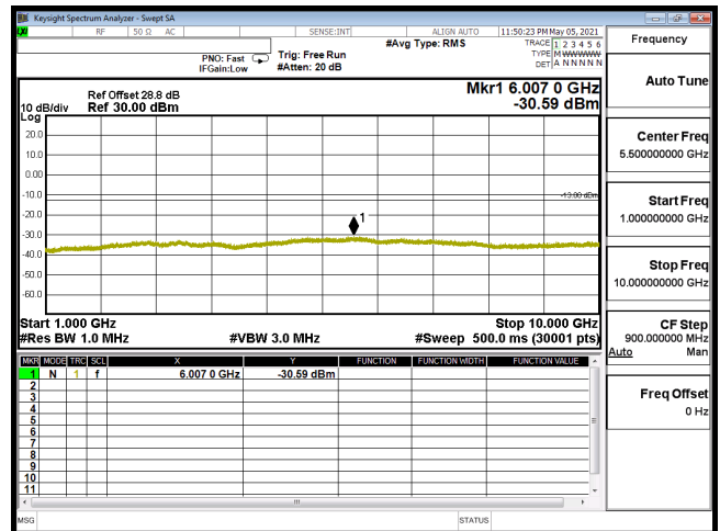
CSE-B14_10M-CH23355-QPSK(1,25)-1G-10G
