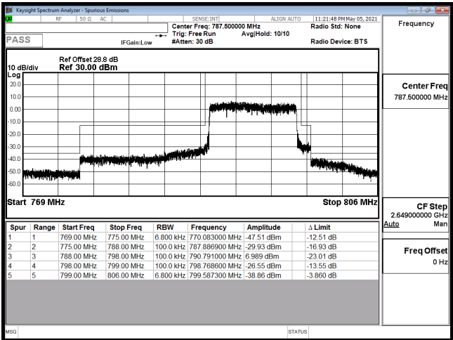
EDGE-B14_10M-CH23330-16QAM(50,0)
