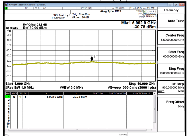
CSE-B14 5M-CH23305-64QAM(1,0)-1G-10G
