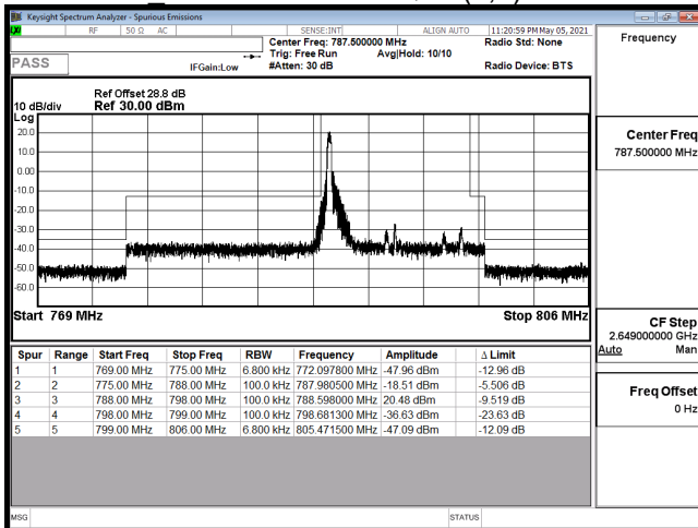
EDGE-B14_10M-CH23330-64QAM(1,0)
