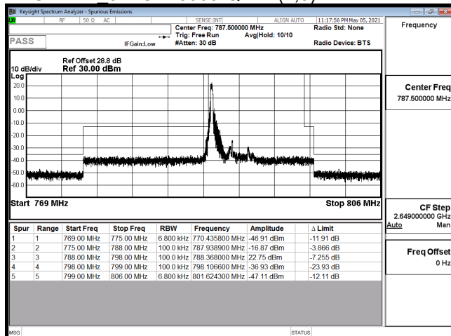
EDGE-B14 5M-CH23305-16QAM(1,0)
