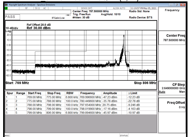
EDGE-B14_5M-CH23355-64QAM(1,24)
