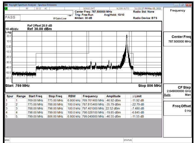
EDGE-B14 10M-CH23330-QPSK(1,49)
