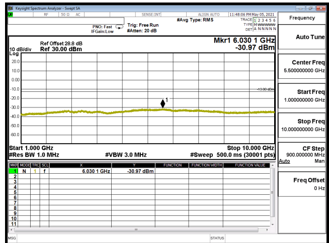
CSE-B14_5M-CH23355-QPSK(1,12)-1G-10G
