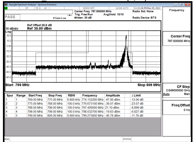
EDGE-B14_10M-CH23330-64QAM(1,49)
