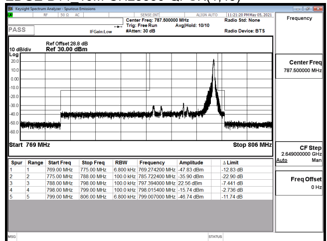
EDGE-B14 10M-CH23330-16QAM(1,49)
