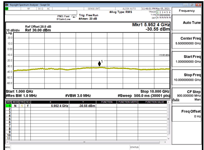
CSE-B14 5M-CH23305-QPSK(1,12)-1G-10G
