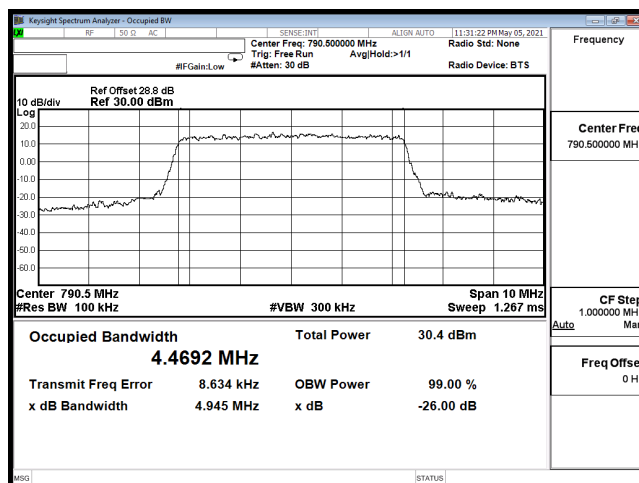
OCC-B14_5M-CH23305-16QAM
