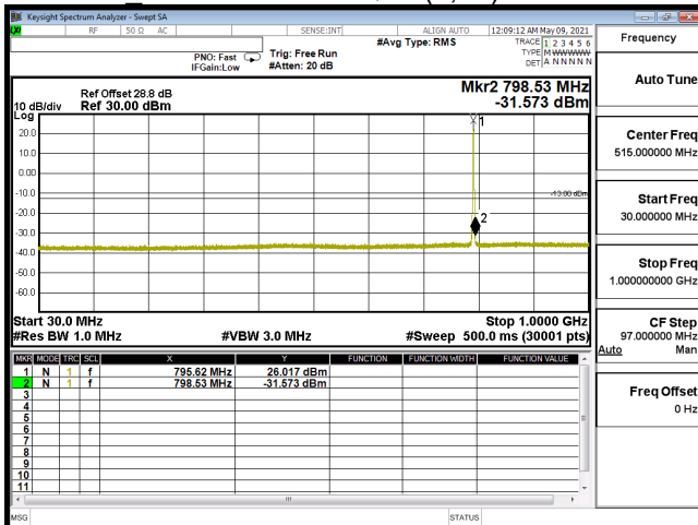
CSE-B14_5M-CH23355-64QAM(1,12)-30M-1G
