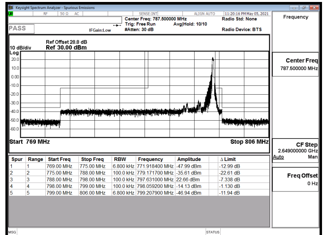
EDGE-B14 5M-CH23355-QPSK(1,24)
