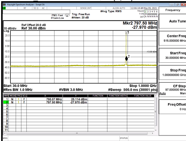
CSE-B14_5M-CH23330-64QAM(1,24)-30M-1G
