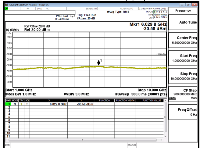
CSE-B14_10M-CH23355-64QAM(1,25)-1G-10G
