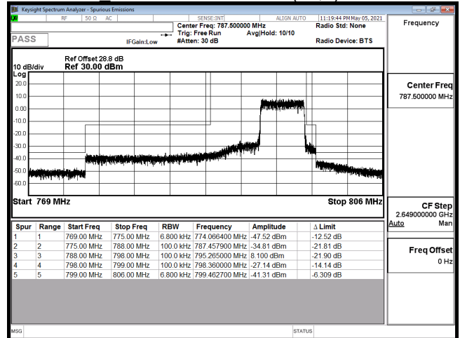
EDGE-B14_5M-CH23355-64QAM(25,0)
