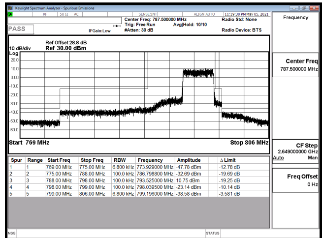
EDGE-B14 5M-CH23355-QPSK(25,0)
