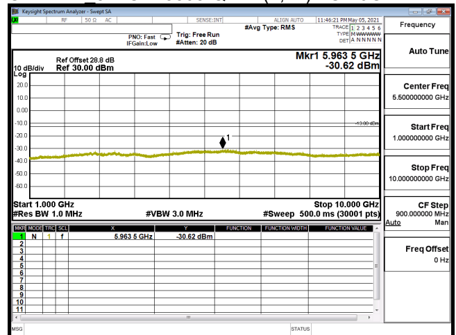
CSE-B14 5M-CH23305-16QAM(1,0)-1G-10G
