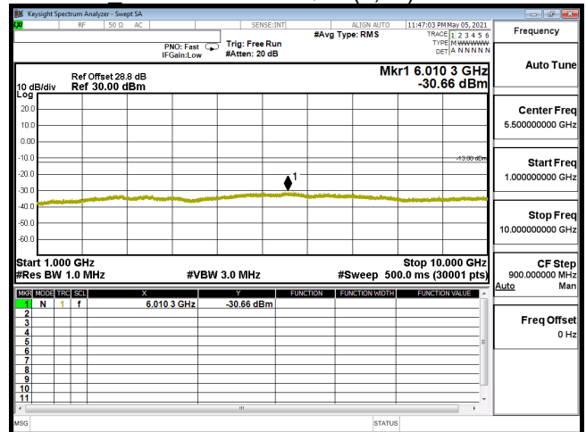
CSE-B14_5M-CH23330-64QAM(1,24)-1G-10G
