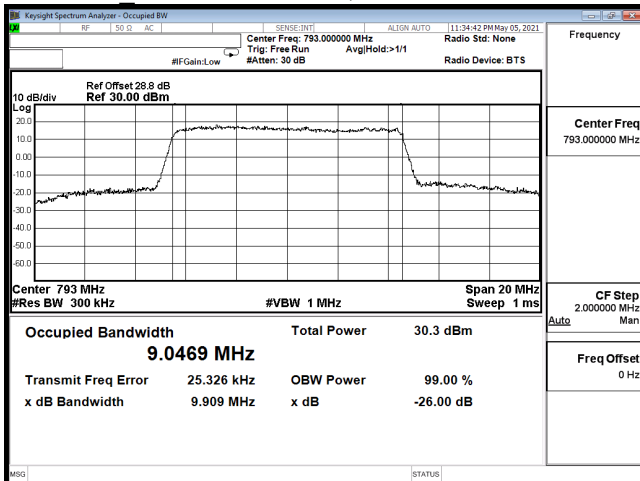
OCC-B14_10M-CH23330-16QAM
