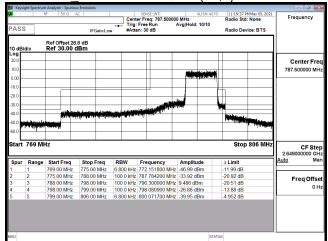
EDGE-B14 5M-CH23355-16QAM(25,0)
