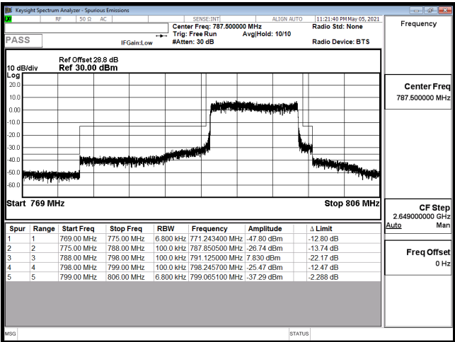
EDGE-B14 10M-CH23330-QPSK(50,0)
