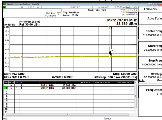
CSE-B14 5M-CH23305-64QAM(1,0)-30M-1G
