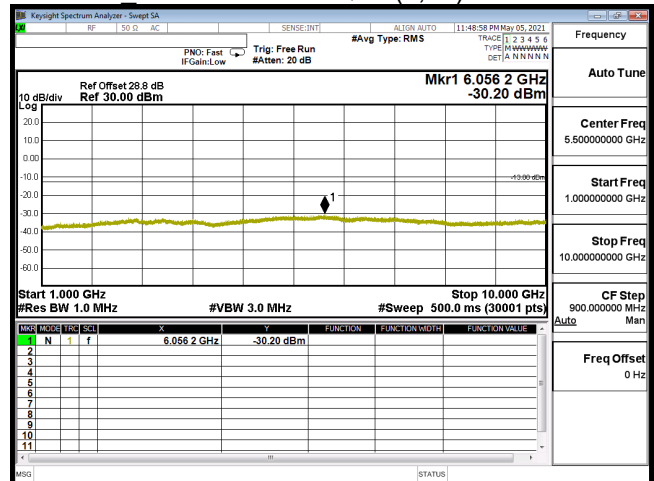
CSE-B14_5M-CH23355-64QAM(1,12)-1G-10G
