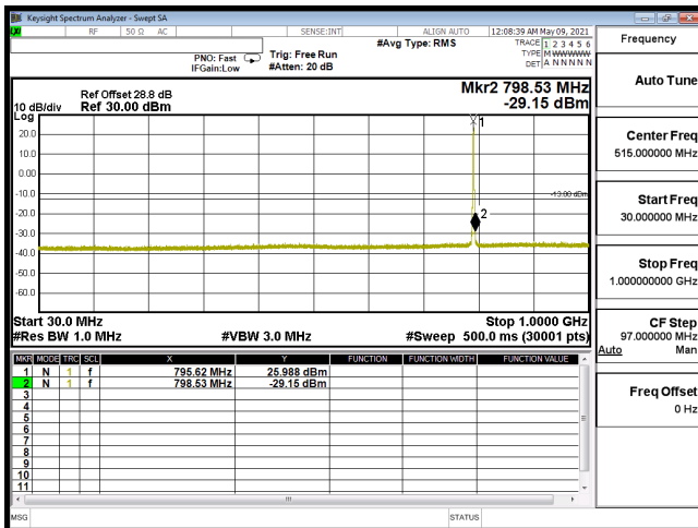
CSE-B14_5M-CH23355-QPSK(1,12)-30M-1G
