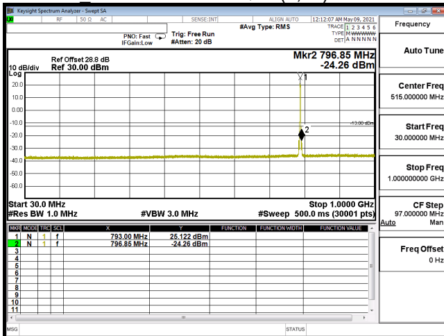
CSE-B14_10M-CH23355-64QAM(1,25)-30M-1G
