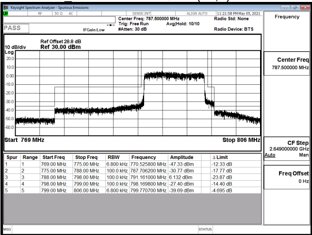
EDGE-B14_10M-CH23330-64QAM(50,0)
