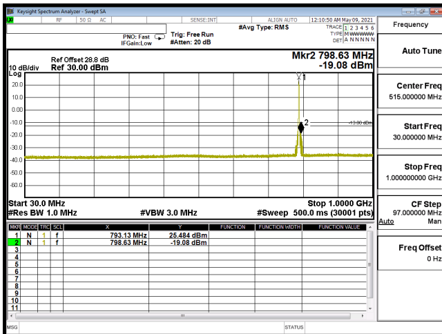
CSE-B14_10M-CH23355-QPSK(1,25)-30M-1G
