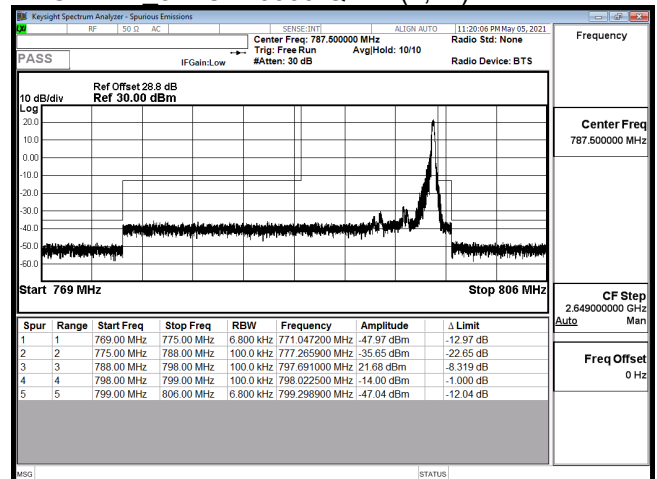
EDGE-B14 5M-CH23355-16QAM(1,24)
