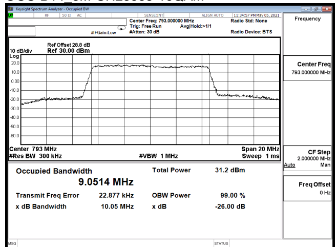
OCC-B14_10M-CH23330-QPSK
