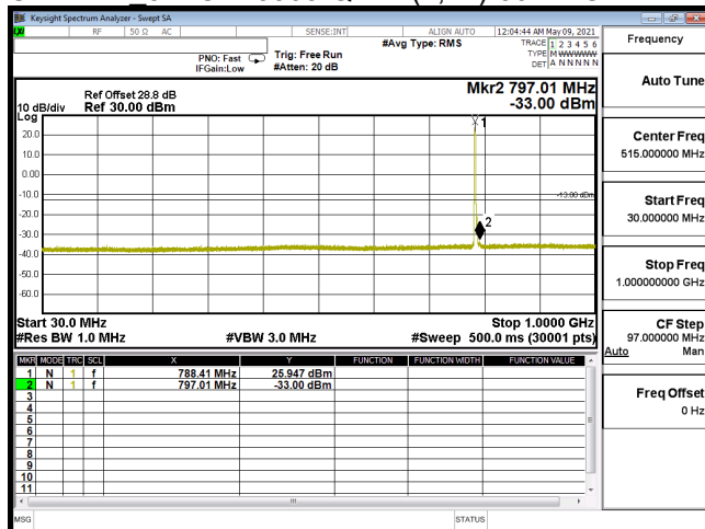
CSE-B14 5M-CH23305-16QAM(1,0)-30M-1G
