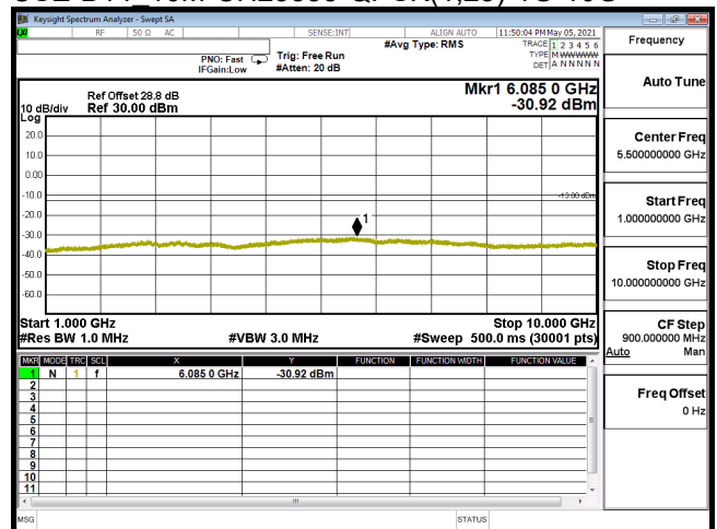
CSE-B14_10M-CH23355-16QAM(1,49)-1G-10G
