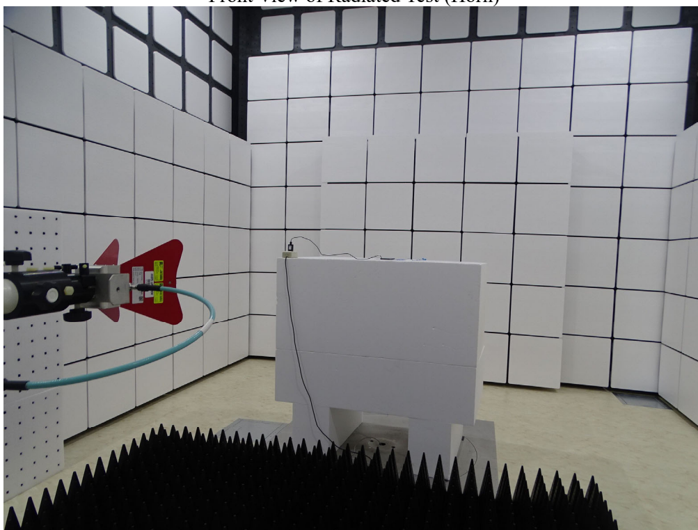
Front View of Radiated Test (Horn)
