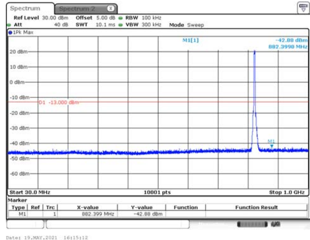
WCDMA_B5_CH4132_RMC_under 1G
