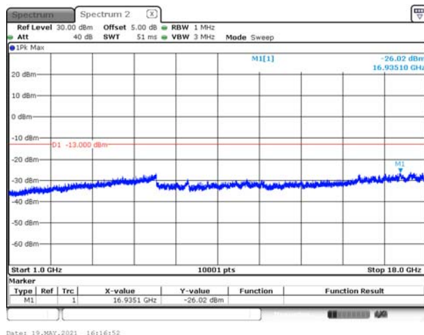
WCDMA_B5_CH4183_RMC_above 1G
