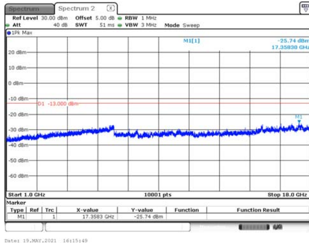
WCDMA_B5_CH4132_RMC_above 1G
