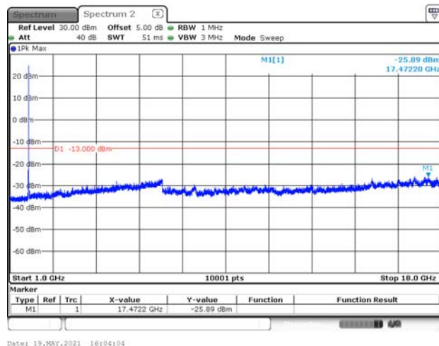
WCDMA_B4_CH1413_RMC_above 1G
