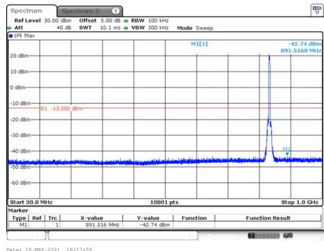
WCDMA_B5_CH4183_RMC_under 1G
