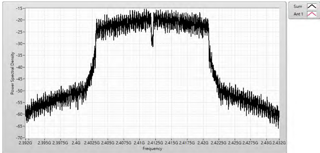
Channel 1 (2412MHz)
