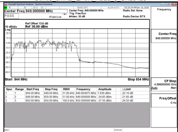
Band5 5MHz QPSK RB25 0 CH20625
