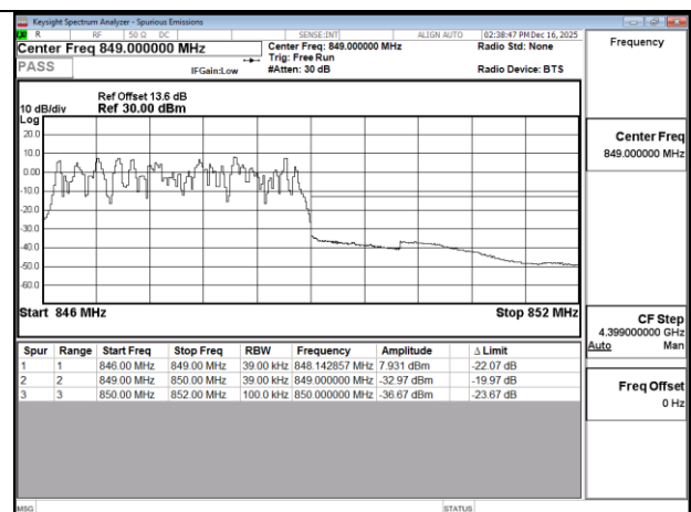
Band5 3MHz QPSK RB15 0 CH20635
