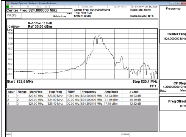
Band5 1.4MHz QPSK RB1 0 CH20407
