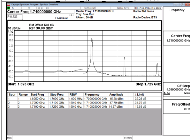
Band4 15MHz QPSK RB1 0 CH20025
