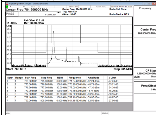
Band13 10MHz QPSK RB1 0 CH23230
