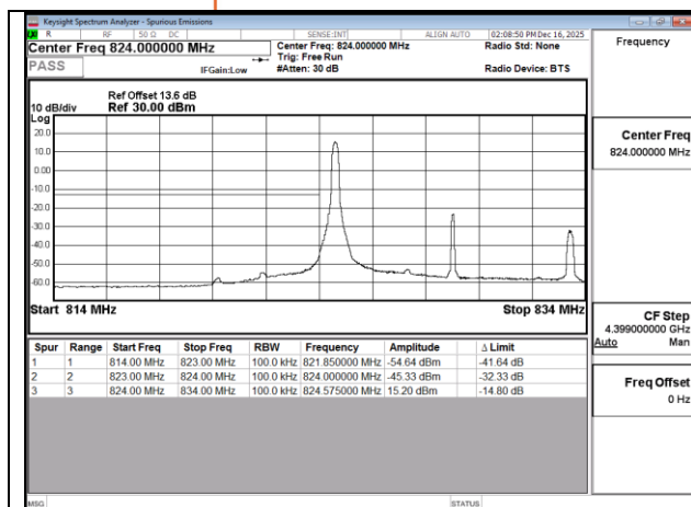
Band5 10MHz QPSK RB1 0 CH20450
