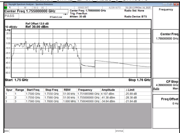
Band4 5MHz QPSK RB25 0 CH20375
