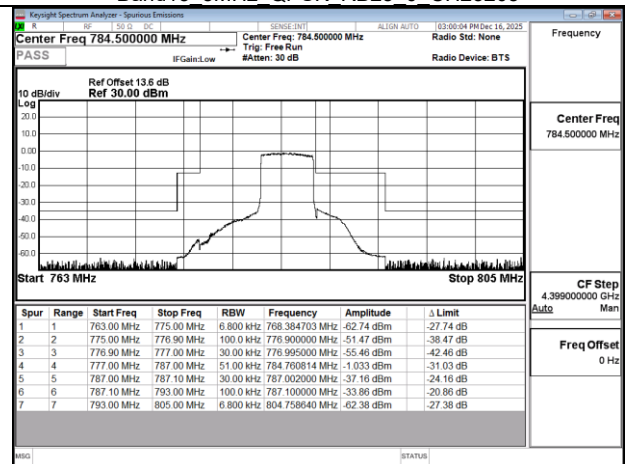
Band13 5MHz QPSK RB25 0 CH23255
