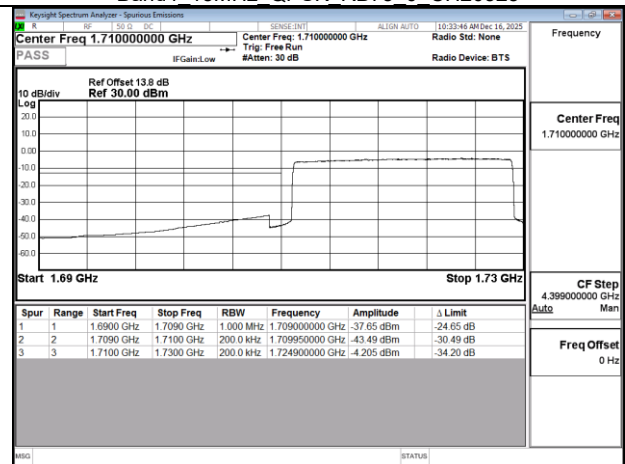
Band4 20MHz QPSK RB100 0 CH20050
