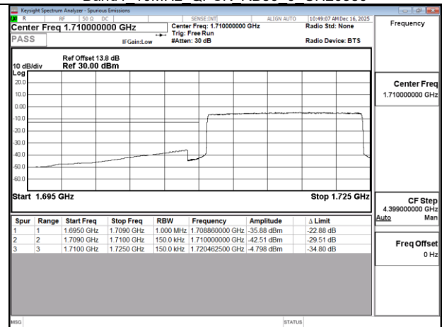
Band4 15MHz QPSK RB75 0 CH20025
