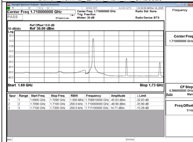
Band4 20MHz QPSK RB1 0 CH20050
