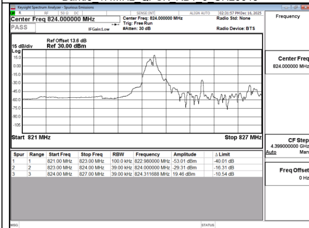
Band5 3MHz QPSK RB1 0 CH20415
