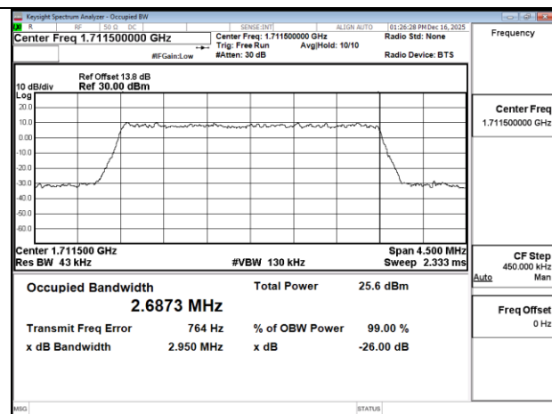
Band4 3MHz 16QAM RB15 0 CH19965
