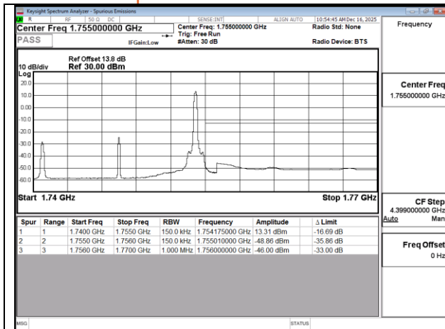
Band4 15MHz QPSK RB1 74 CH20325
