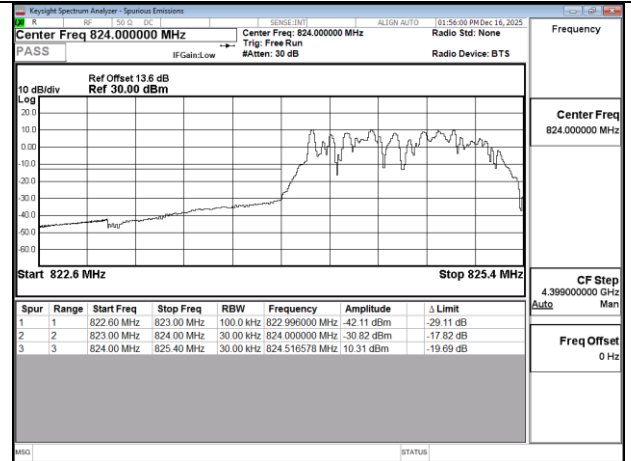
Band5 1.4MHz QPSK RB6 0 CH20407
