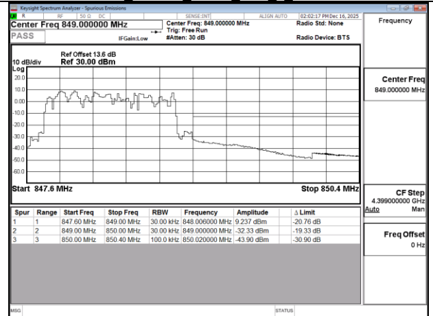
Band5 1.4MHz QPSK RB6 0 CH20643
