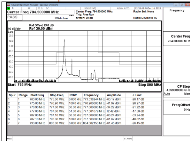
Band13 5MHz QPSK RB1 0 CH23205
