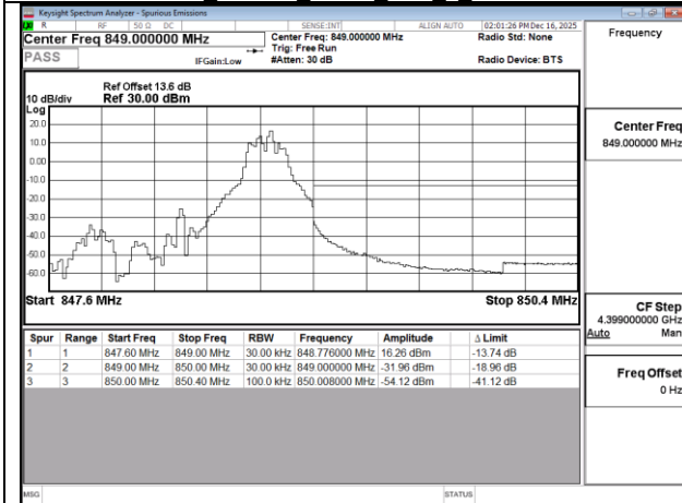
Band5 1.4MHz QPSK RB1 5 CH20643
