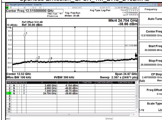
Spurious Emission GFSK 1M DH5 2480MHz
