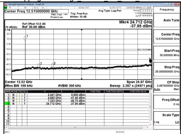
Spurious Emission GFSK 1M DH5 2441MHz
