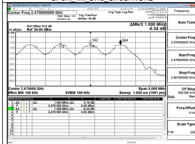
GFSK 1M DH5 CH76CH77CH78
