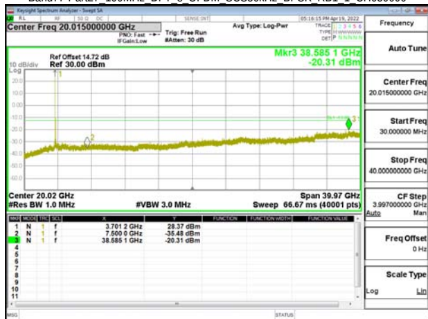
Band77-Part27 100MHz DFT s OFDM SCS30kHz BPSK RB1 1 CH656000
