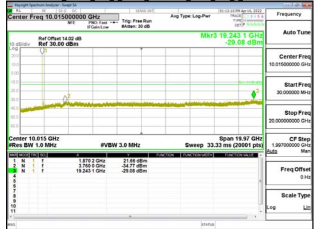
Band2 20MHz DFT s OFDM SCS15kHz BPSK RB1 1 CH380000
