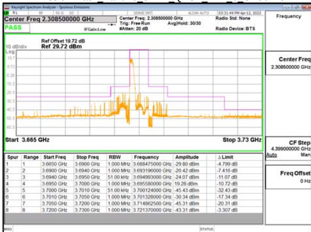
Emission Mask Band48 5MHz QPSK RB1 0 CH56715
