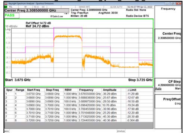
Emission Mask Band48 10MHz QPSK RB50 0 CH56690
