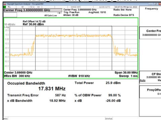
Band48 20MHz 256QAM RB100 0 CH56640
