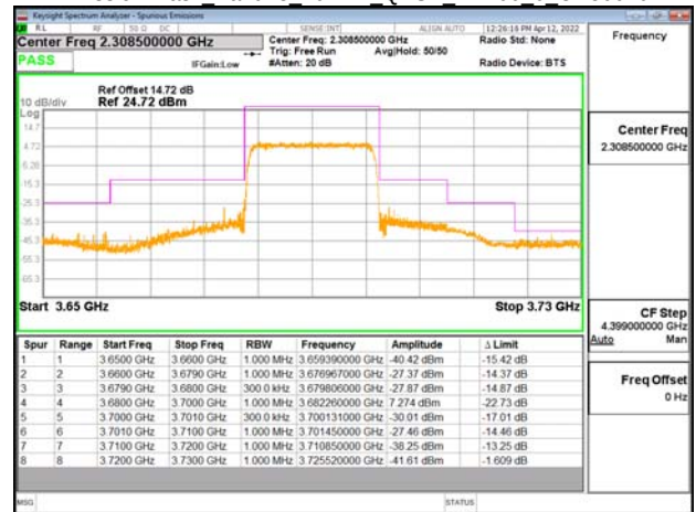
Emission Mask Band48 20MHz QPSK RB100 0 CH56640
