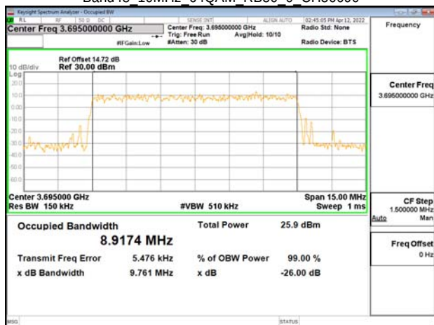
Band48 10MHz 64QAM RB50 0 CH56690
