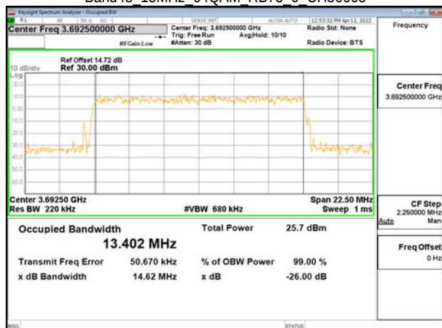
Band48 15MHz 64QAM RB75 0 CH56665
