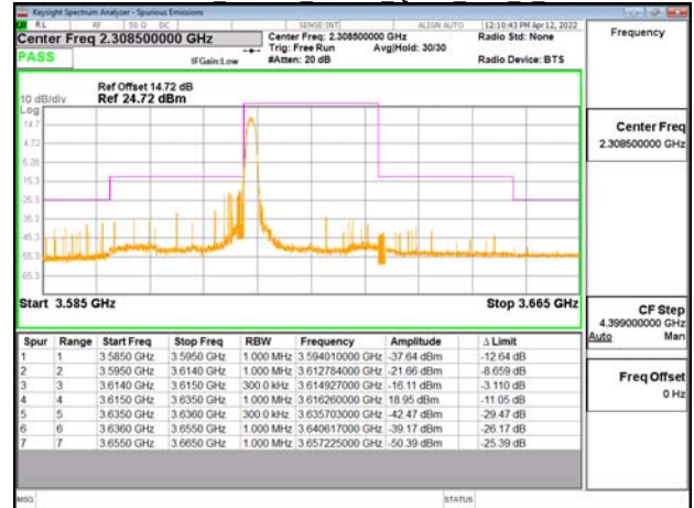
Emission Mask Band48 20MHz QPSK RB1 0 CH56640
