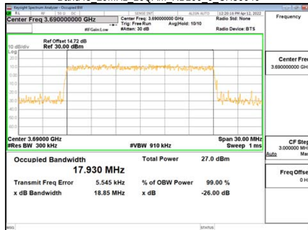
Band48 20MHz 16QAM RB100 0 CH56640
