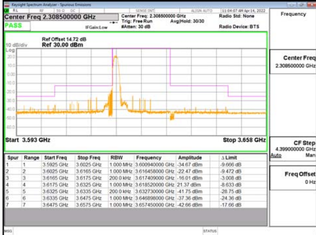
Emission Mask Band48 15MHz QPSK RB1 0 CH56665
