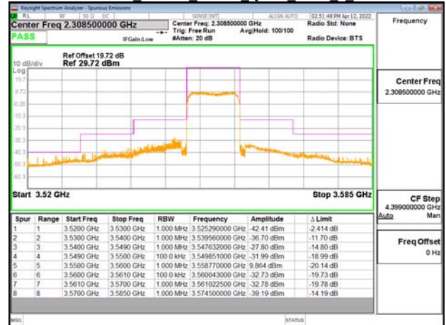
Emission Mask Band48 10MHz QPSK RB50 0 CH55990
