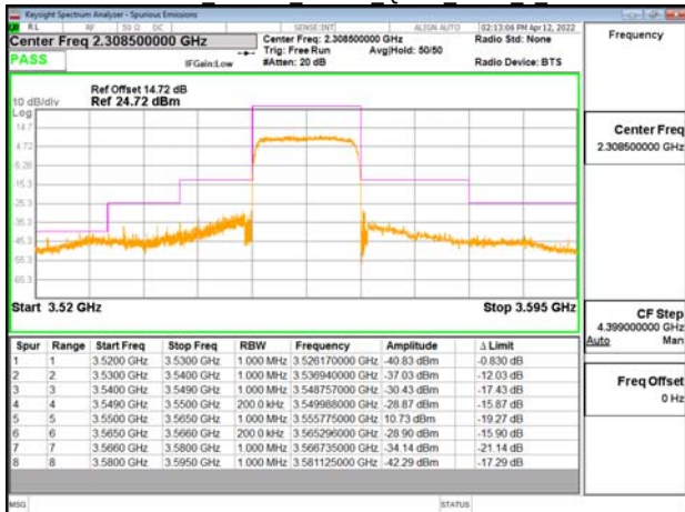
Emission Mask Band48 15MHz QPSK RB75 0 CH55990
