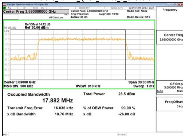
Band48 20MHz QPSK RB100 0 CH56640
