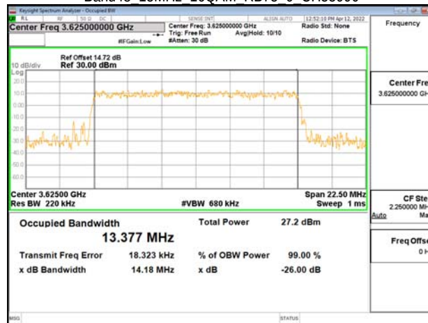
Band48 15MHz 16QAM RB75 0 CH56665
