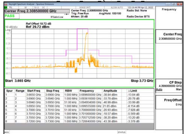
Emission Mask Band48 5MHz QPSK RB1 24 CH56715
