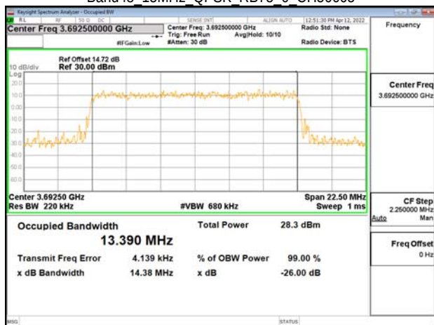
Band48 15MHz QPSK RB75 0 CH56665
