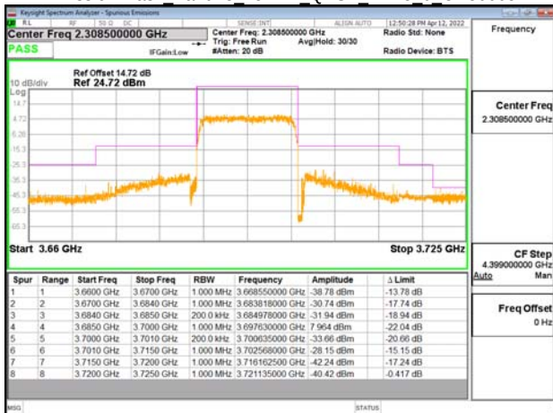
Emission Mask Band48 15MHz QPSK RB75 0 CH56665
