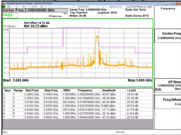
Emission Mask Band48 20MHz QPSK RB1 99 CH56640
