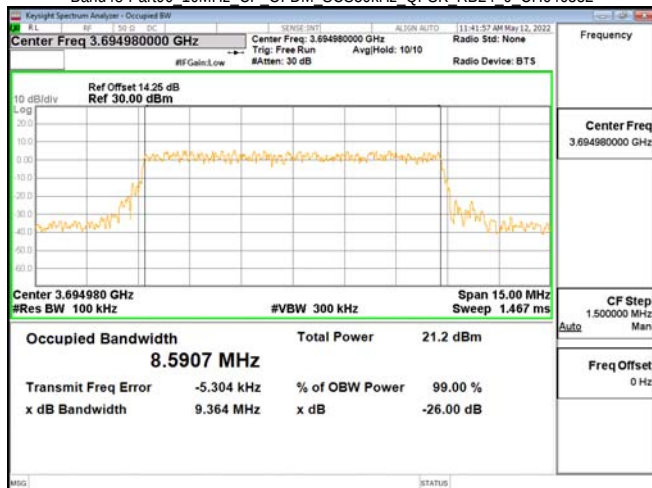
Band48-Part96_10MHz_CP_OFDM_SCS30kHz_QPSK_RB24_0_CH646332
