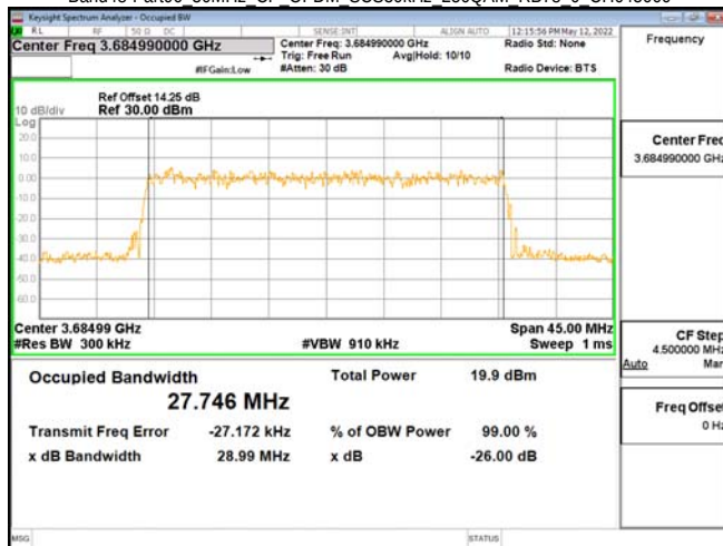
Band48-Part96 30MHz CP OFDM SCS30kHz 256QAM RB78 0 CH645666
