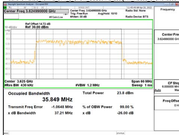
Band48-Part96 40MHz DFT s OFDM SCS30kHz 256QAM RB100 0 CH645332
