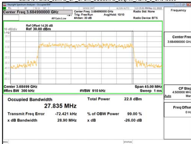
Band48-Part96 30MHz CP OFDM SCS30kHz 16QAM RB78 0 CH645666
