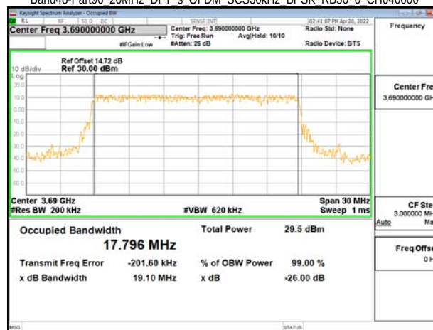
Band48-Part96 20MHz DFT s OFDM SCS30kHz BPSK RB50 0 CH646000
