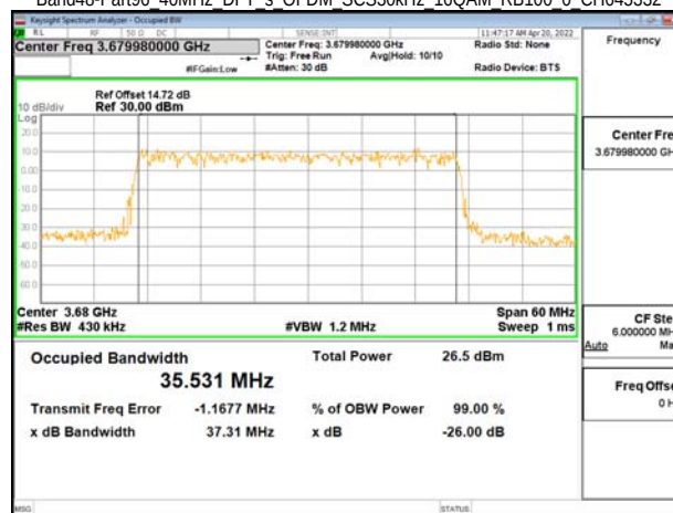
Band48-Part96 40MHz DFT s OFDM SCS30kHz 16QAM RB100 0 CH645332
