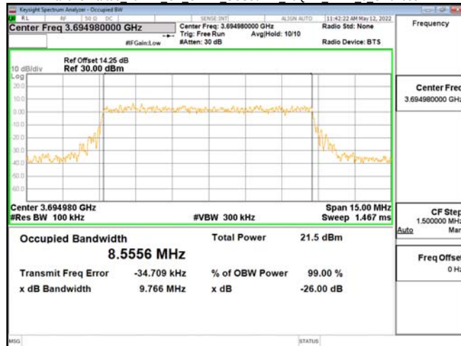
Band48-Part96_10MHz_CP_OFDM_SCS30kHz_16QAM_RB24_0_CH646332
