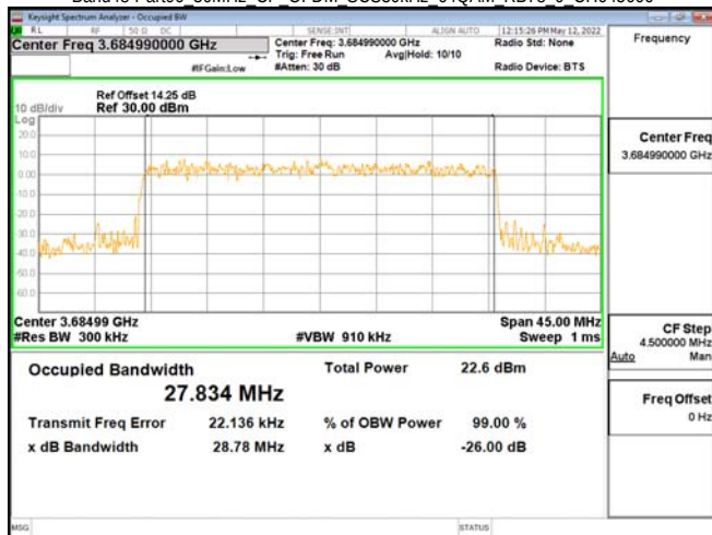
Band48-Part96 30MHz CP OFDM SCS30kHz 64QAM RB78 0 CH645666
