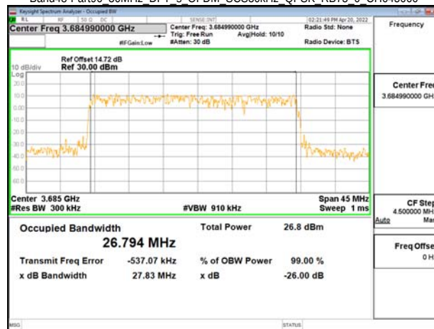
Band48-Part96 30MHz DFT s OFDM SCS30kHz QPSK RB75 0 CH645666
