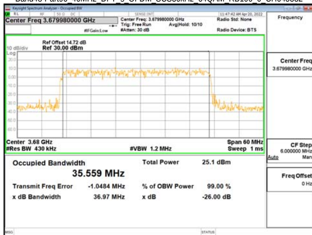
Band48-Part96 40MHz DFT s OFDM SCS30kHz 64QAM RB100 0 CH645332
