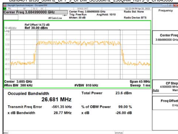
Band48-Part96 30MHz DFT s OFDM SCS30kHz 256QAM RB75 0 CH645666
