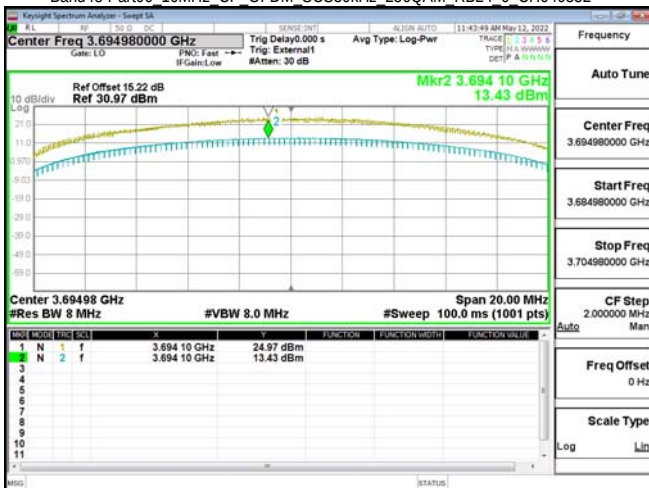
Band48-Part96 10MHz_CP_OFDM_SCS30kHz_256QAM_RB24_0_CH646332
