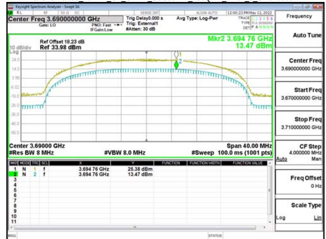
Band48-Part96 20MHz_CP_OFDM_SCS30kHz_256QAM_RB51_0_CH646000
