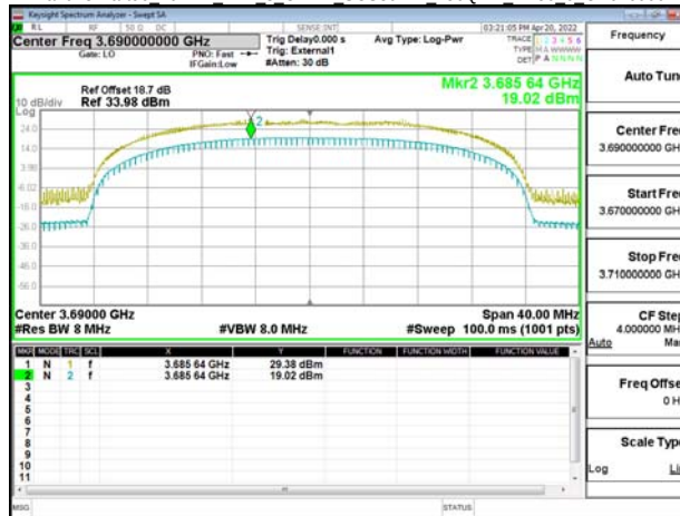
Band48-Part96 20MHz DFT s OFDM SCS30kHz 256QAM RB50 0 CH646000
