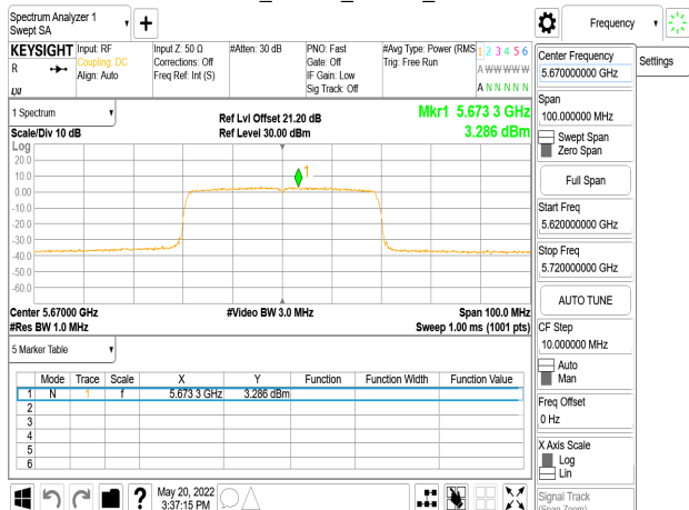
802.11ax_40MHz_Chain0_5670MHz
