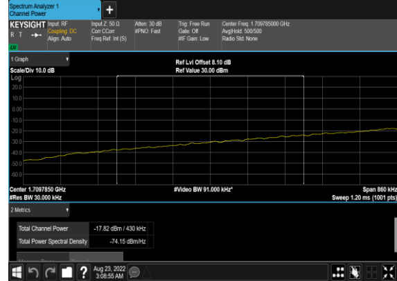
N66(40M)_DFT-s- OFDM_QPSK_Edge_1RB_Left_Low_CH_CHP_PASS
