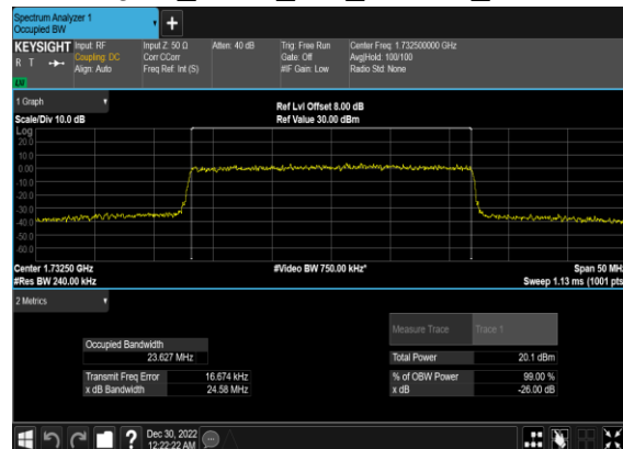
N66(25M)_CP-OFDM_256 QAM_Outer_Full_426500_CH
