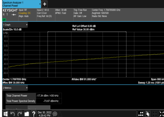
B2_N66(40M)_DFT-s- OFDM_BPSK_Edge_1RB_Left_Low_CH_CHP_PASS
