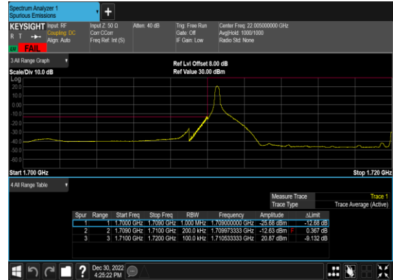
B2_N66(20M)_DFT-s- OFDM_QPSK_Edge_1RB_Left_Low_CH
