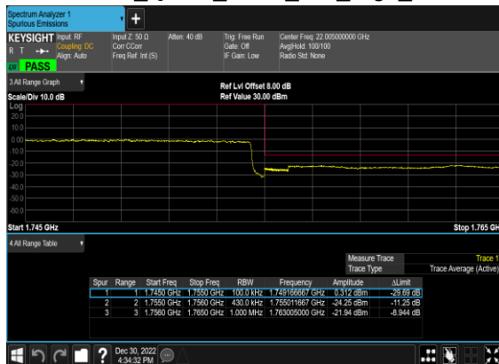
B2_N66(40M)_DFT-s- OFDM_QPSK_Outer_Full_High_CH
