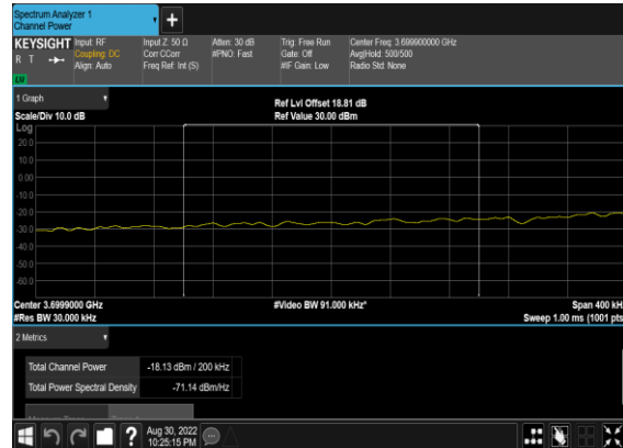
N77(20M)_CP- OFDM_QPSK_Edge_1RB_Left_Low_CH CHP- PASS
