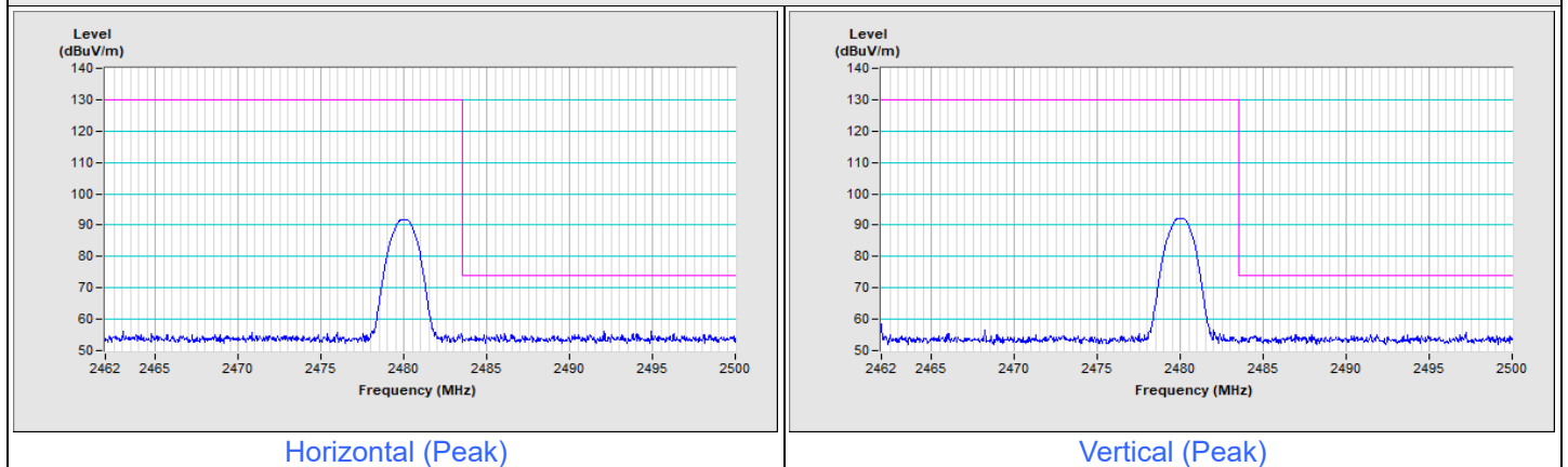
BT 8DPSK Channel 78
