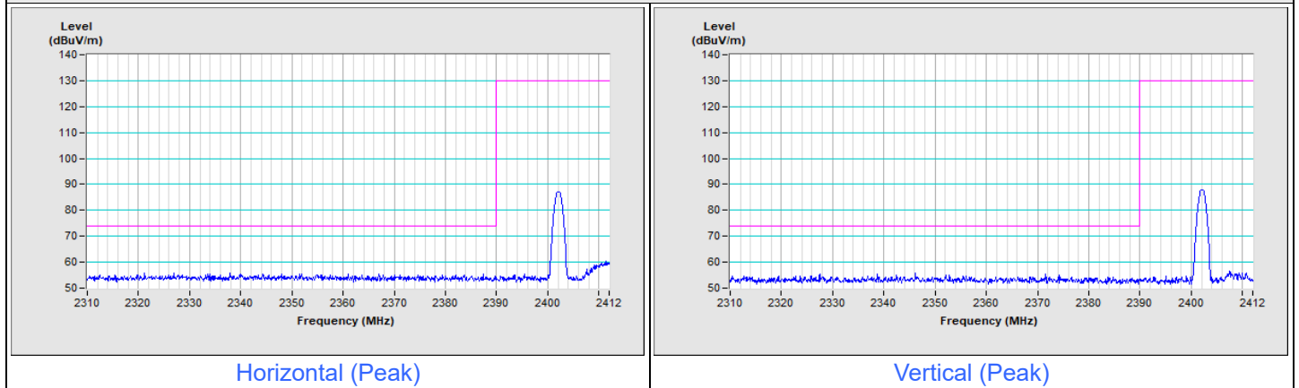
BT 8DPSK Channel 0
