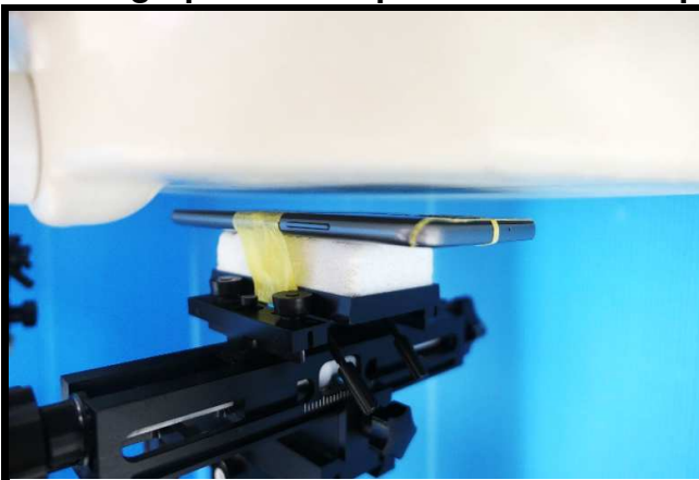
Front Face of EUT Tested at 10 mm
