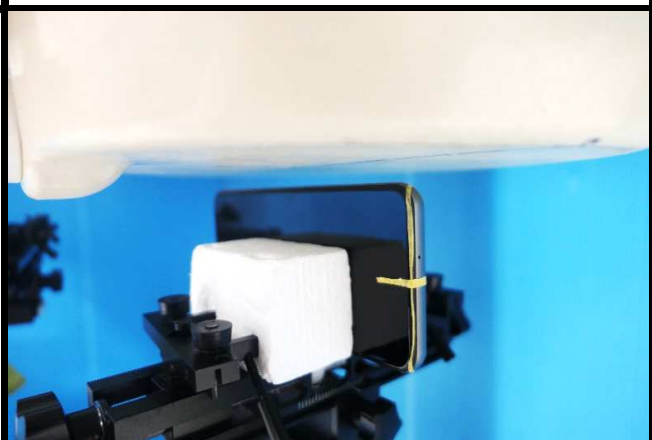
Right Side of EUT Tested at 10 mm
