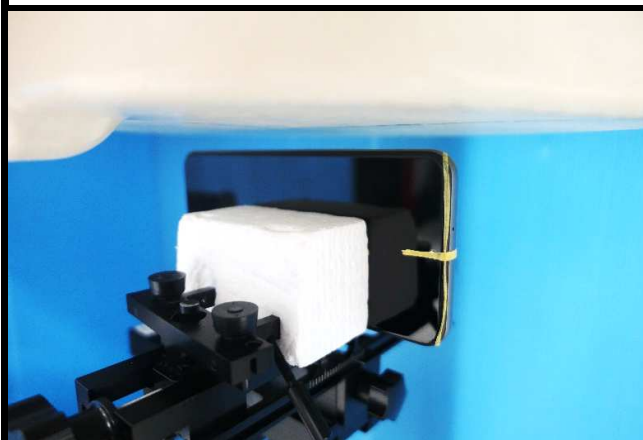
Left Side of EUT Tested at 10 mm
