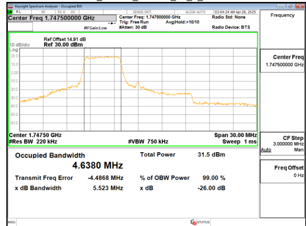
Band4_15MHz_16QAM_25_0_CH20325
