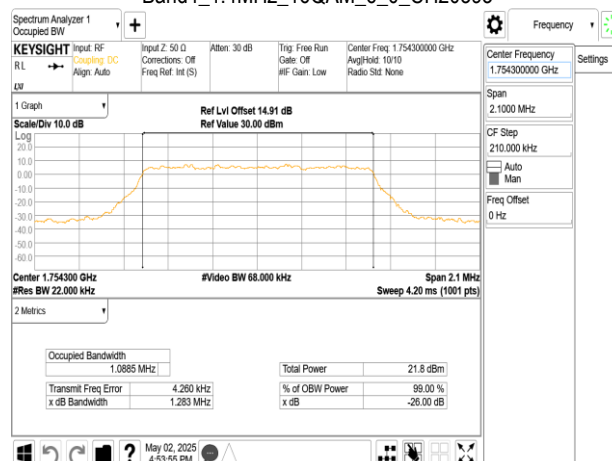
Band4_1.4MHz_16QAM_6_0_CH20393
