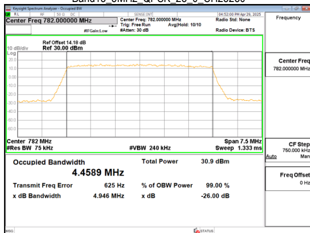
Band13_5MHz_QPSK_25_0_CH23255
