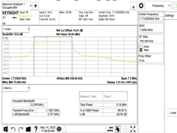
Band4_5MHz_64QAM_25_0_CH20175
