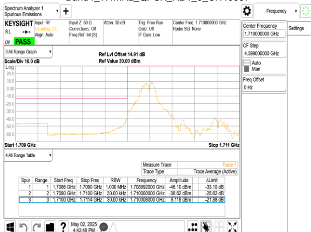
Band4_1.4MHz_QPSK_RB6_0_CH19957
