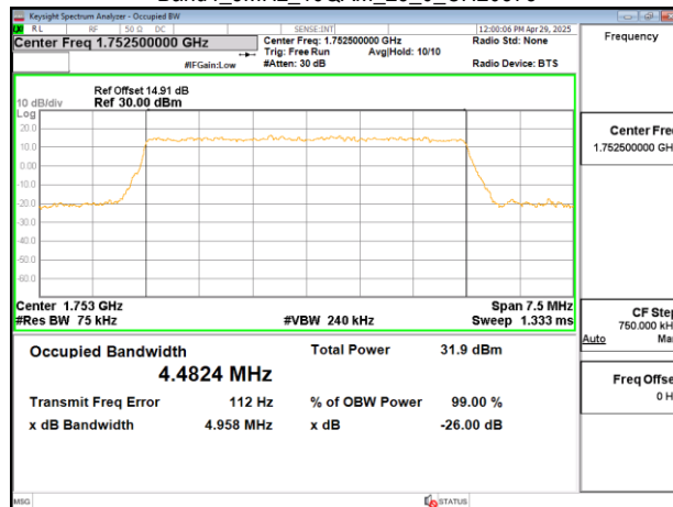
Band4_5MHz_16QAM_25_0_CH20375
