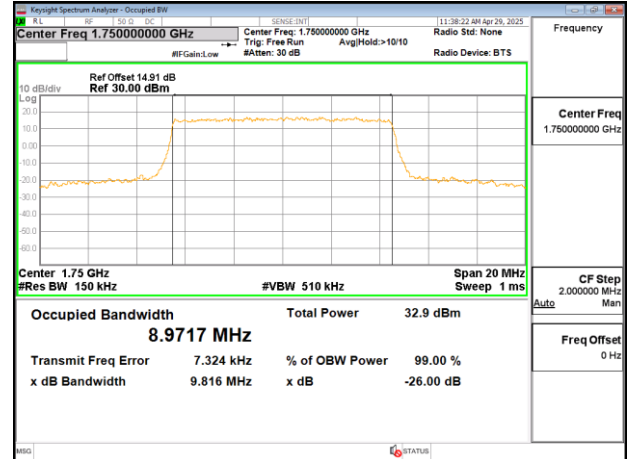
Band4_10MHz_QPSK_50_0_CH20350
