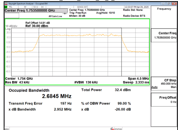
Band4_3MHz_QPSK_15_0_CH20385
