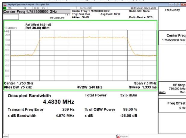
Band4_5MHz_QPSK_25_0_CH20375
