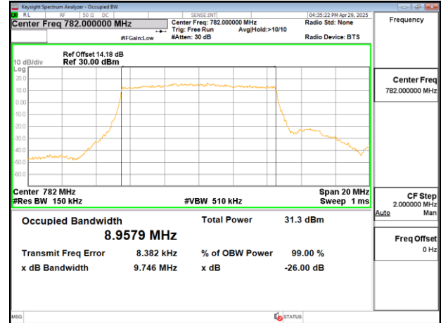
Band13_10MHz_16QAM_25_0_CH23230
