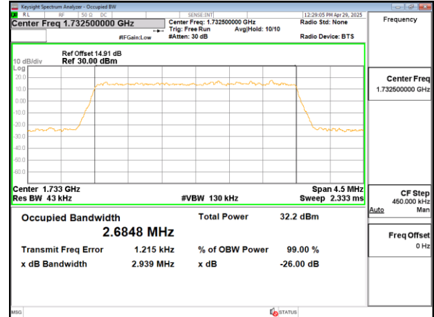
Band4_3MHz_QPSK_15_0_CH20385
