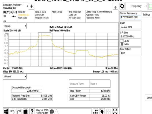
Band4_10MHz_64QAM_50_0_CH20350
