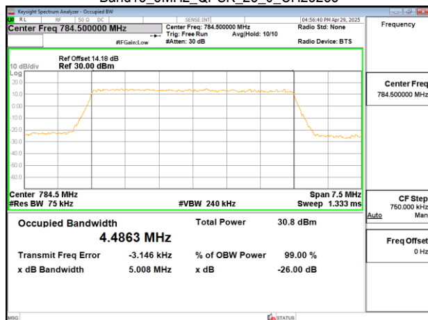
Band13_5MHz_QPSK_25_0_CH23255
