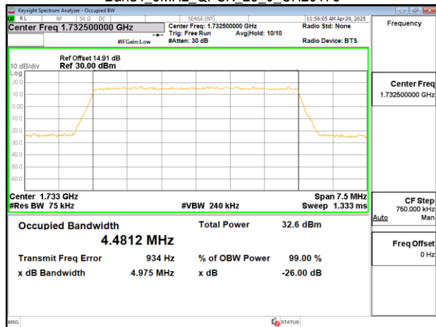
Band4_5MHz_QPSK_25_0_CH20375
