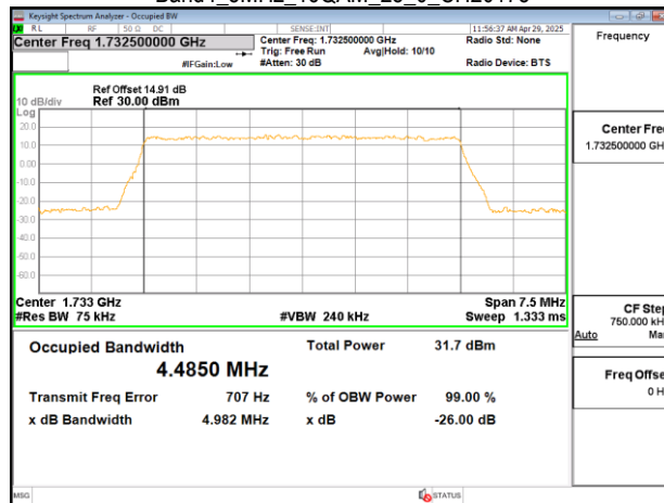
Band4_5MHz_16QAM_25_0_CH20375
