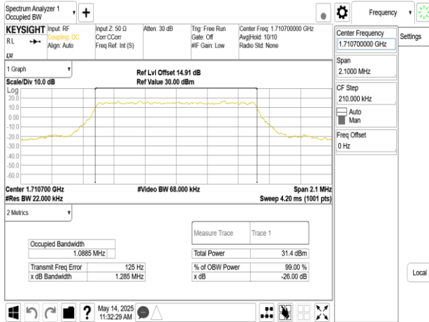
Band4_1.4MHz_64QAM_6_0_CH20175
