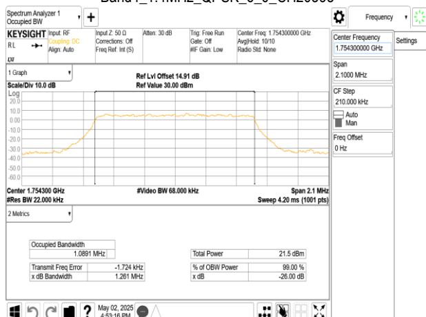
Band4_1.4MHz_QPSK_6_0_CH20393
