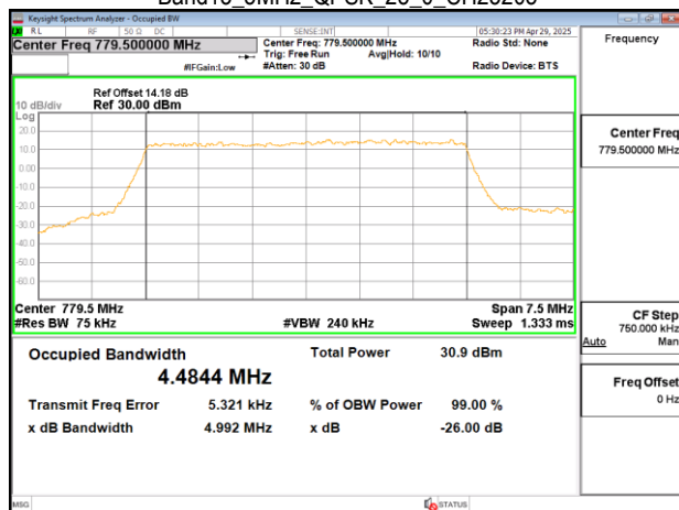
Band13_5MHz_QPSK_25_0_CH23230
