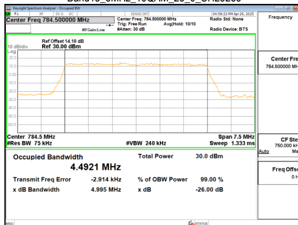
Band13_5MHz_16QAM_25_0_CH23255
