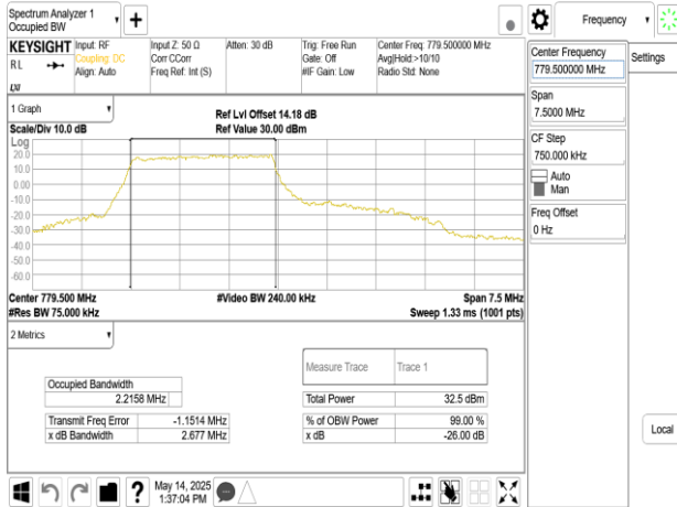
Band13_5MHz_64QAM_25_0_CH23230
