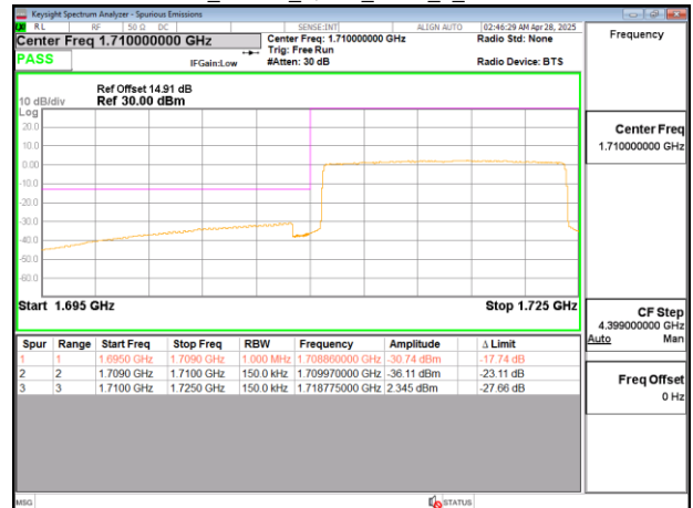
Band4_15MHz_QPSK_RB75_0_CH20025
