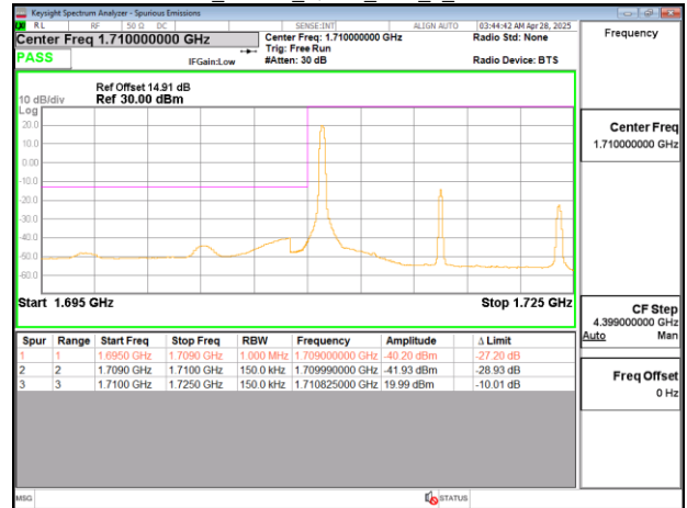
Band4_15MHz_QPSK_RB75_0_CH20025
