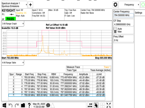
Band13_5MHz_QPSK_RB25_0_CH23205
