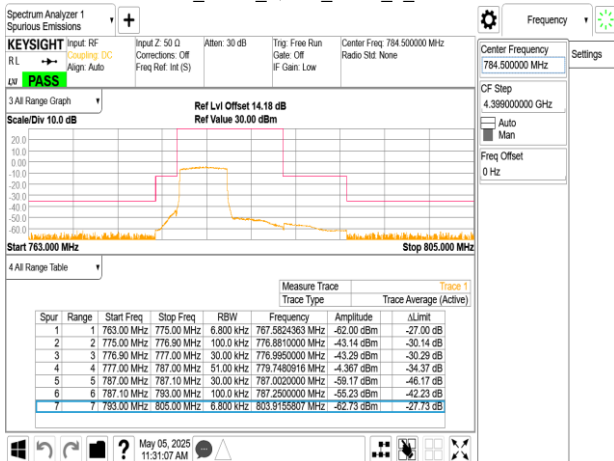
Band13_5MHz_QPSK_RB1_24_CH23255
