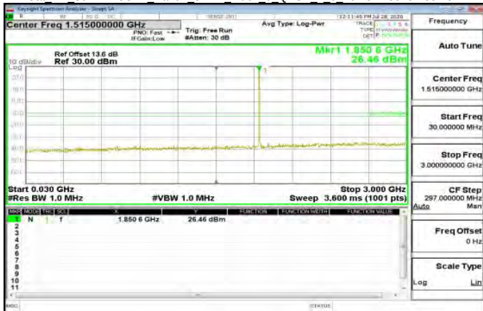
Cat M1 30MHz~3GHz Band2 5MHz index 0 QPSK 1 0 LowCH18625-1852.5
