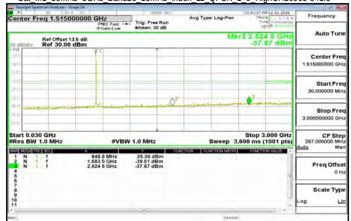
Cat M1 30MHz~3GHz Band26 15MHz index 11 QPSK 1 0 HighCH26965-841.5
