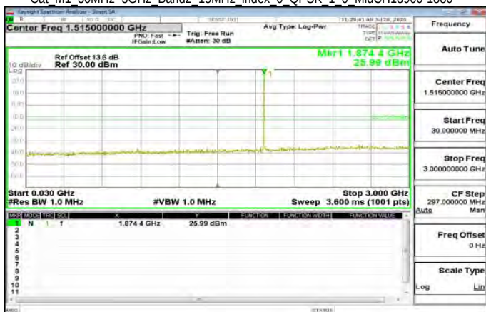
Cat M1 30MHz~3GHz Band2 15MHz index 0 QPSK 1 0 MidCH18900-1880
