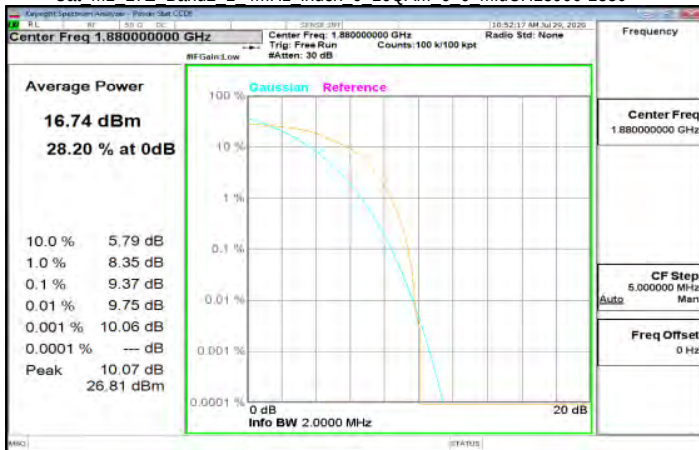
Cat M1 LTE Band2 1 4MHz index 0 16QAM 6 0 MidCH18900-1880
