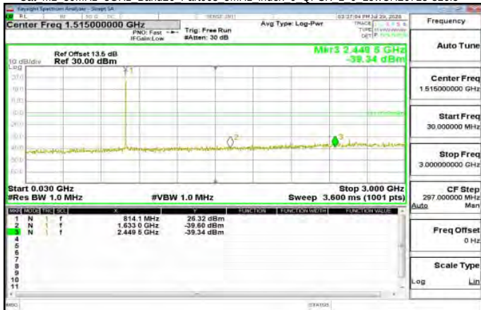
Cat M1 30MHz-3GHz Band26 Part90s 5MHz index 0 QPSK 1 0 LowCH26715-816.5
