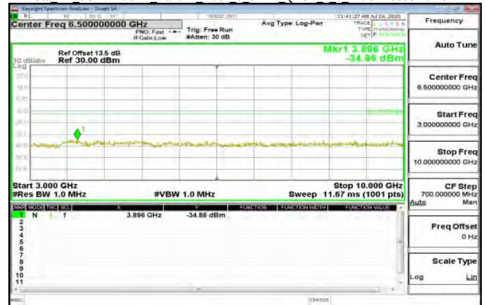
Cat M1 3GHz-10GHz Band12 index 0 3MHz QPSK 1 0 MidCH23095-707.5
