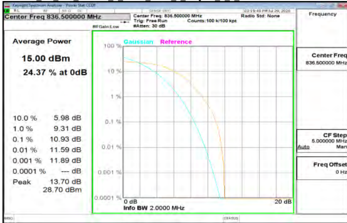
Cat M1 LTE Band26 1 4MHz index 0 16QAM 6 0 MidCH26915-836.5
