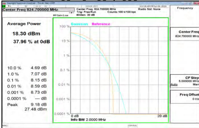
Cat M1 LTE Band26 1 4MHz index 0 16QAM 6 0 LowCH26797-824.7
