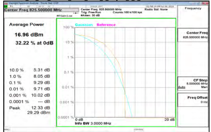
Cat M1 LTE Band26 3MHz index 0 16QAM 6 0 LowCH26805-825.5
