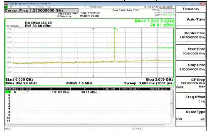
Cat M1 30MHz~3GHz Band2 10MHz index 7 QPSK 1 0 HighCH19150-1905
