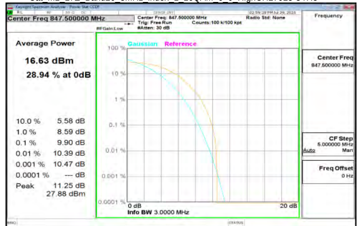
Cat M1 LTE Band26 3MHz index 1 16QAM 6 0 HighCH27025-847.5
