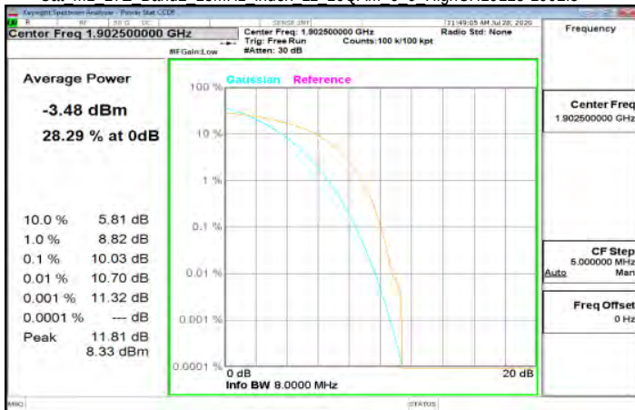
Cat M1 LTE Band2 15MHz index 11 16QAM 6 0 HighCH19125-1902.5
