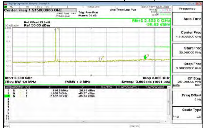
Cat M1 30MHz~3GHz Band26 10MHz index 7 QPSK 1 0 HighCH26990-844
