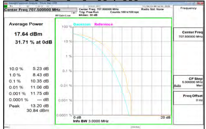
Cat M1 LTE Band12 3MHz index 0 16QAM 6 0 MidCH23095-707.5
