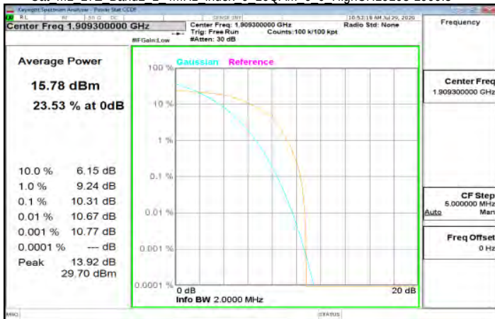
Cat M1 LTE Band2 1 4MHz index 0 16QAM 6 0 HighCH19193-1909.3
