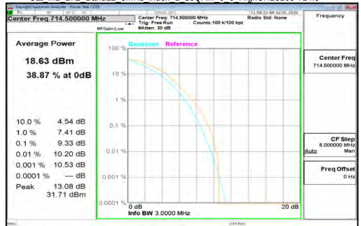
Cat M1 LTE Band12 3MHz index 1 16QAM 6 0 HighCH23165-714.5
