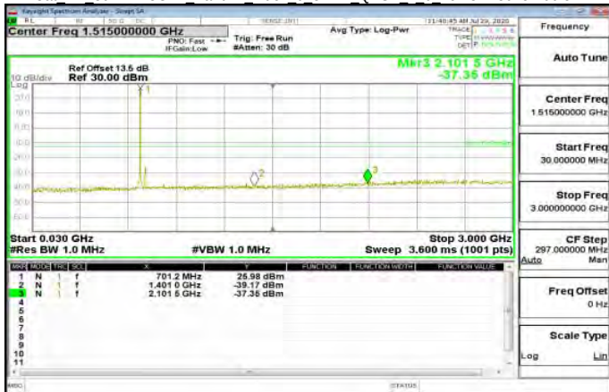
Cat M1 30MHz-3GHz Band12 index 0 3MHz QPSK 1 0 LowCH23025-700.5
