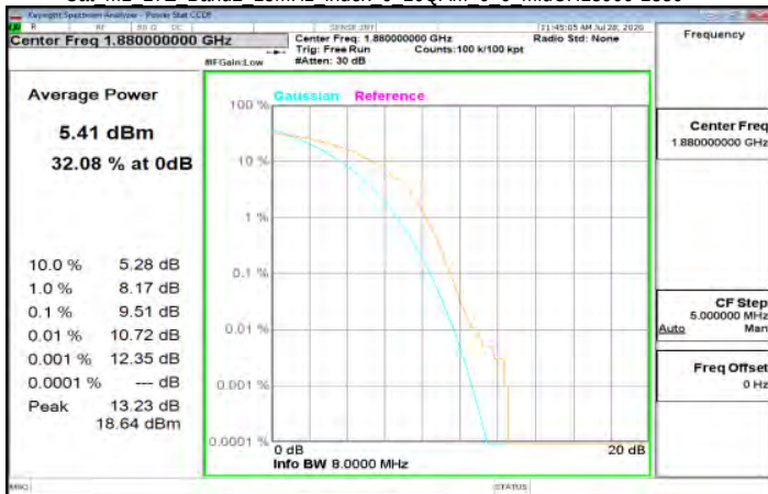
Cat M1 LTE Band2 15MHz index 0 16QAM 6 0 MidCH18900-1880
