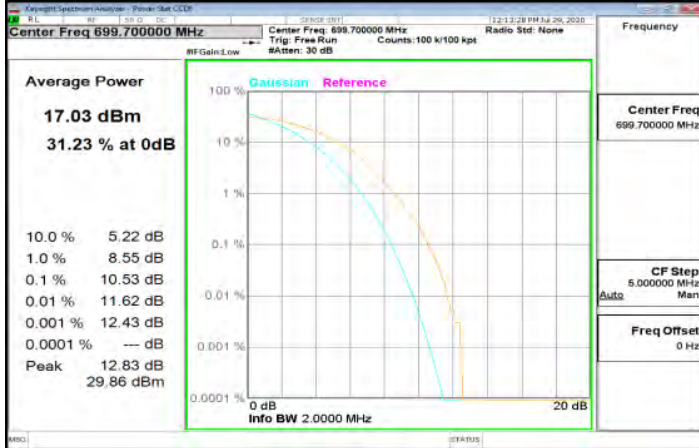
Cat M1 LTE Band12 1 4MHz index 0 16QAM 6 0 LowCH23017-699.7
