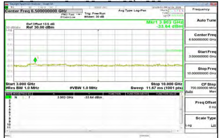
Cat M1 3GHz-10GHz Band26 1 4MHz index 0 QPSK 1 0 MidCH26915-836.5
