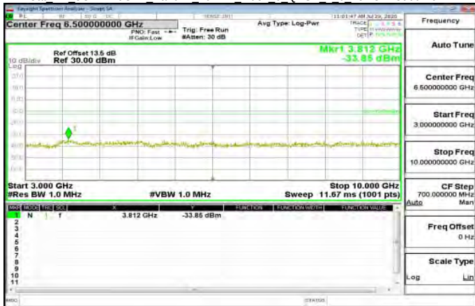
Cat M1 3GHz~10GHz Band12 10MHz index 0 QPSK 1 0 LowCH23060-704
