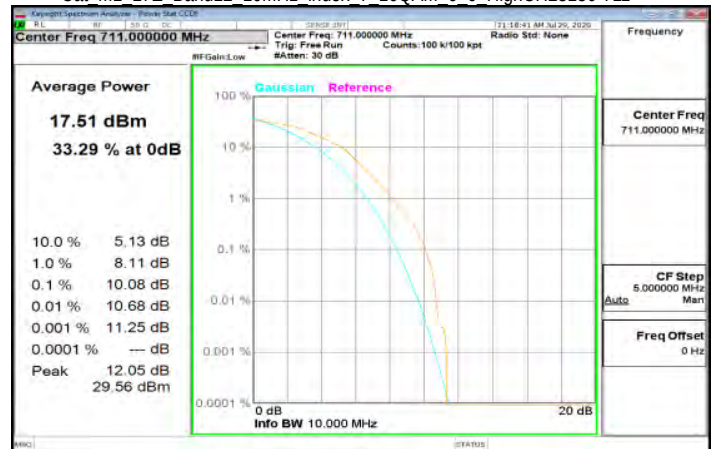
Cat M1 LTE Band12 10MHz index 7 16QAM 6 0 HighCH23130-711
