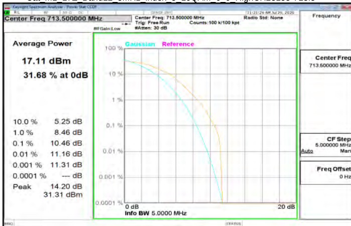
Cat M1 LTE Band12 5MHz index 3 16QAM 6 0 HighCH23155-713.5
