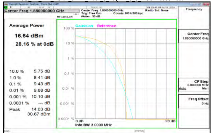
Cat M1 LTE Band2 3MHz index 0 16QAM 6 0 MidCH18900-1880
