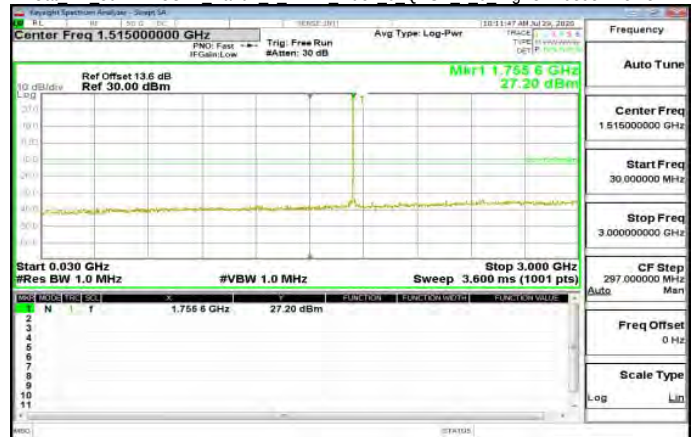
Cat M1 30MHz-3GHz Band4 1 4MHz index 0 QPSK 1 0 HighCH20393-1754.3
