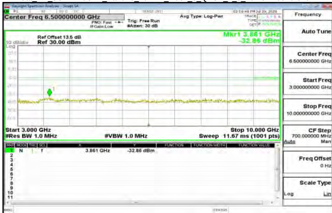
Cat M1 3GHz~10GHz Band26 10MHz index 0 QPSK 1 0 LowCH26840-829
