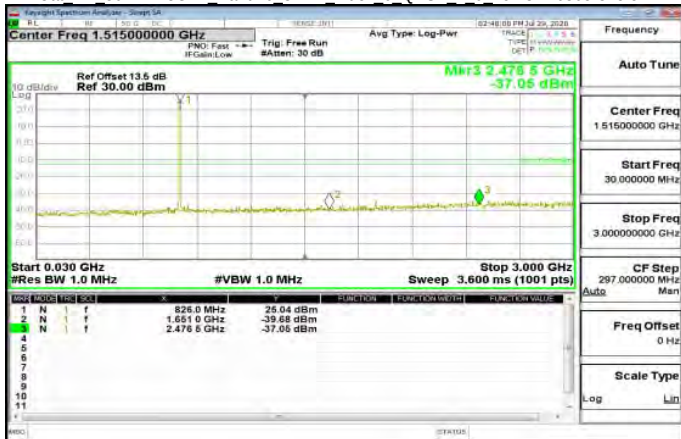
Cat M1 30MHz-3GHz Band26 3MHz index 0 QPSK 1 0 LowCH26805-825.5
