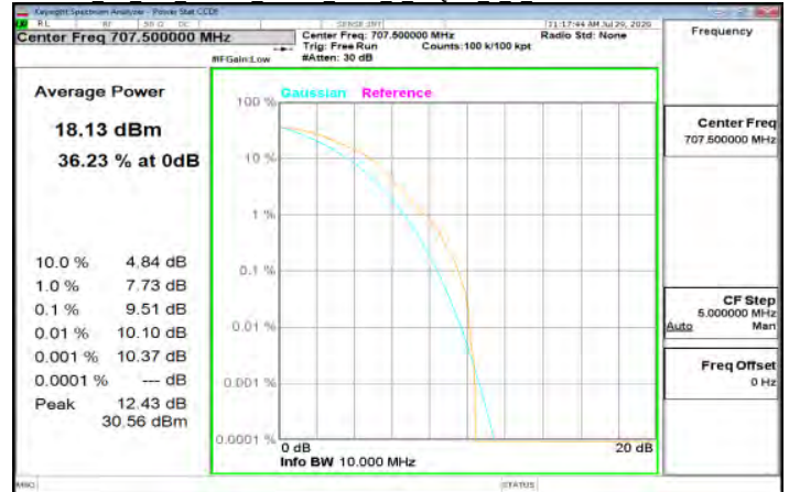
Cat M1 LTE Band12 10MHz index 0 16QAM 6 0 MidCH23095-707.5
