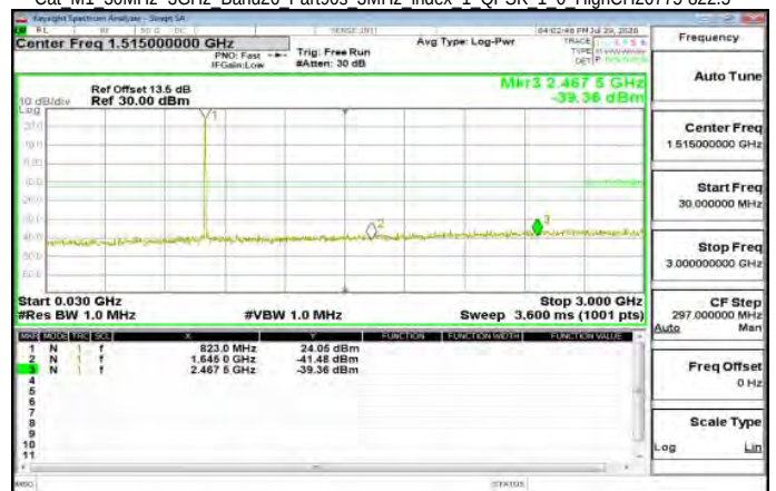
Cat M1 30MHz-3GHz Band26 Part90s 3MHz index 1 QPSK 1 0 HighCH26775-822.5
