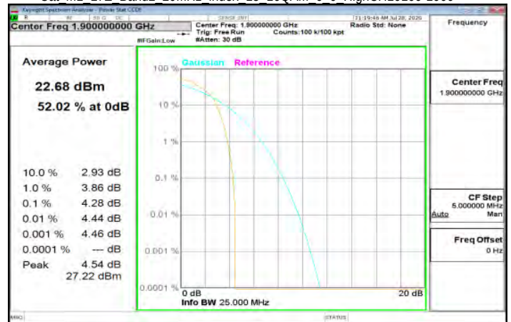
Cat M1 LTE Band2 20MHz index 15 16QAM 6 0 HighCH19100-1900
