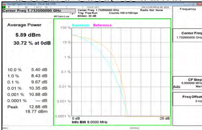
Cat M1 LTE Band4 15MHz index 0 16QAM 6 0 MidCH20175-1732.5
