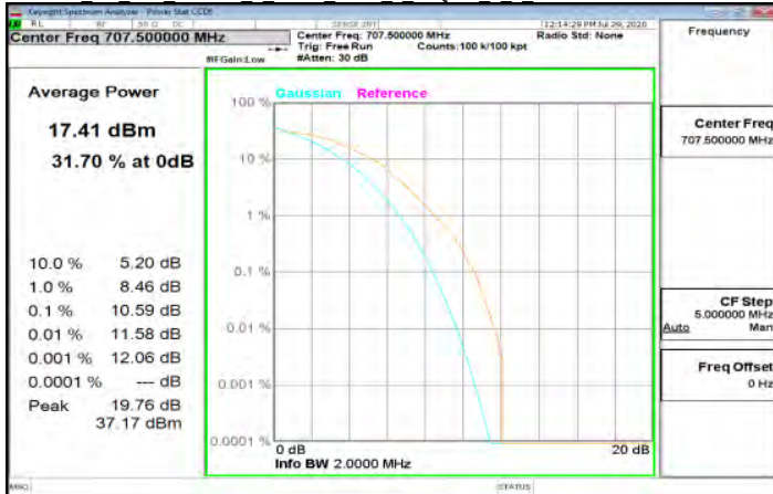
Cat M1 LTE Band12 1 4MHz index 0 16QAM 6 0 MidCH23095-707.5
