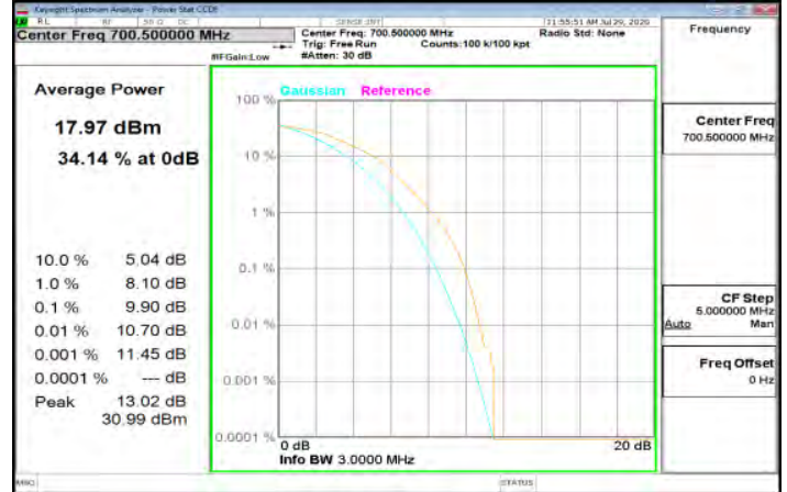
Cat M1 LTE Band12 3MHz index 0 16QAM 6 0 LowCH23025-700.5
