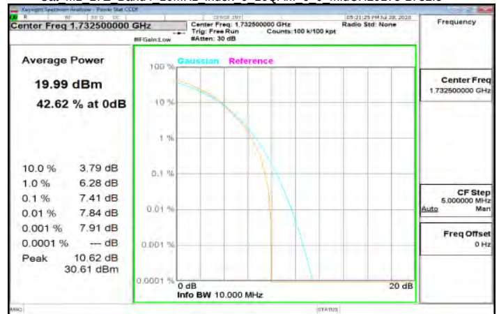
Cat M1 LTE Band4 10MHz index 0 16QAM 6 0 MidCH20175-1732.5
