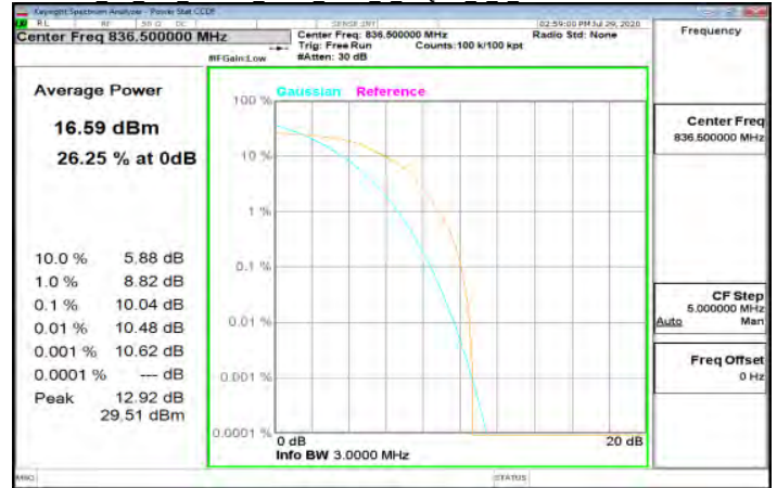
Cat M1 LTE Band26 3MHz index 0 16QAM 6 0 MidCH26915-836.5
