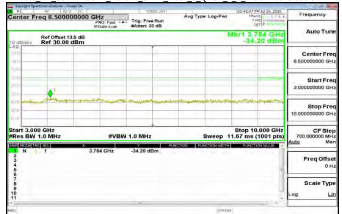
Cat M1 3GHz-10GHz Band26 3MHz index 0 QPSK 1 0 MidCH26915-836.5
