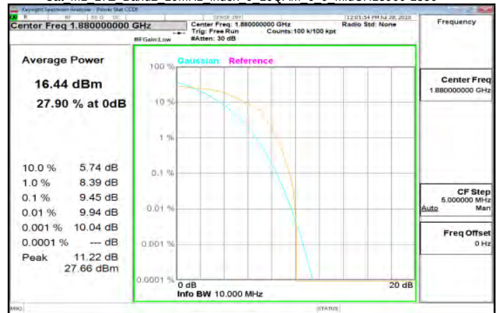
Cat M1 LTE Band2 10MHz index 0 16QAM 6 0 MidCH18900-1880
