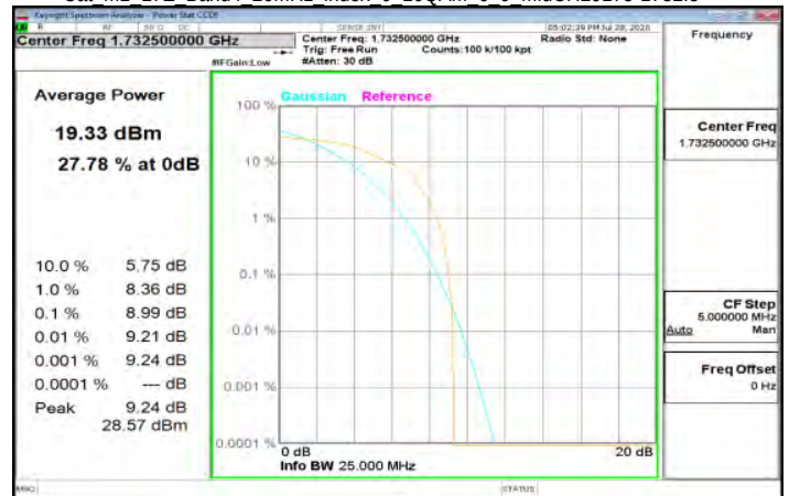
Cat M1 LTE Band4 20MHz index 0 16QAM 6 0 MidCH20175-1732.5
