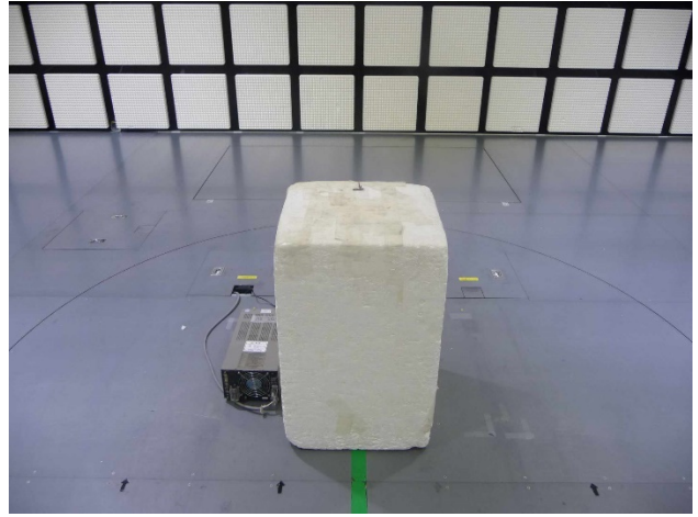
ANT, Nordic Original, IEEE802.15.4 Front
