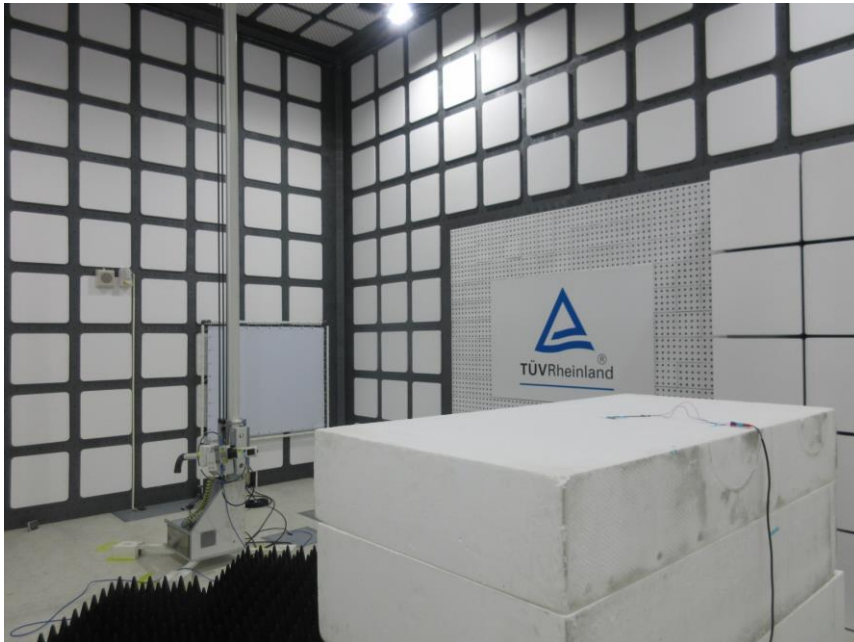
Photograph 6: Set-up for Spurious Emissions (Back View 4)
