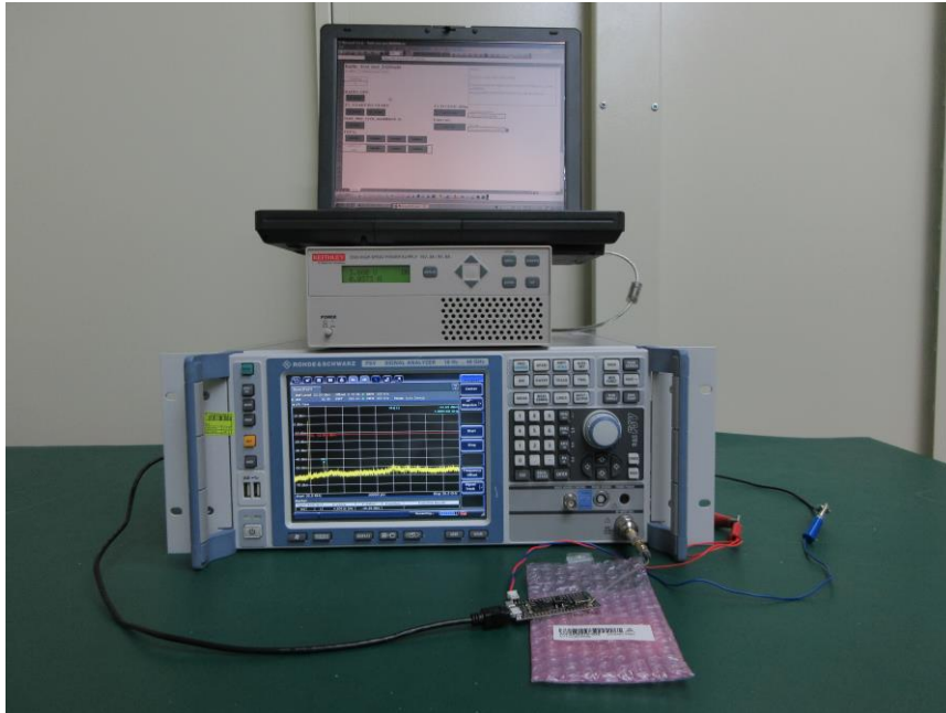
Photograph 7: Set-up for Conducted Test
