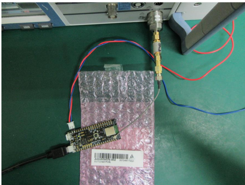
Photograph 8: Set-up for Conducted Test
