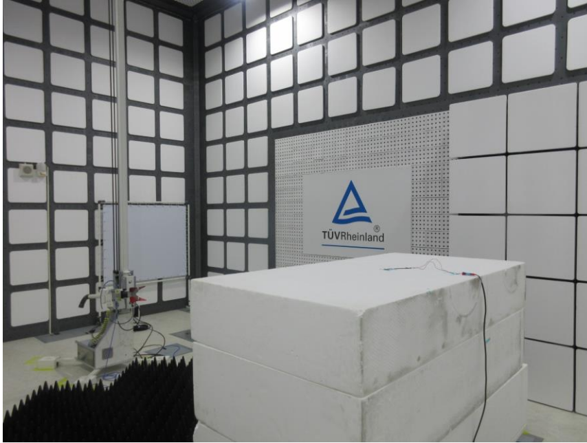
Photograph 5: Set-up for Spurious Emissions (Back View 3)
