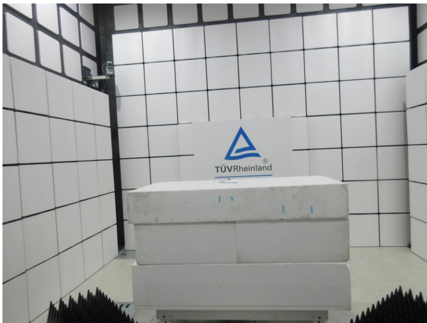
Photograph 2: Set-up for Spurious Emissions (Front View 2)
