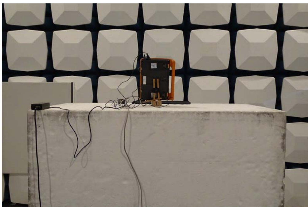
Back View of Radiated Test (Horn)
