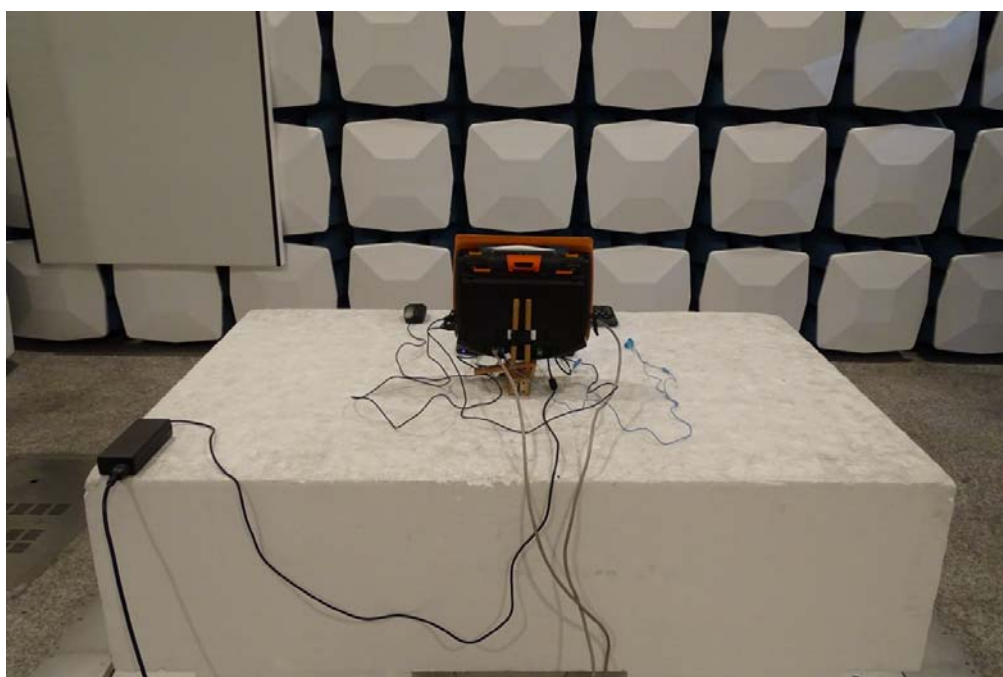
Back View of Radiated Test - Charger Mode
