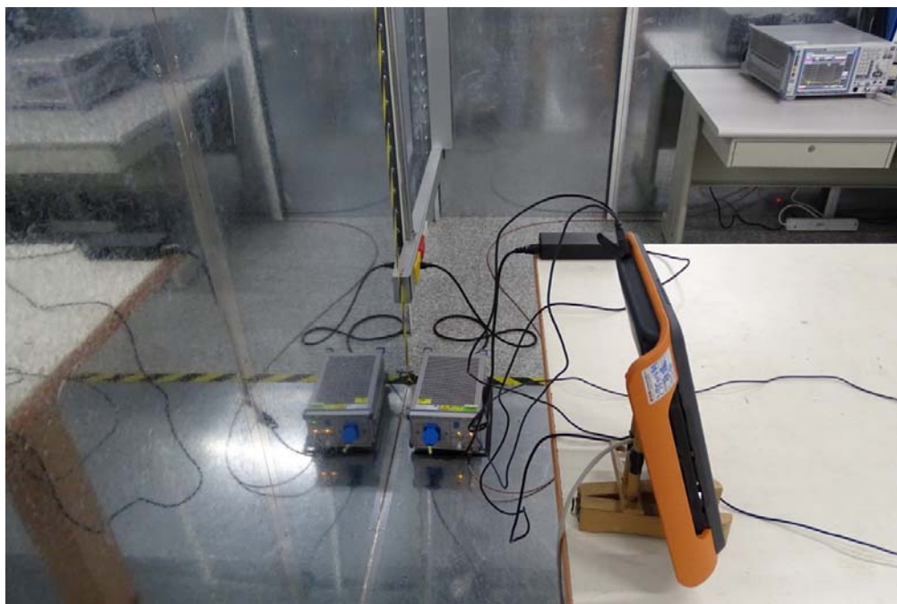
Back View of Conducted Test
