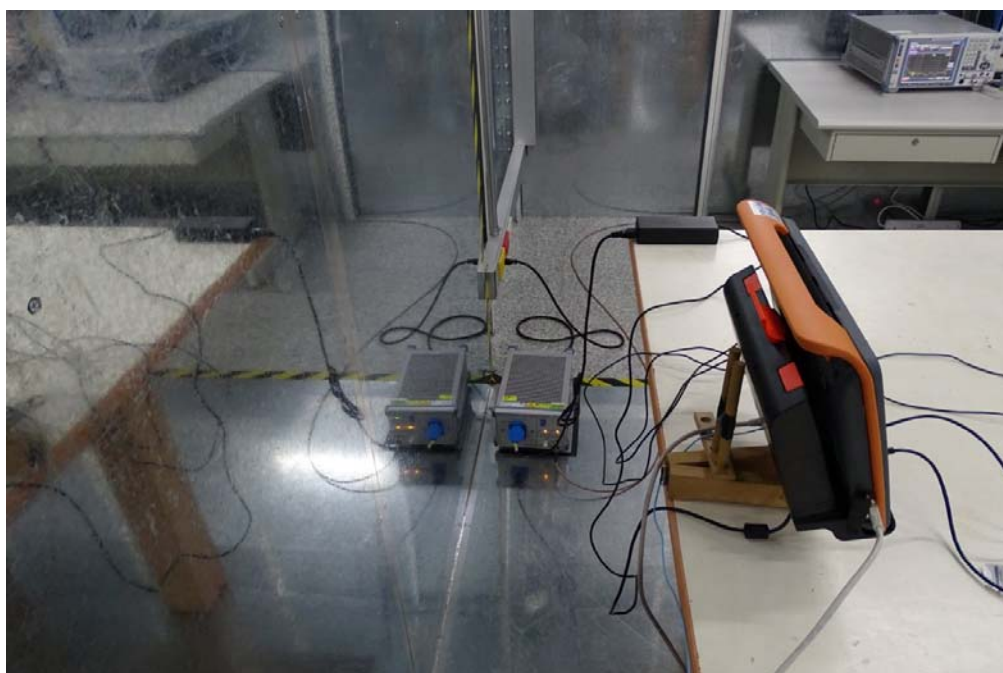
Back View of Conducted Test - Charger Mode
