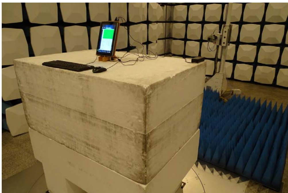
Front View of Radiated Test (Horn)
