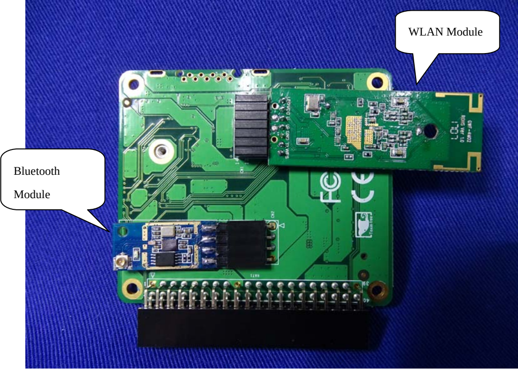
(11) EUT Photo
