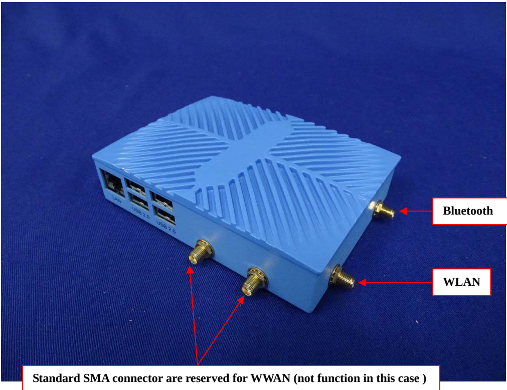
(1) EUT Photo
