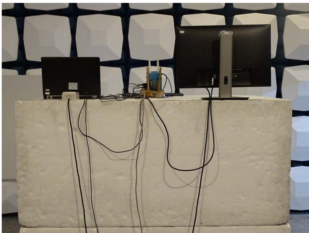
Back View of Radiated Test (Horn_18~40GHz)_ATM020-W050U
