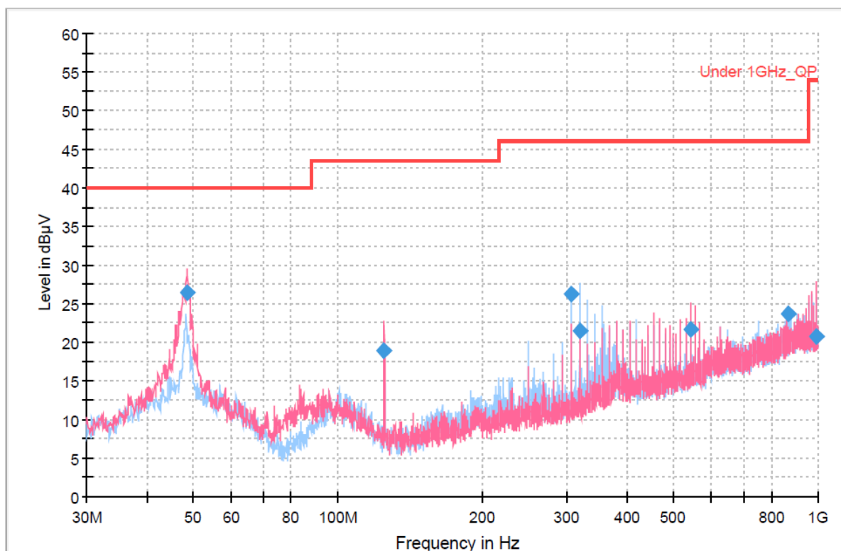
Worst case – RSE (Below 1 GHz)_TM 4 (NII 5)
