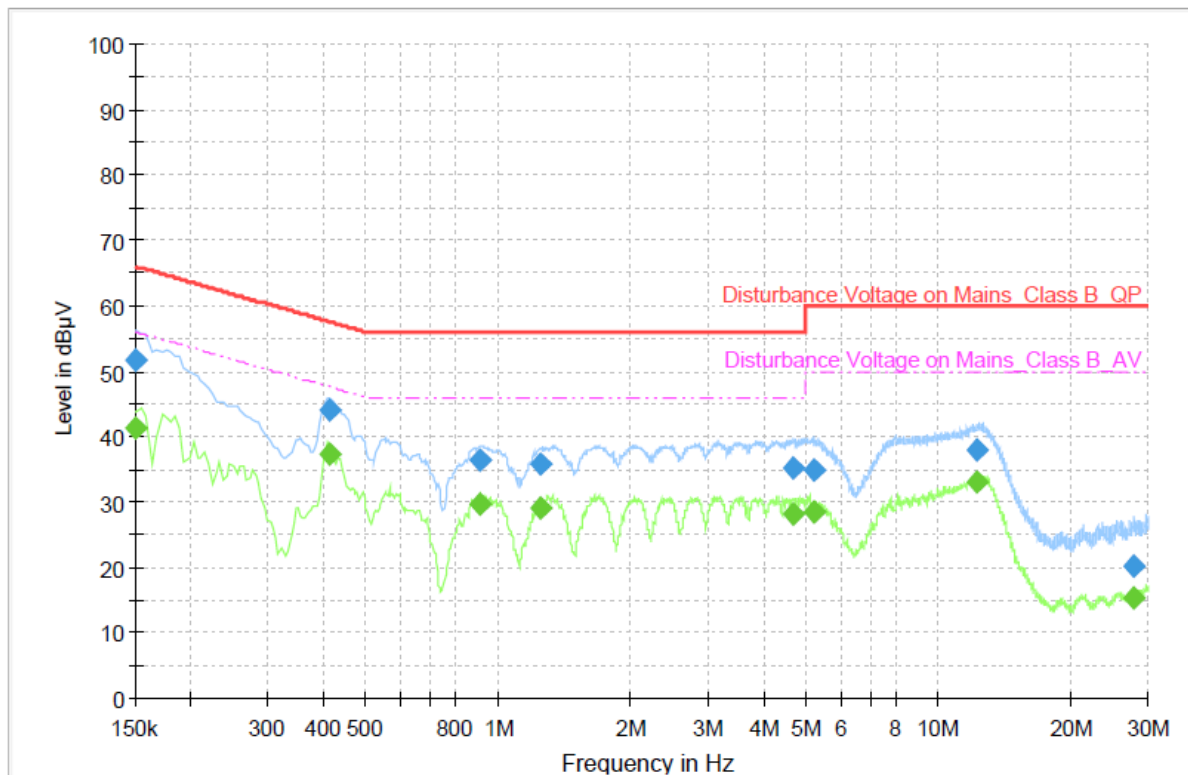
Worst case – AC Line (150 kHz ~ 30 MHz)_TM 1
