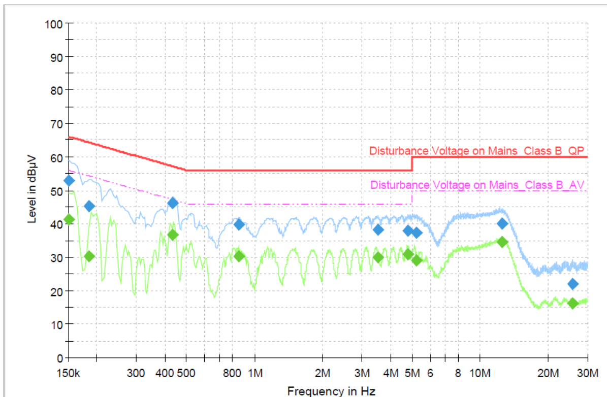
Worst case – AC Line (150 kHz ~ 30 MHz)_TM 2 (NII 1)
