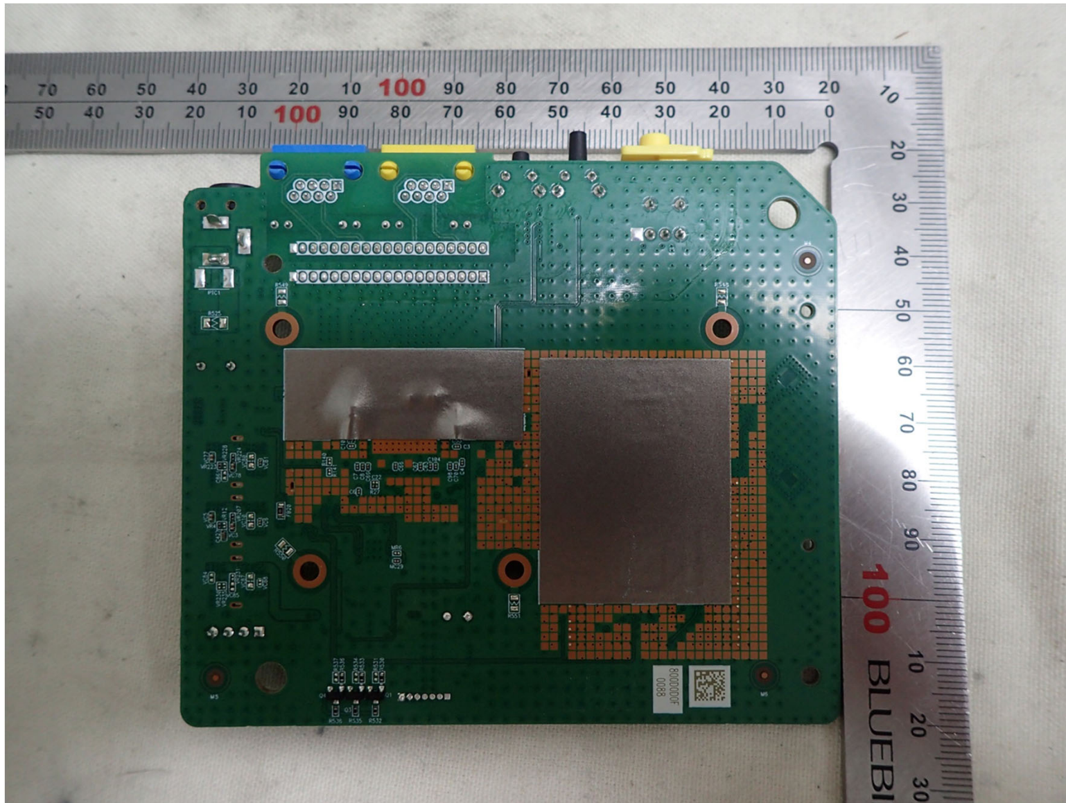
MAIN BOARD BOTTOM
