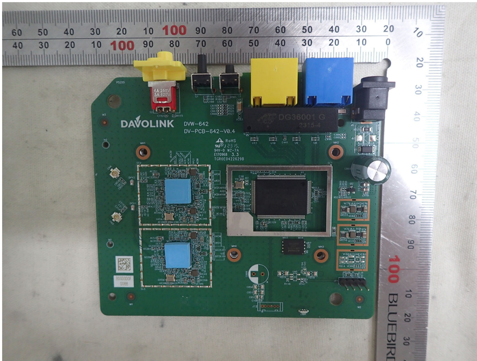
MAIN BOARD TOP
