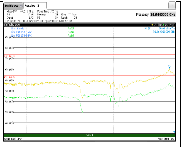
Polarity:Vertical
