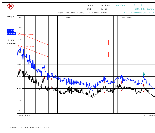
HOT LINE
