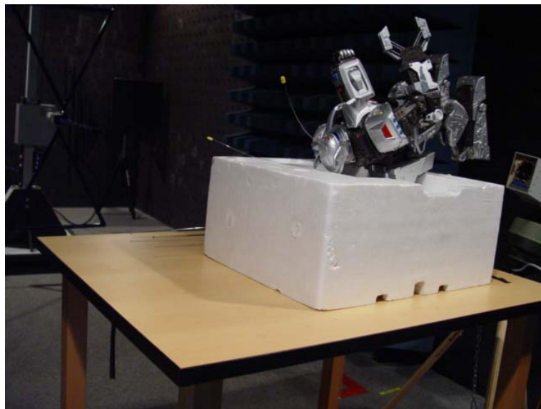
Set-up for radiated emission, operated
