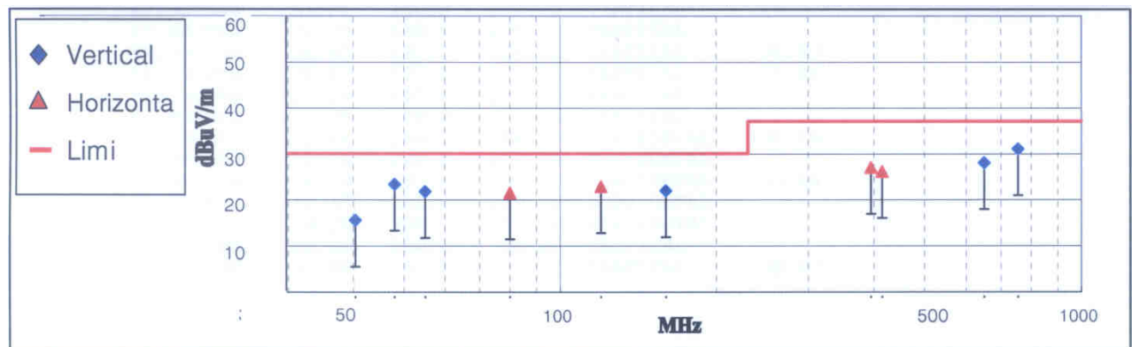
< Fig 4. Radiated emission result _ Stand by mode >
