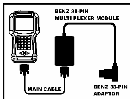
[Connecting MB 38-pin multiplexer to the head unit]
