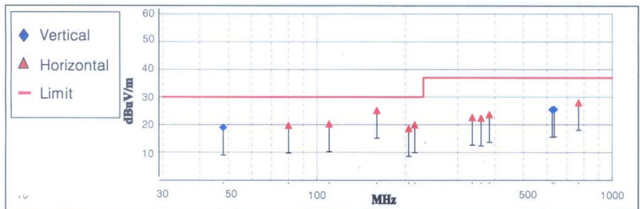
< Fig 4. Radiated emission result >
