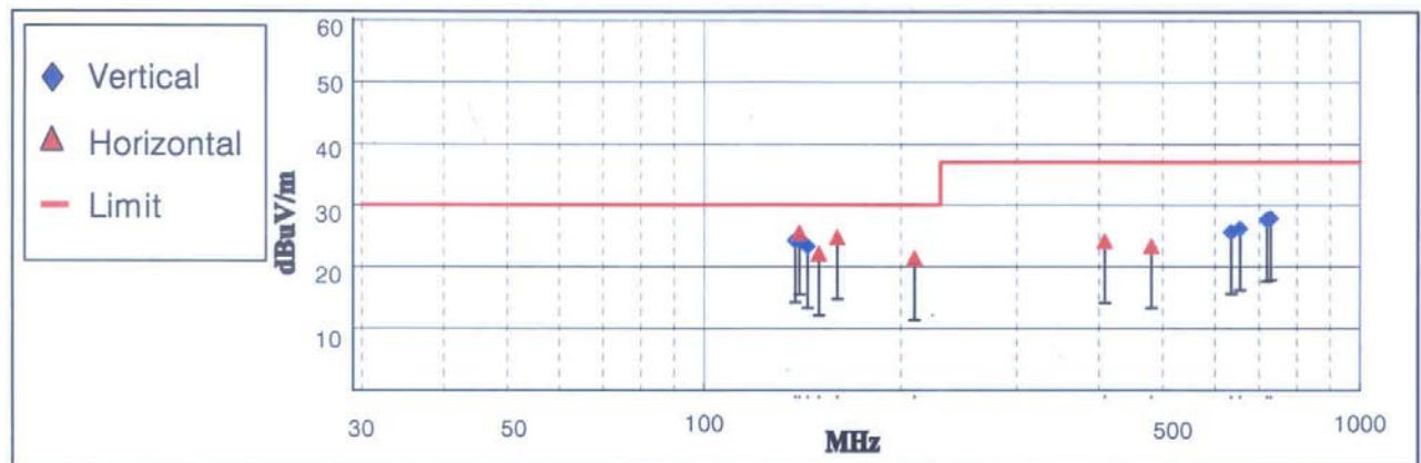
< Fig 5. Radiated emission result >
