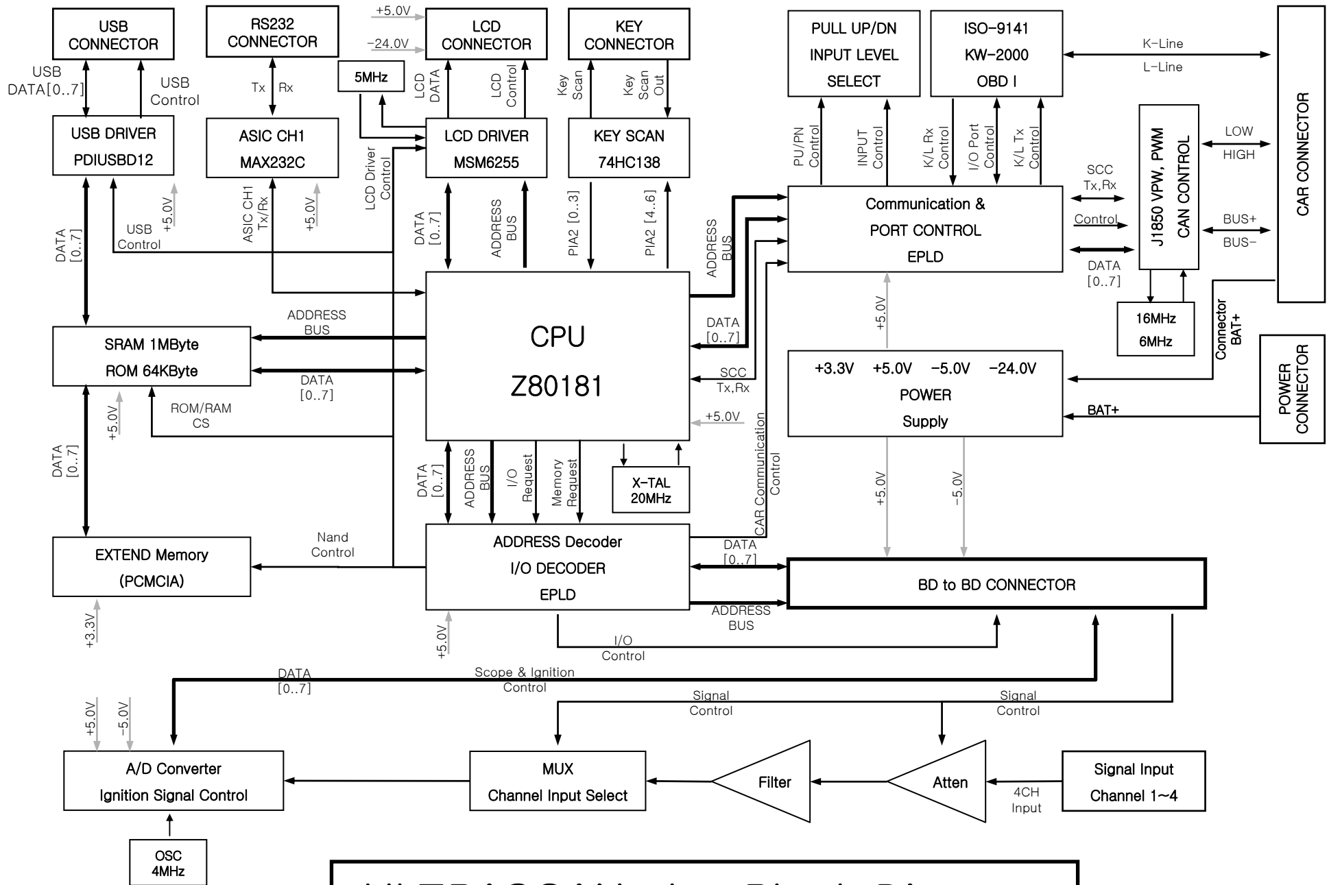
ULTRASCAN plus Block Diagram
