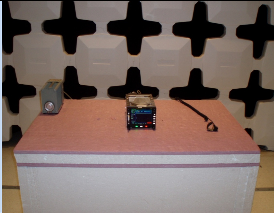
Test Set Up Photo 1
