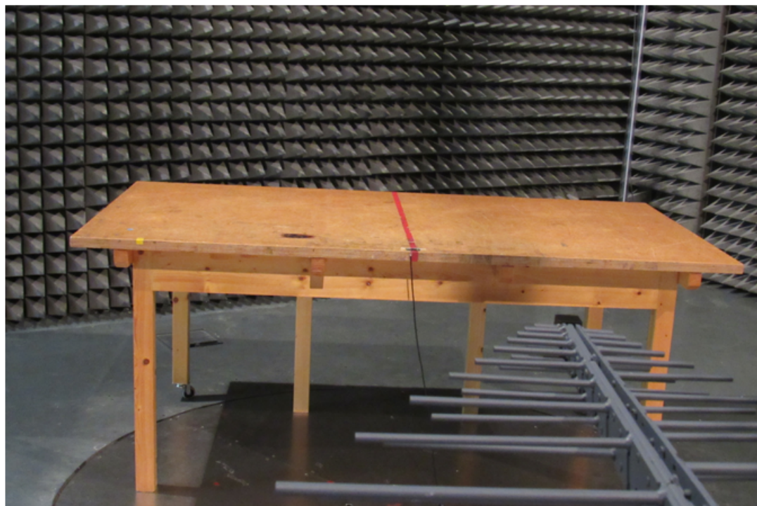
Setup radiated
