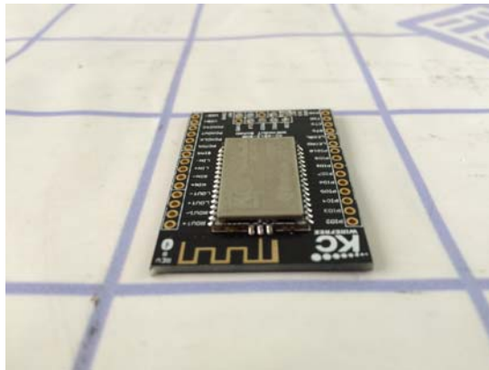
PCB Antenna type External view-6
