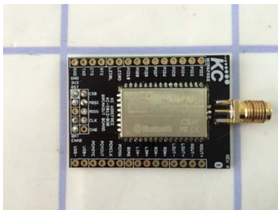
External Antenna type External view-1
