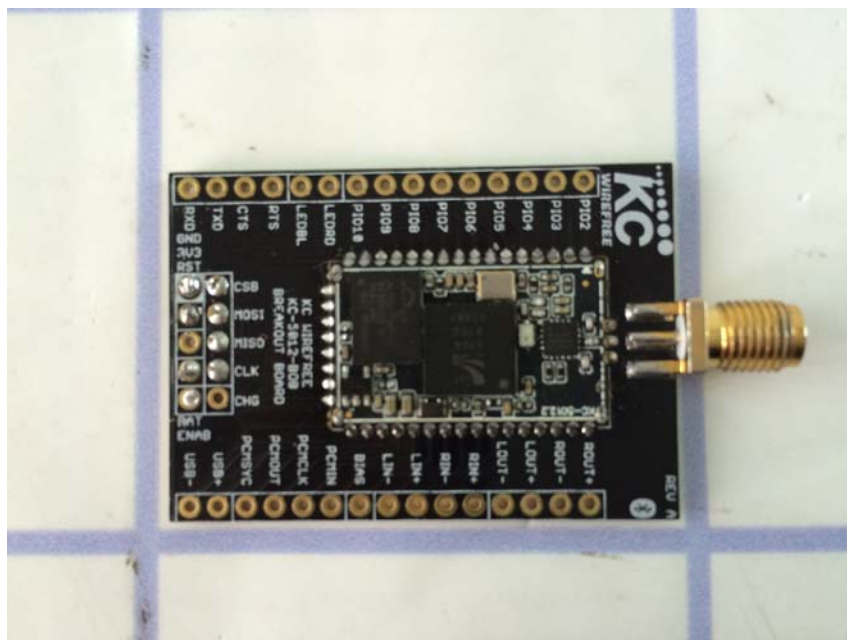
External Antenna type PCB side 1 view
