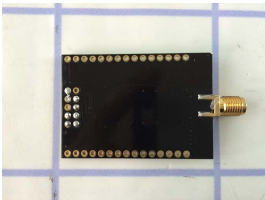
External Antenna type PCB side 2 view
