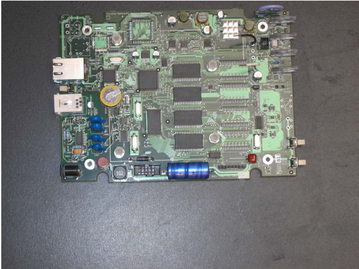
Digital Board top and bottom (no rf circuitry on this board)
