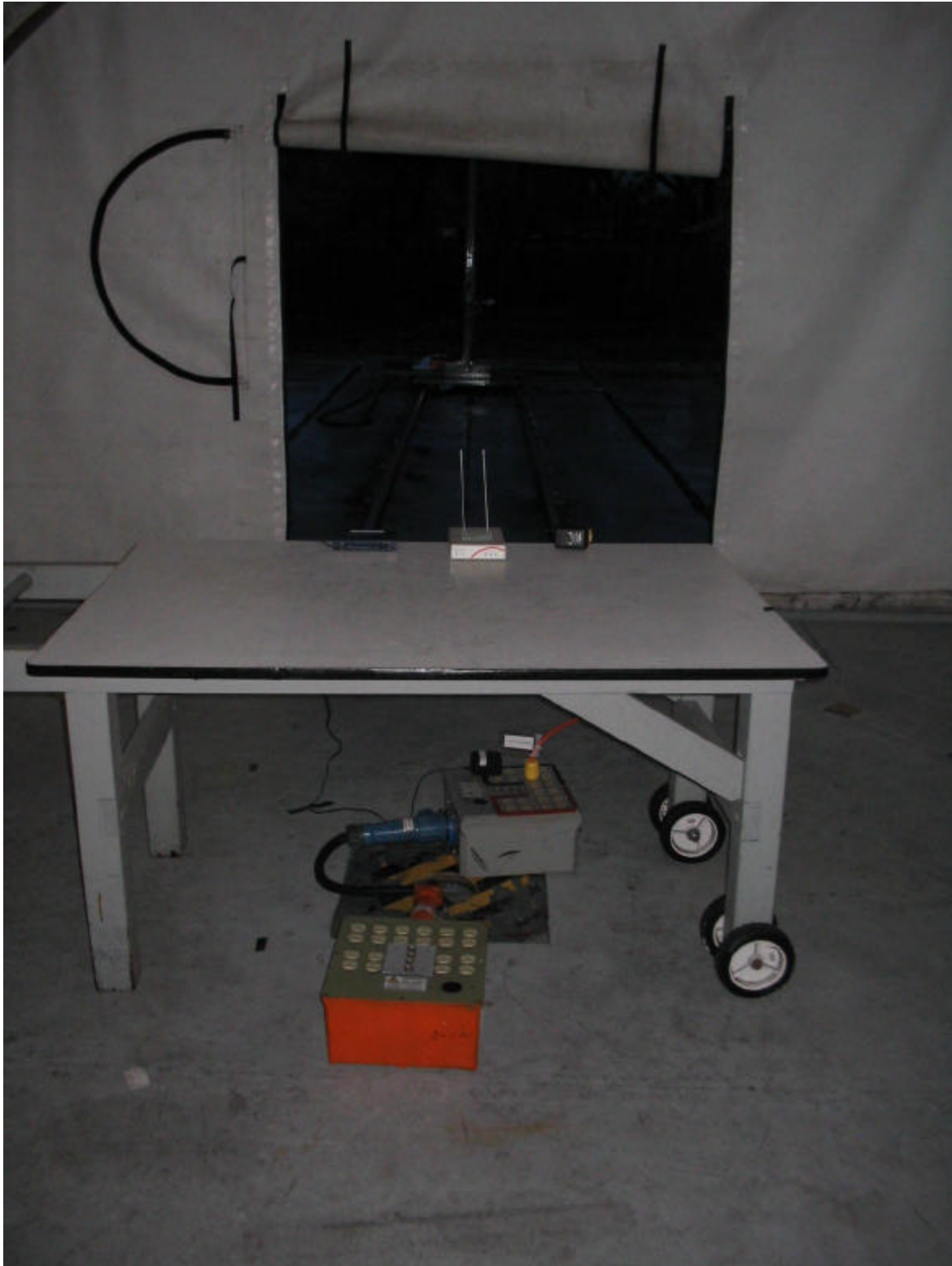
Figure 2: Radiated Emissions - Front View
