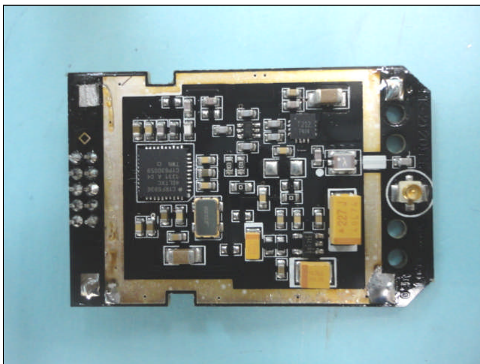
2.4G Transceiver Module
