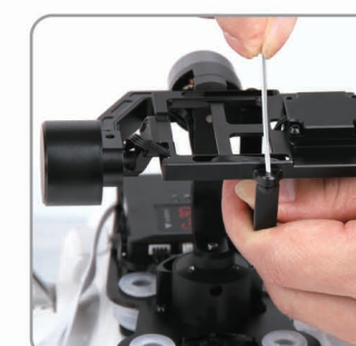
5.2 Unscrew 2 M2x4 screw, Loosen the camera fixed frame.
