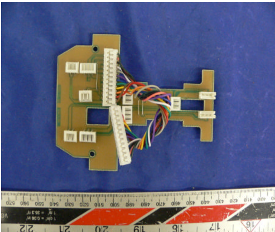
Interface Board Top View
